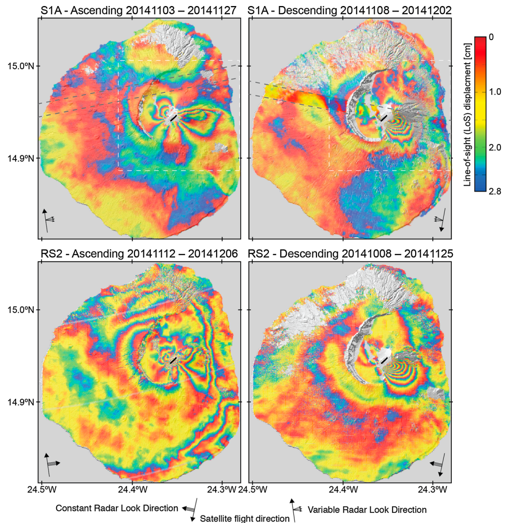
Figure 2. Interferograms of Fogo Island for the onset of the 2014–2015 Pico do Fogo eruption. (top left) Ascending co-ruptive Sentinel-1A interferogram spanning 3 November 2014 to 27 November 2014; (top right) Descending co-ruptive Sentinel-1A interferogram spanning 8 November 2014 to 2 December 2014; (bottom left) Ascending co-ruptive RADARSAT-2 interferogram spanning 12 November 2014 to 6 December 2014; and (bottom right) Descending co-ruptive RADARSAT-2 interferogram spanning 8 October 2014 to 25 November 2014.
