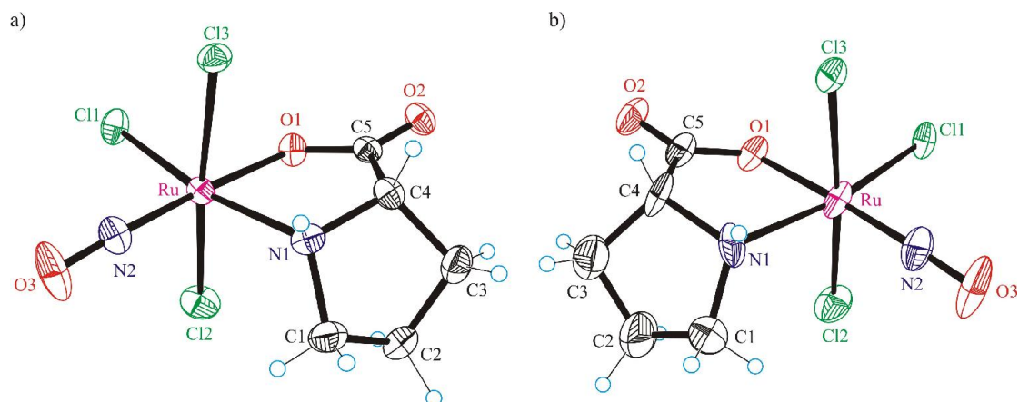
Figure 2. ORTEP drawings of the complex anion [RuCl 3 (L-Pro-H)(NO)] - in 4 (a), and [RuCl 3 (D-Pro-H)(NO)] - in 5 (b) with atom labeling. The thermal ellipsoids are shown at 50% probability level.
