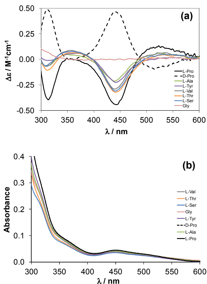
Figure 4. CD (a) and UV–vis (b) spectra of the studied ( n Bu 4 N)[RuCl 3 (AA–H)(NO)] complexes at pH 7.40 [ c_{complex} = 50 \mu M; 0.02 M phosphate buffer; 0.1 M KCl; T = 298 K].
