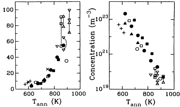
FIG. 33. Radii and concentrations of He bubbles in Al for different experimental conditions. The values correspond to bubbles annealed at T_{ann} after the introduction of He at lower temperatures. The solid symbols denote values from positron lifetime analysis, and the open symbols correspond to transmission electron microscope data (from Jensen, Eldrup, Singh, and Victoria, 1988).
