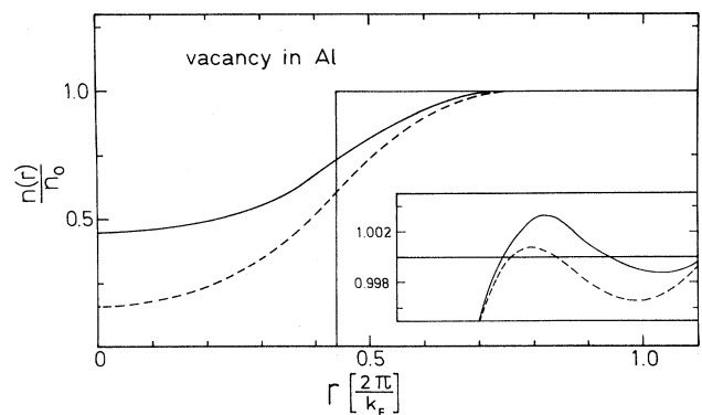
FIG. 28. Electron density at an Al vacancy in the jellium model. The results of the two-component density-functional theory in the presence of a trapped positron (solid curve) and without a positron (dashed curve) are shown (from Boroński and Nieminen, 1986).
