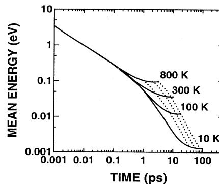
FIG. 9. Positron mean energy \bar{E} as a function of time after implantation in Al at different temperatures. The dotted lines connect points corresponding to \bar{E} = 1.1E_{\text{th}} , \bar{E} = 1.01E_{\text{th}} , and \bar{E} = 1.001E_{\text{th}} , where E_{\text{th}} is the thermal energy \frac{3}{2}k_B T (from Jensen and Walker, 1990).
