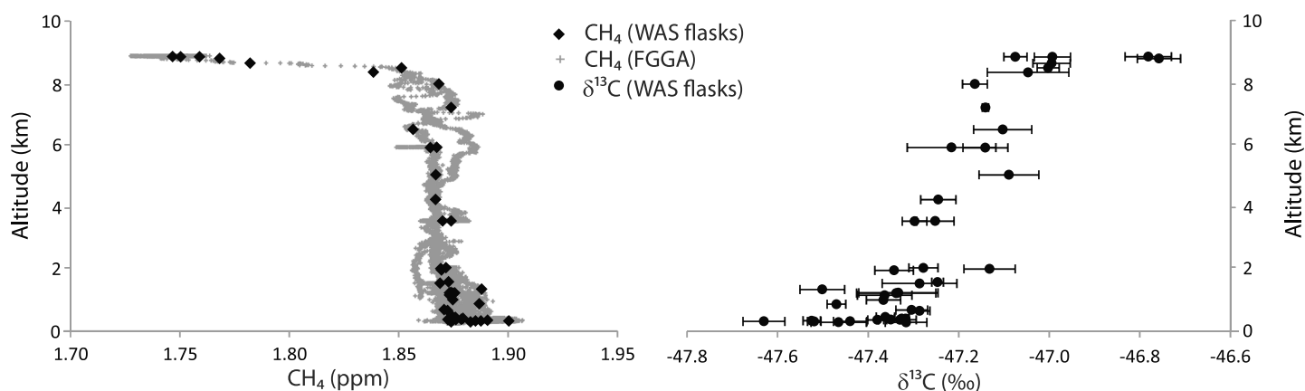
Figure 6. Variation in methane mole fraction (measured using the FGGA on board the aircraft and in WAS flasks) and \delta^{13}\text{C} (measured in WAS flasks) on flight B720 on 22 July 2012.
