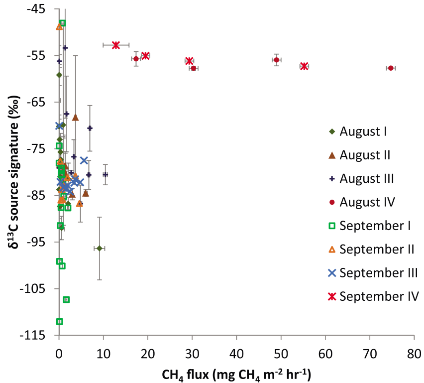
Figure 3. Calculated \delta^{13}\text{C} source signatures and fluxes for 41 chambers at Stordalen Mire in August 2013 and September 2013. Different colored symbols correspond to the four classes of chambers. Source signatures are only plotted if there was a >0.05 ppm increase in mole fraction in the chamber. The x error bars show the standard errors for flux measurements made on 18 August and 22 September. Some error bars are smaller than the symbol size. The y error bars for August show the standard error in two source signature calculation measurements for each chamber carried out on 18 and 19 August. The September isotope sampling was carried out on 21 September and was not repeated so error bars are not shown.
