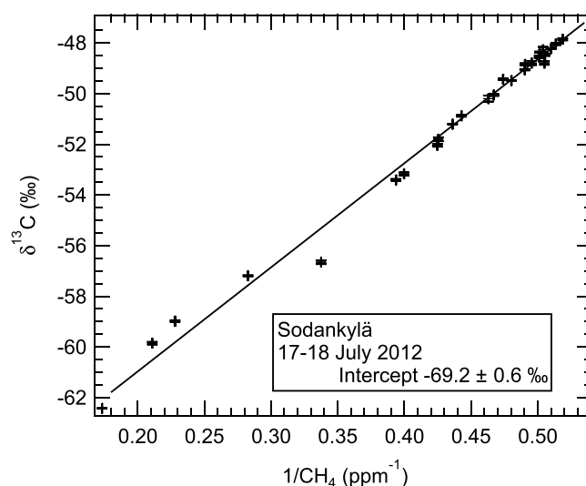
Figure 5. Keeling plot for air samples collected at 0.3 and 3 m above ground level in the Sodankylä fen, 17–18 July 2012.
