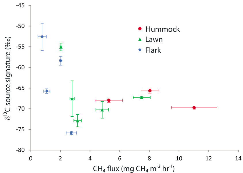
Figure 2. Calculated \delta^{13}\text{C} source signature and \text{CH}_4 flux measured in 12 chambers at Sodankylä. Chambers were categorized according to wetness: hummocks (red), lawns (green), and flarks (blue). The y axis error bars denote the standard error in calculated signature from two or three samples collected from each chamber on different days, between 20 and 26 July 2012. The x axis error bars denote the standard error in flux measurements carried out on 4 or 5 days between 20 and 26 July 2012.
