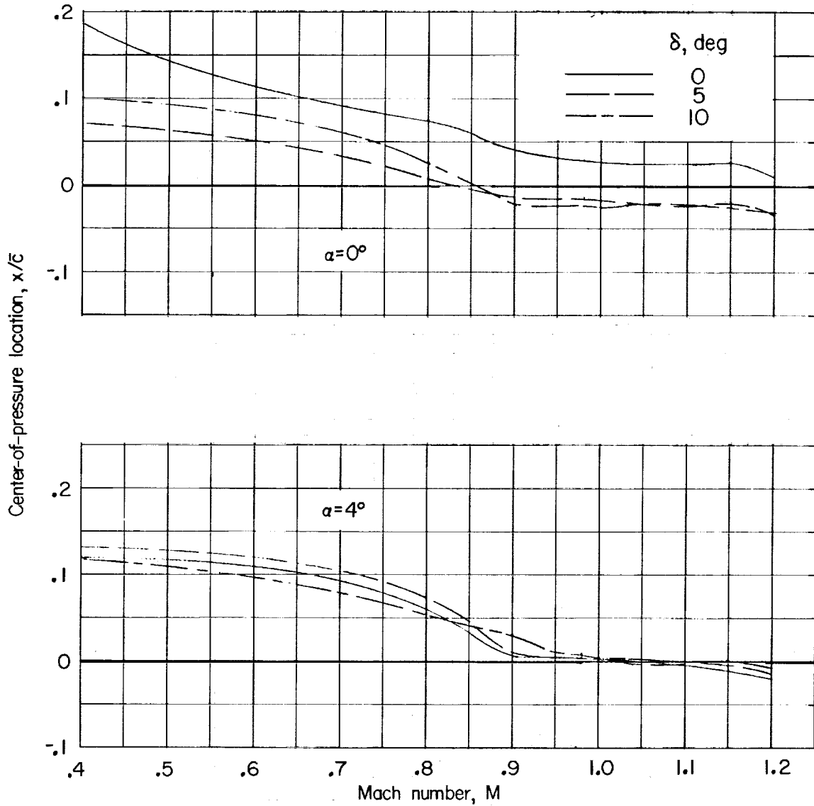
(e) Control surface 5.
