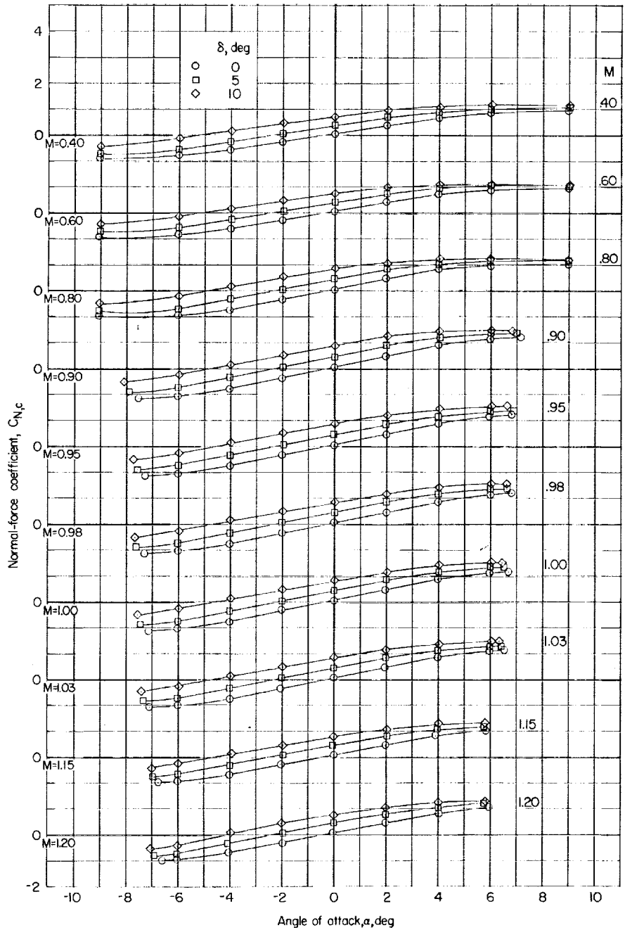
(e) Control surface 5. Figure 15.- Continued.
