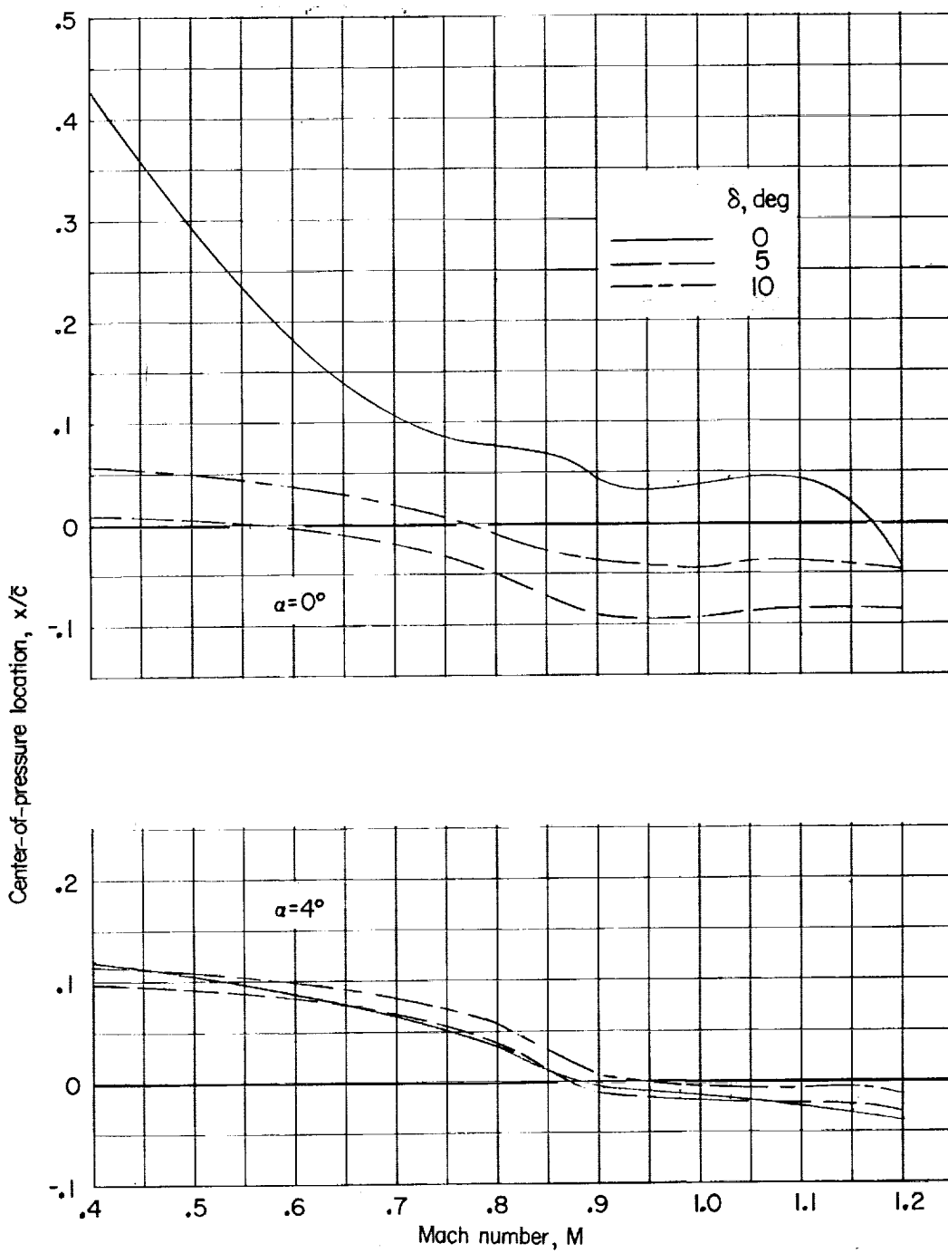
(f) Control surface 6.
