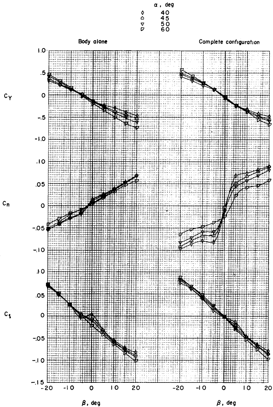
(c) \alpha = 40^\circ to \alpha = 60^\circ .
