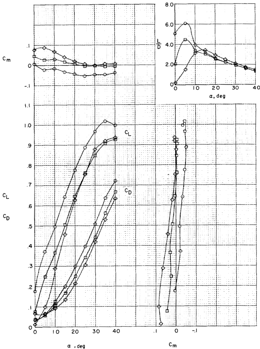
Figure 10.- Effect of horizontal-tail and trimmer-flap deflection on longitudinal aerodynamic characteristics of model with 6-inch spanwise extension on horizontal tails and 1.9-inch chordwise extension on trimmer flaps; \beta = 0^\circ .
