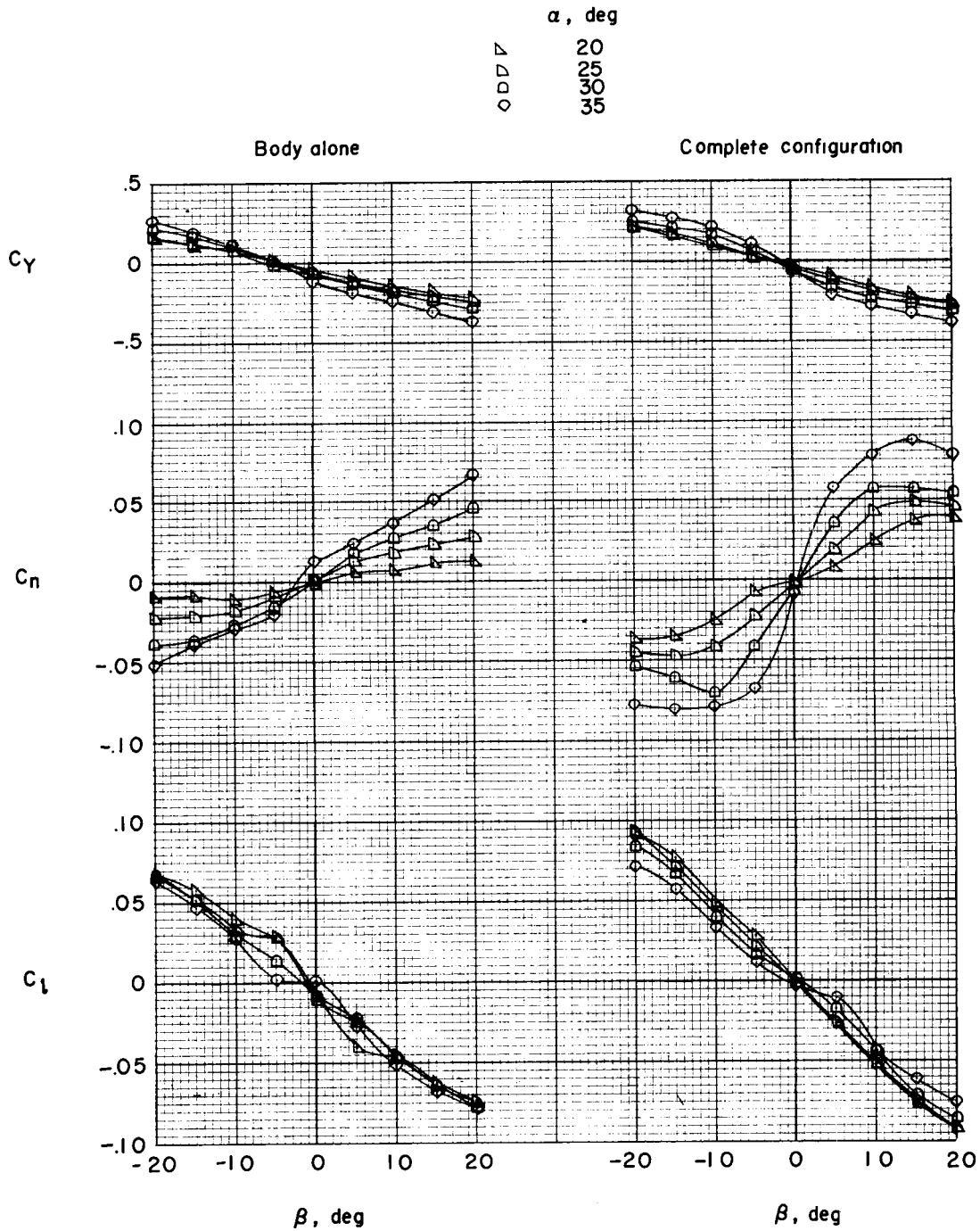
(b) \alpha = 20^\circ to \alpha = 35^\circ .
