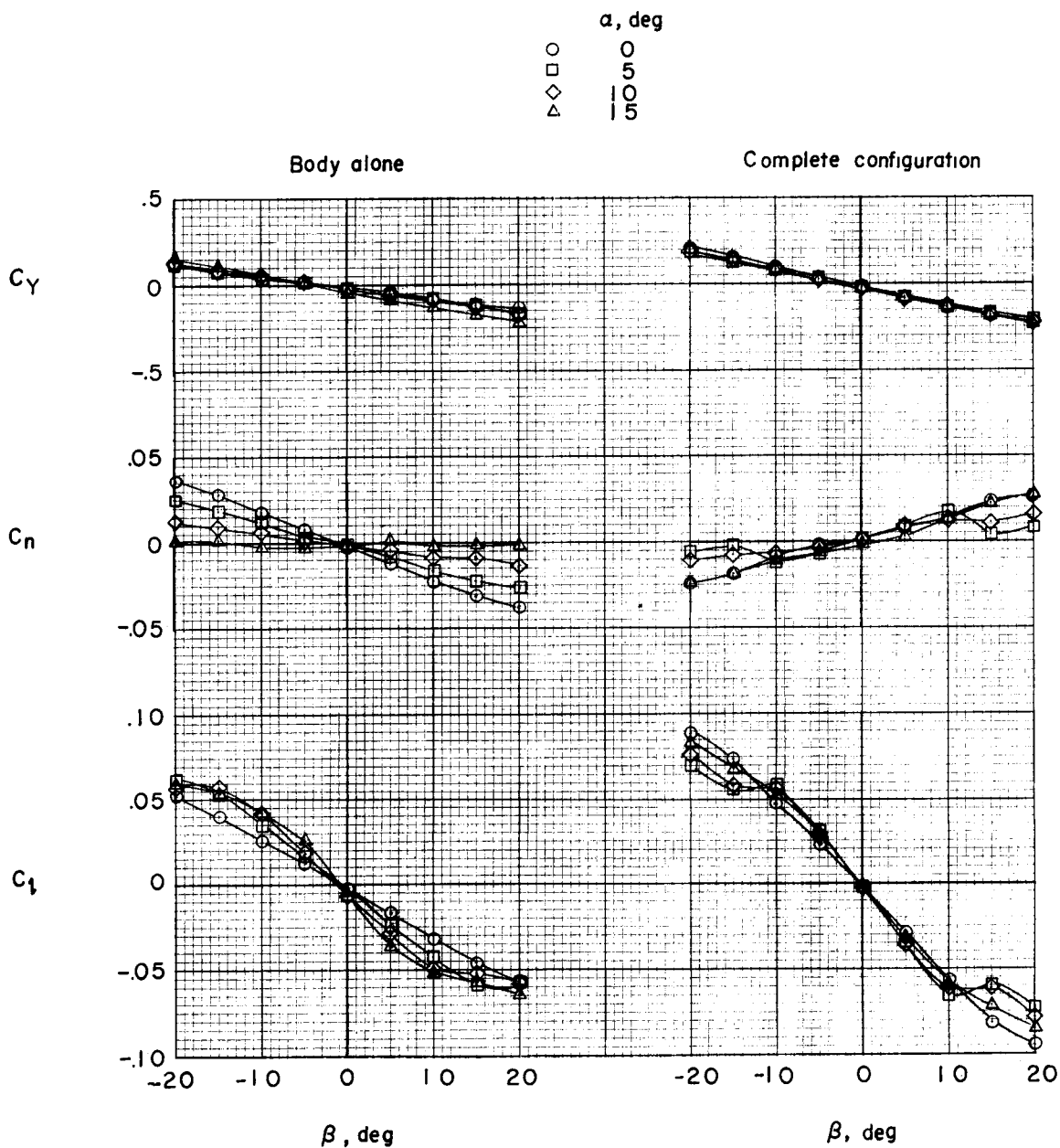
(a) \alpha = 0^\circ to \alpha = 15^\circ .
