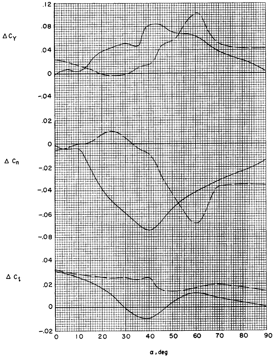
(b) Basic horizontal tails and trimmer flaps with 1.9-inch chordwise extension both deflected differentially.
