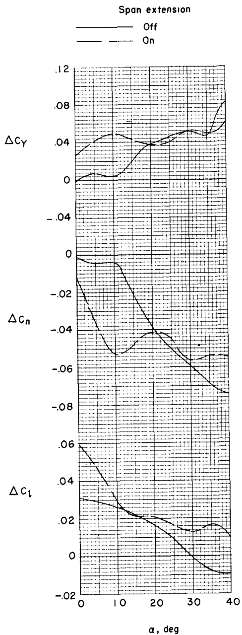
(c) Effect of 6-inch spanwise extensions on horizontal tails (trimmer flaps with 1.9-inch chordwise extensions and horizontal tails both deflected differentially); \delta_e = \delta_{fe} = 0^\circ .
