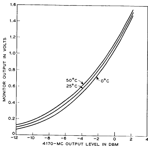
Fig. 14 — Voltage-power relations in the monitor.
