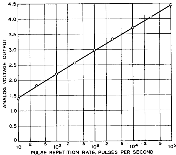
Fig. 25 — Ratemeter response.
