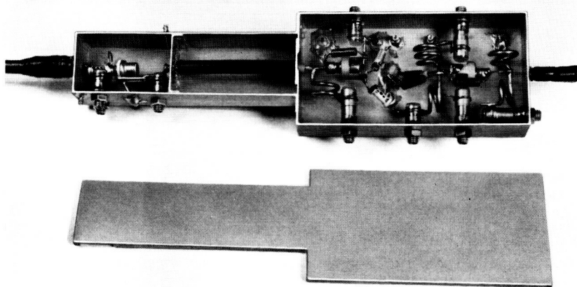
Fig. 20 — The varactor octupler.
