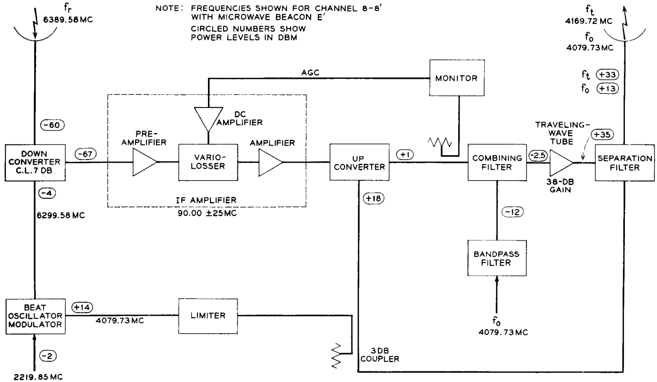
Fig. 4 — Telstar satellite amplifier simplified block diagram.
