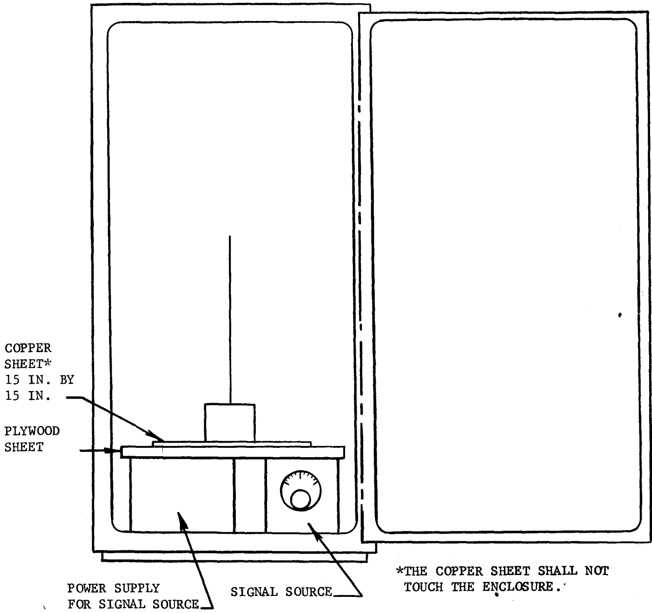
Figure 5. Signal source location.
