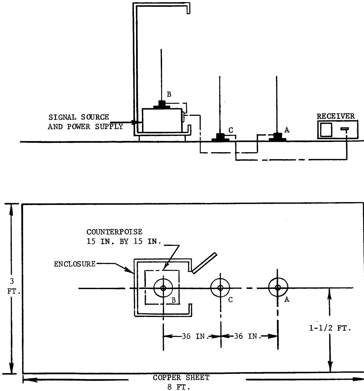
Figure 3. Test configuration for attenuation measurements of front of enclosure.
