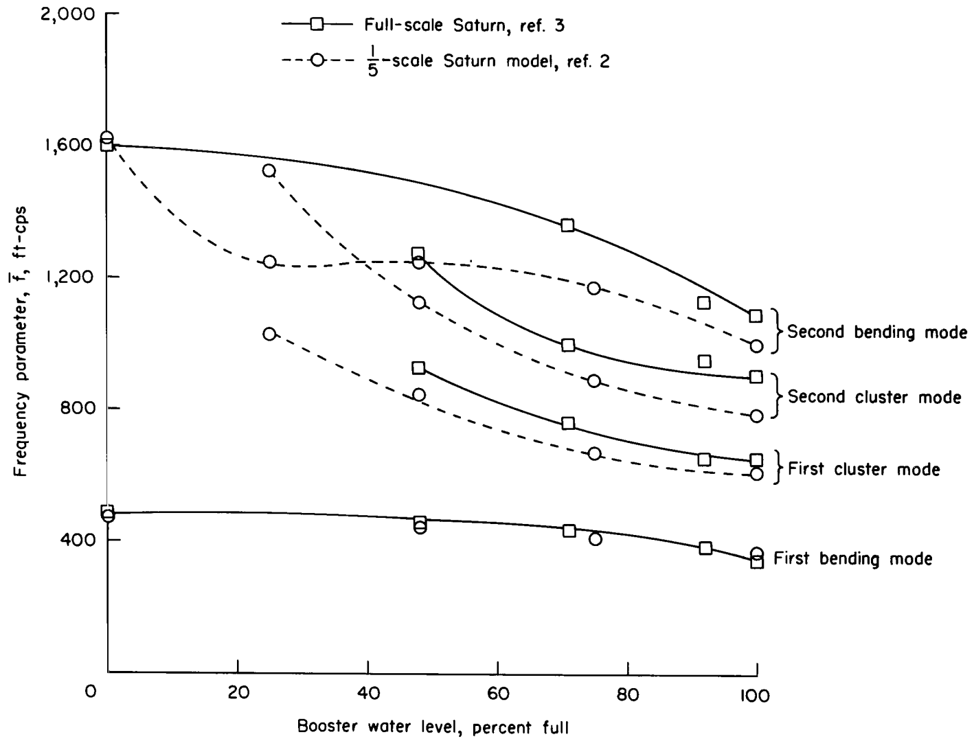
Figure 17.- Variation of frequency parameter of first four principal modes of Saturn with booster water level.
