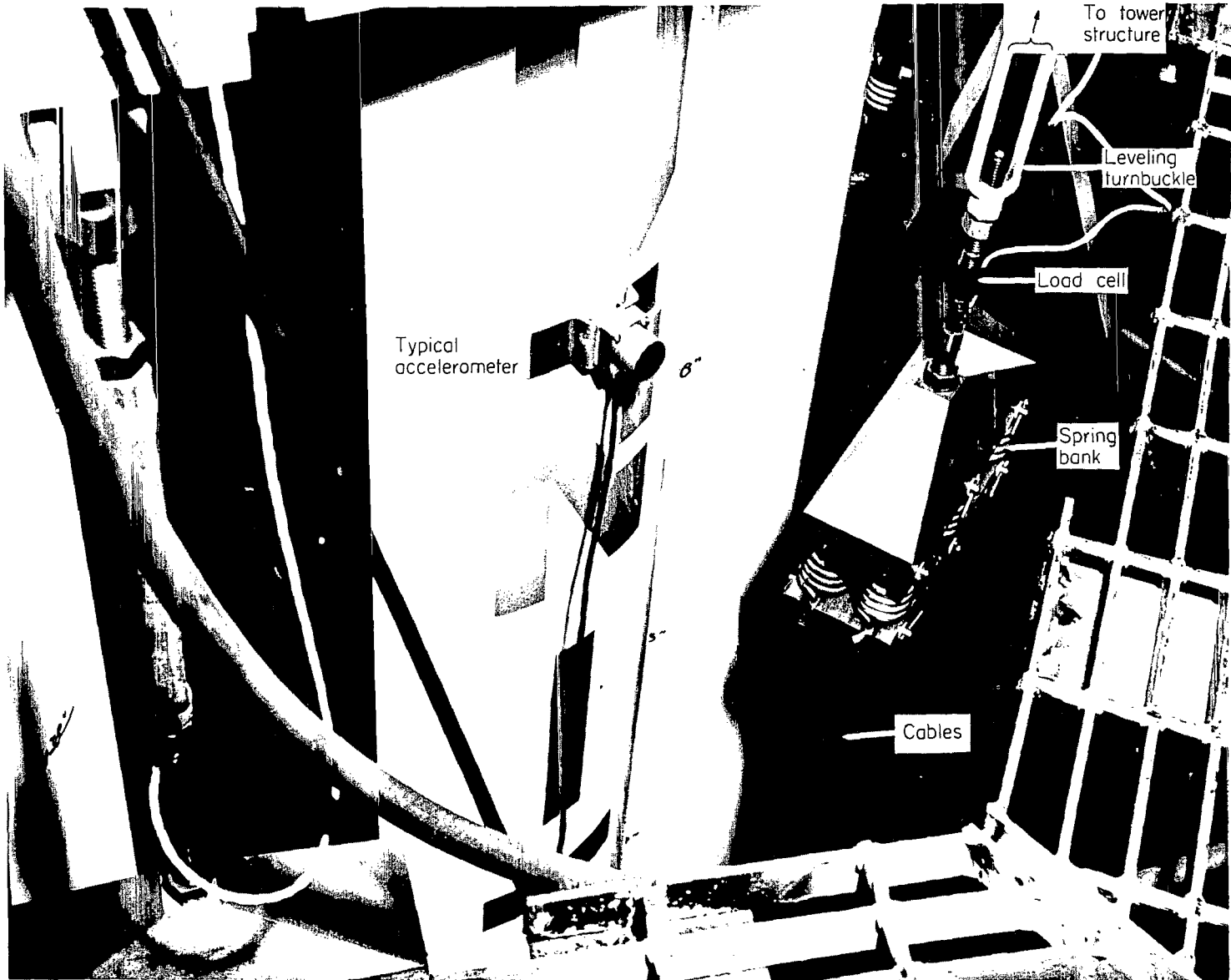
Figure 16.- Spring bank area of 1/5-scale Saturn model.
