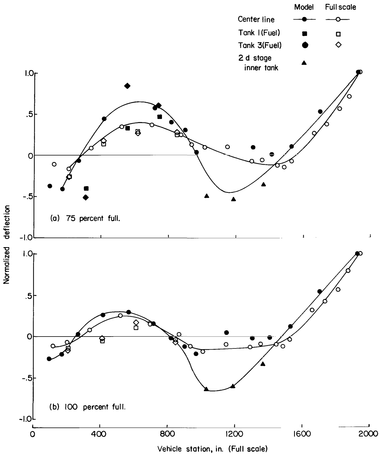
Figure 23.- Comparison of model with full-scale second bending modes.
