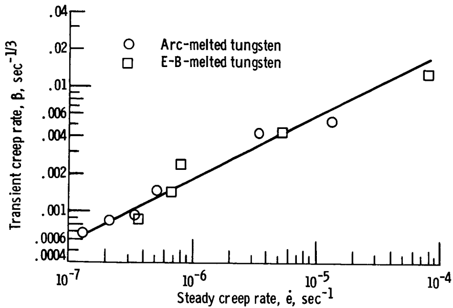
Fig. 9. - Relation between transient and steady creep rates for tungsten at 2875 o to 3500 o F.
