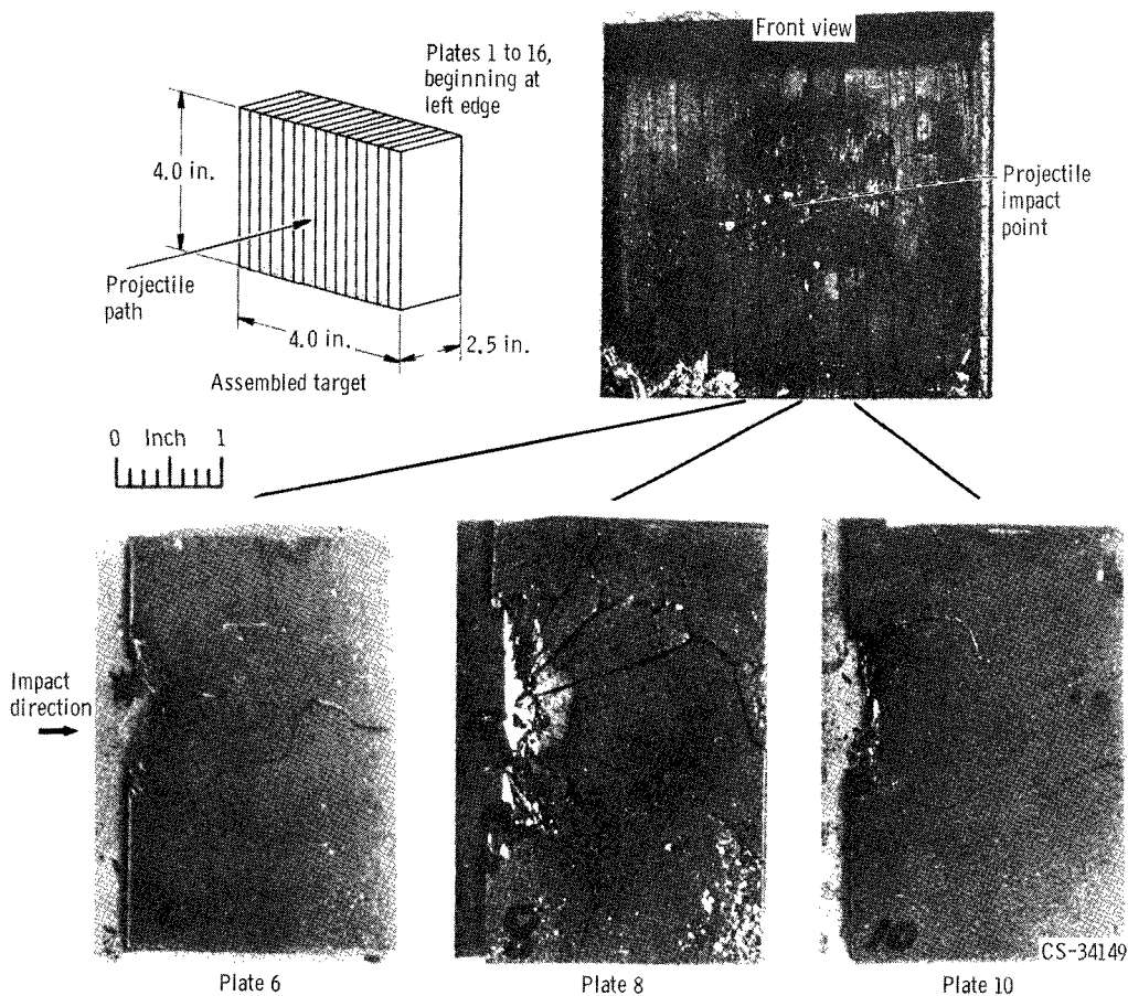
Figure 15. - Pyrolytic graphite semi-infinite block target (target 16) with individual plates oriented parallel to impact direction. Impact velocity, 25 600 feet per second with 1/8-inch-diameter pyrex sphere; target temperature, 1300° F.
