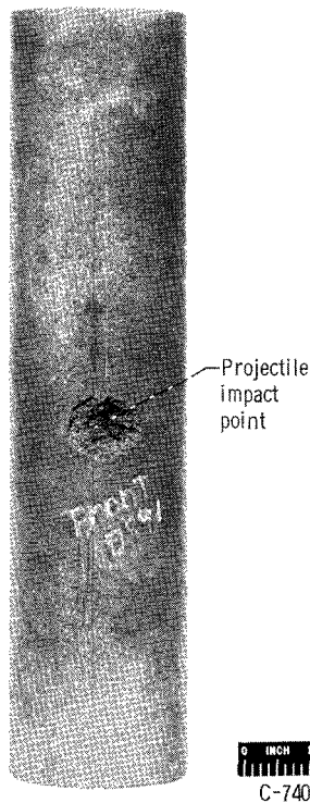
Figure 16. - AGSR graphite tube target (target 17, 2.50-in. o.d. by 0.50-in. i.d. by 12.0-in. length). Impact velocity, 24 600 feet per second with 3/32-inch-diameter pyrex sphere; target temperature, 1300° F.
