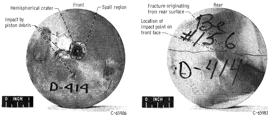
Figure 7. - Impact into a 4.0-inch-outside-diameter by 1.0-inch-thick hot-pressed beryllium disk (target 4) at 1300 o F. Impact velocity, 25 800 feet per second with 3/32-inch-diameter pyrex sphere.
