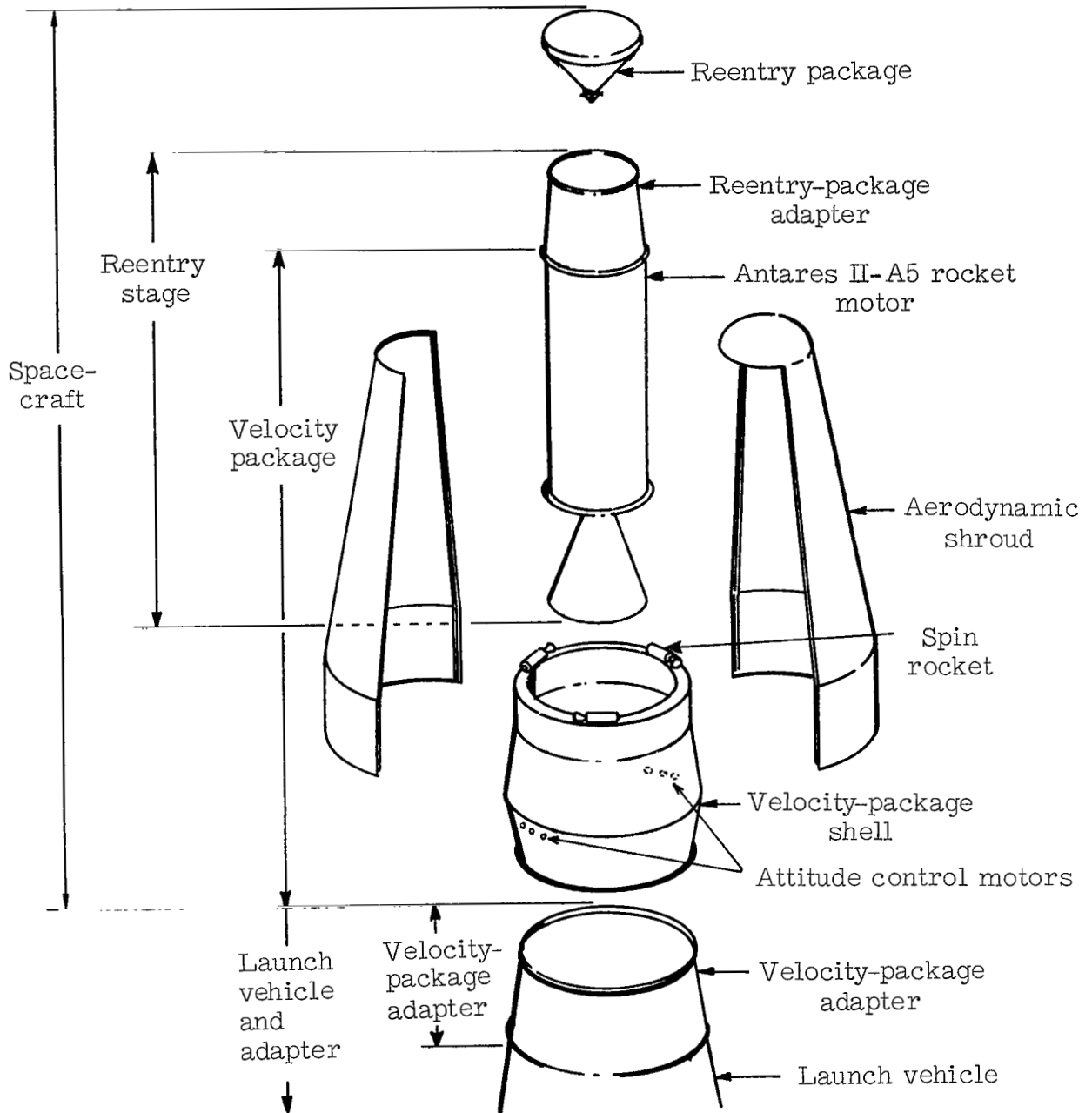
(b) Exploded view of spacecraft.
