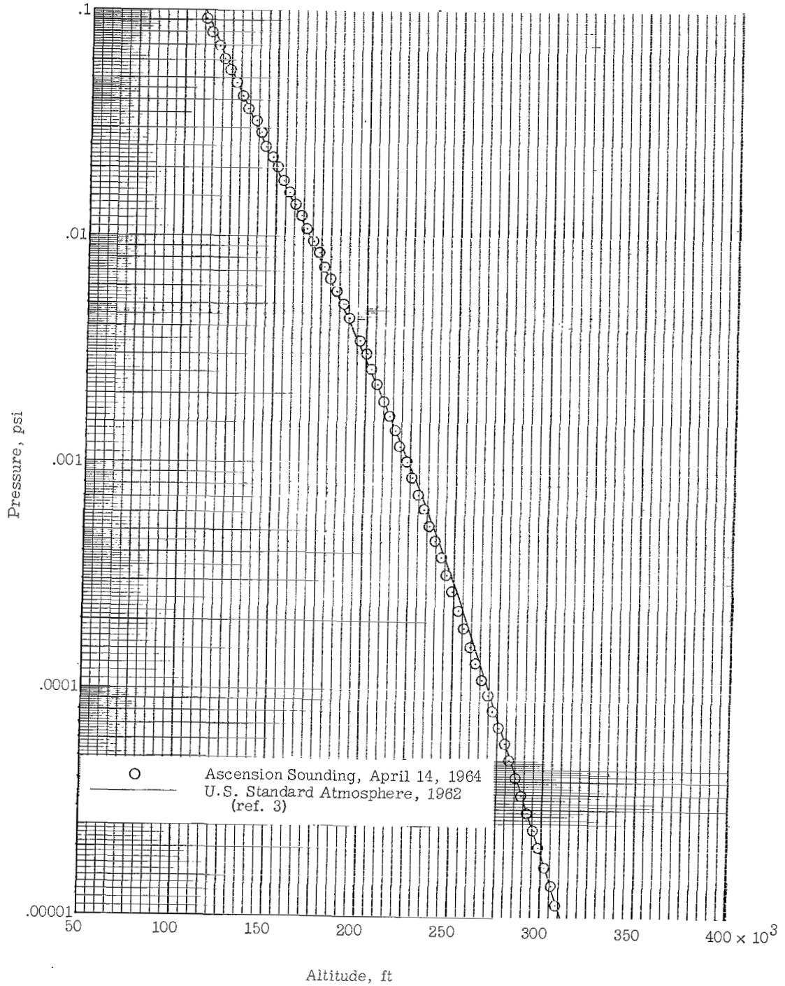
(a) Variation of pressure with altitude. Sea-level pressure = 14.68055 psi.
