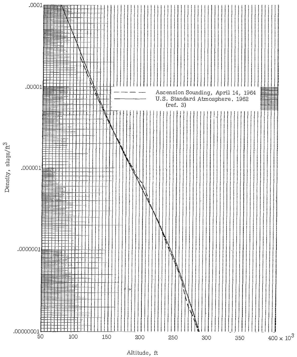
(b) Variation of density with altitude. Sea-level density = 0.00228 slug/ft 3 .
