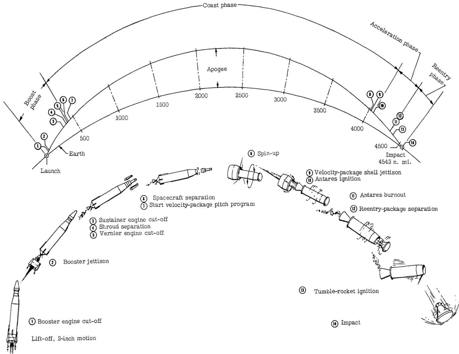
Figure 6.- Sequence of events in Project Fire flight 1.
