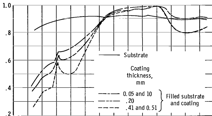
(a) Type A substrate.
