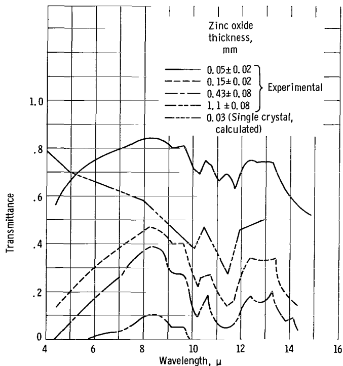
Figure 6. - Calculated transmittance of single crystal of zinc oxide and experimental transmittance of composites of zinc oxide and sodium chloride.
