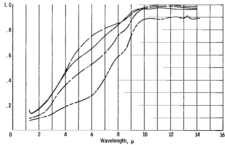
(c) Zinc oxide 0.4 millimeter above filled substrate.
