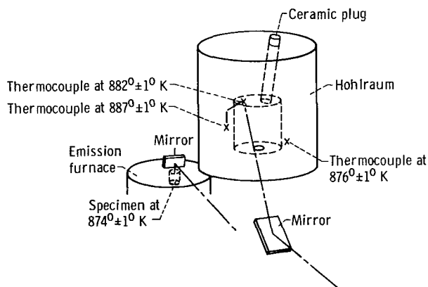
Figure 1. - Schematic drawing of hohlraum and emission furnace.
