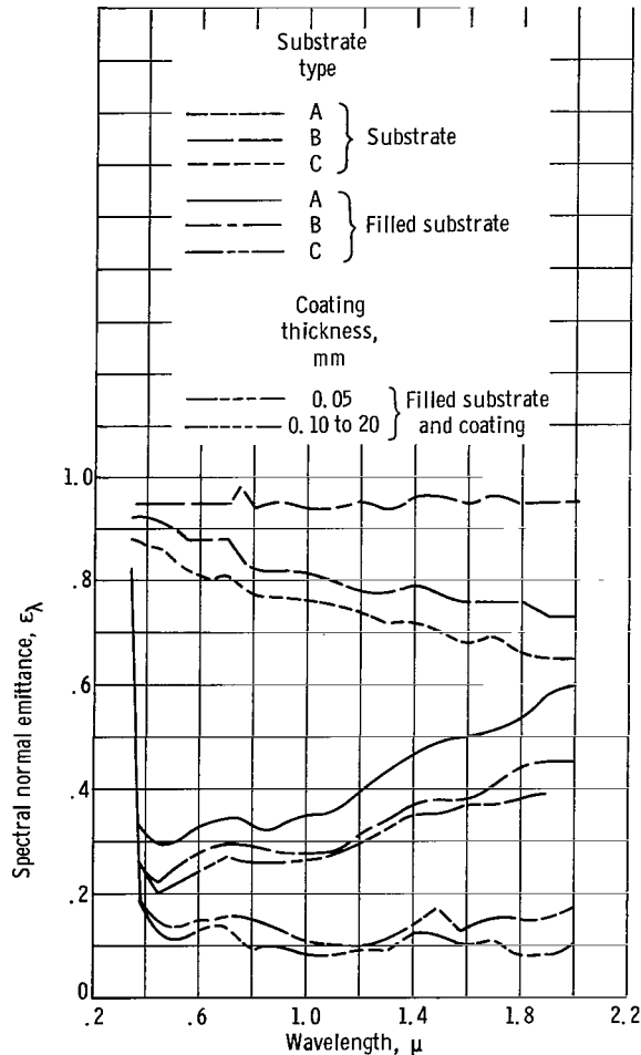
Figure 4. - Room-temperature spectral emittance of zinc oxide composites and substrates.
