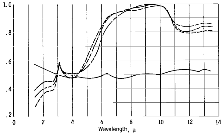
(c) Type C substrate.
