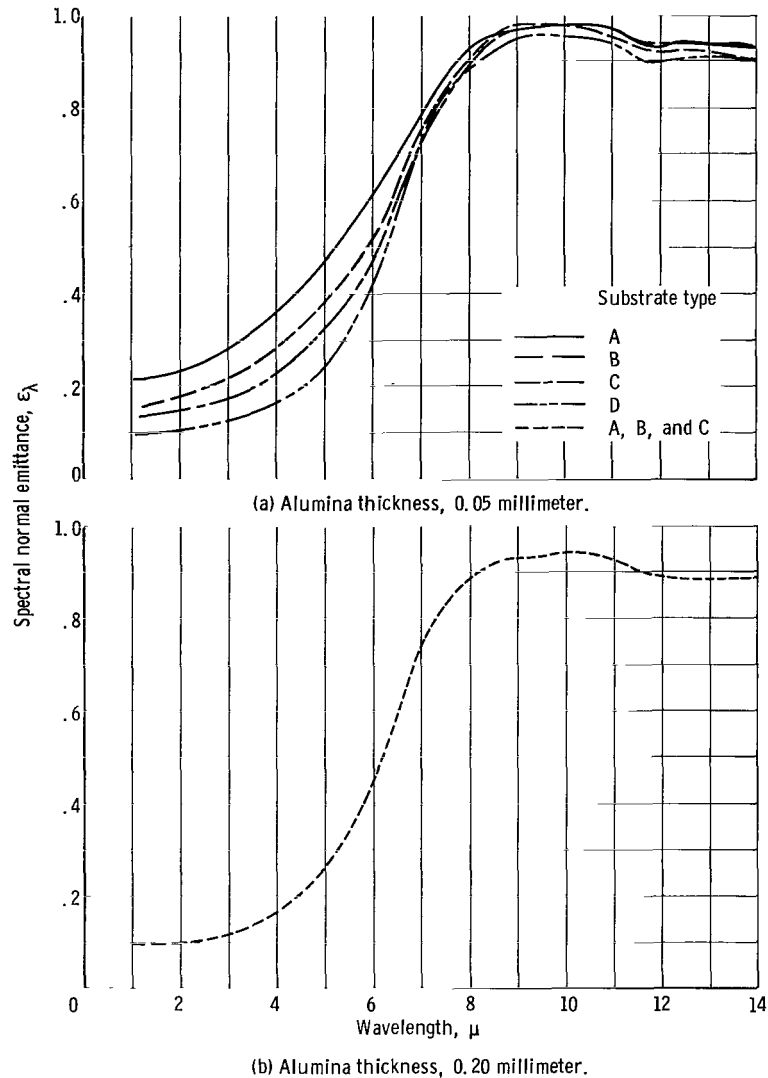
Figure 11. - Spectral composite emittance of powdered alumina above filled substrates.
