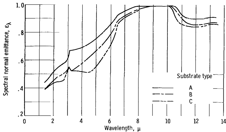
Figure 8. - Variation of spectral composite emittance of 0.05- and 0.10-millimeter, flame-sprayed alumina above filled substrate on three substrates. Surface temperature, 880^{\circ} \pm 8^{\circ} K.
