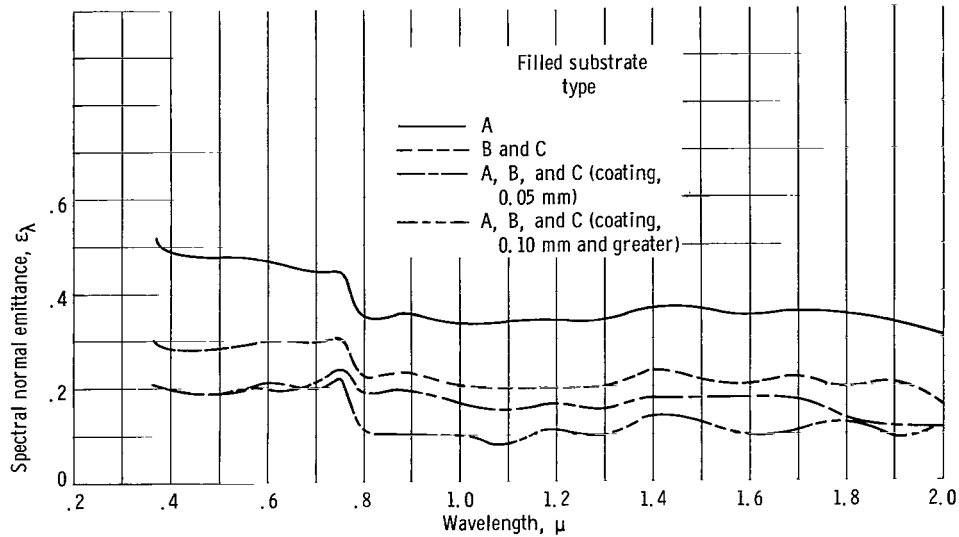
Figure 10. - Spectral emittance at room temperature of powdered alumina composites. (Substrate emittances are identical to those shown in fig. 4.)
