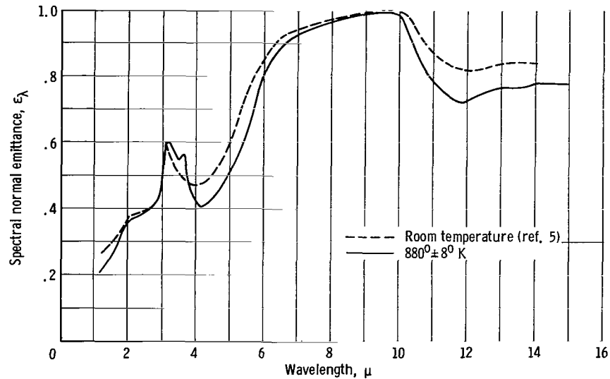
Figure 2. - Spectral emittance of flame-sprayed alumina.
