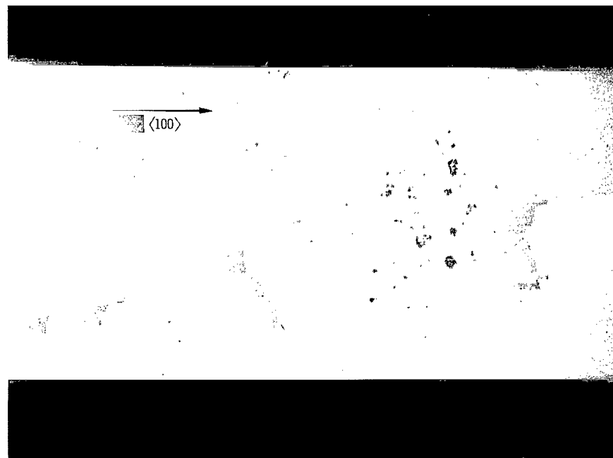
Figure 9. - Bright line traces on \{110\} flat of \{100\} oriented tungsten single crystal after 14 percent elongation. Etched with copper sulfate - ammonium hydroxide solution; X100.
