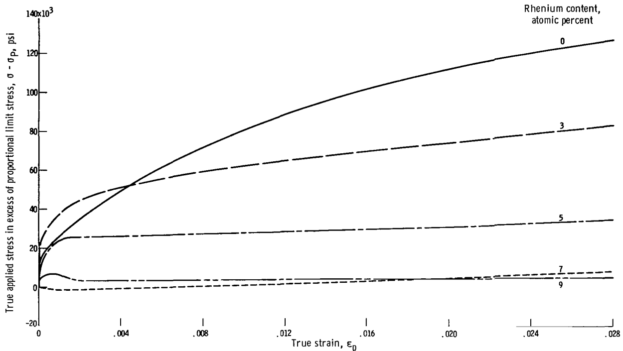
Figure 5. - Effect of rhenium on flow stress in excess of proportional limit stress of \langle 100 \rangle oriented tungsten single crystals.
