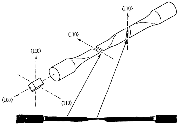
Figure 7. - Tungsten - 9 atomic percent rhenium tensile specimen after 15 percent strain.
