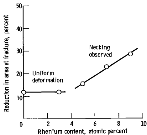
Figure 6. - Effect of rhenium on reduction in area of \langle 100 \rangle oriented tungsten single crystals.
