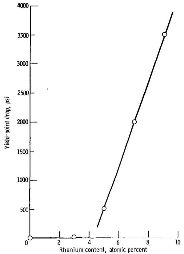
Figure 4. - Yield-point drop exhibited by \langle 100 \rangle oriented tungsten crystals with rhenium in solid solution.
