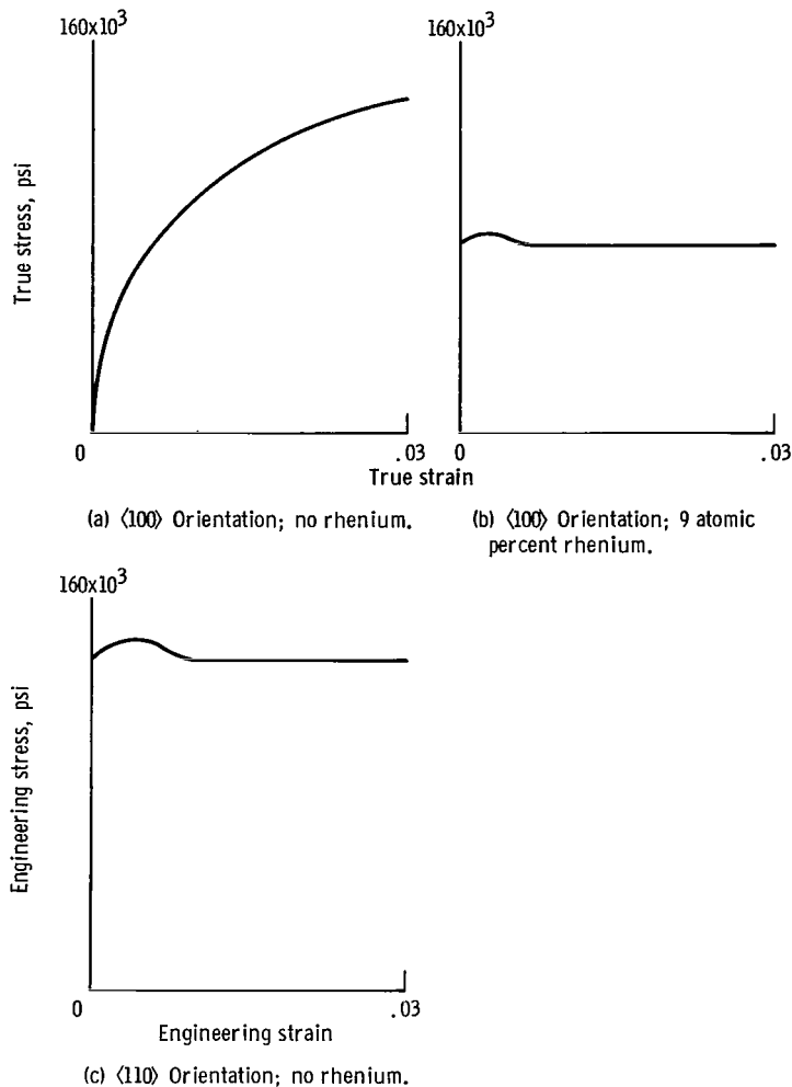
Figure 12. - Effect of orientation and rhenium content on tensile behavior of tungsten single crystals.
