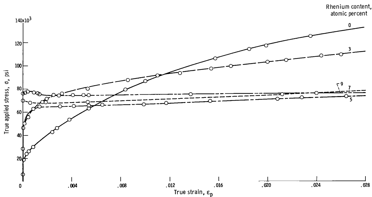
Figure 2. - Tensile curves of \langle 100 \rangle oriented tungsten single crystals containing various rhenium contents. Beyond 0.030 strain localized deformation occurs in 5, 7, and 9 atomic percent rhenium specimens.
