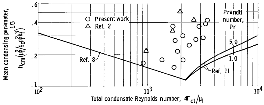
Figure 12. - Mean condensing heat-transfer parameter as function of total condensate Reynolds number.
