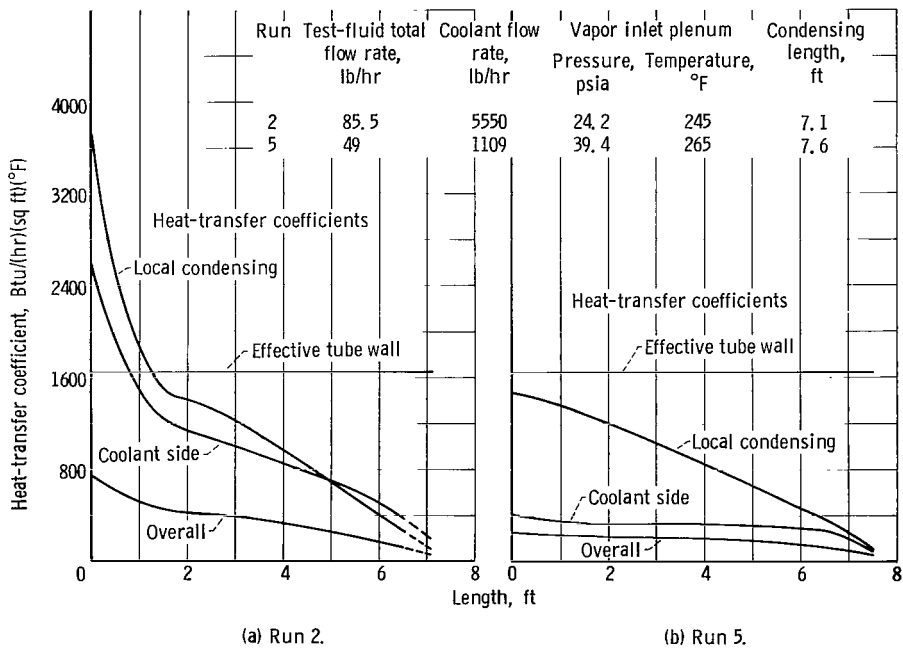
Figure 11. - Variation of individual and overall heat-transfer coefficients with length.
