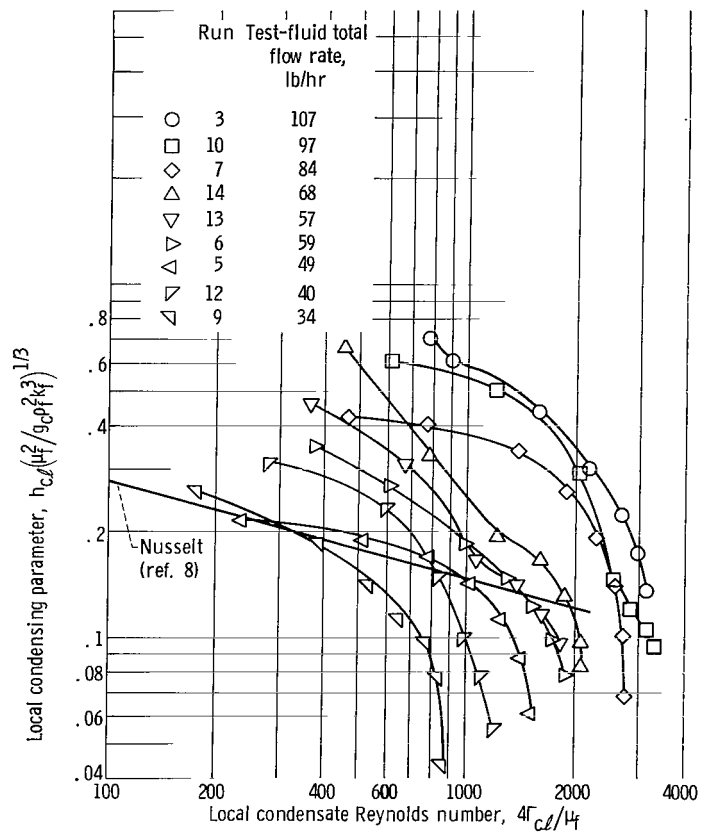
Figure 9. - Local condensing heat-transfer parameter as function of local condensate Reynolds number.
