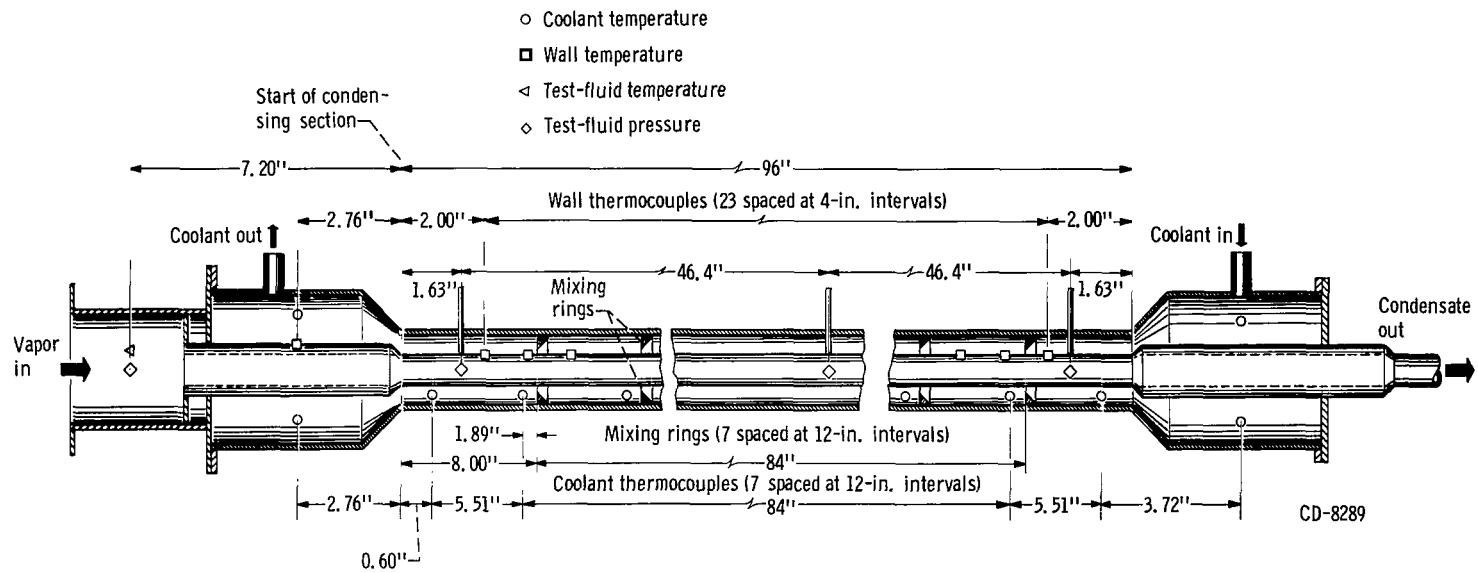
Figure 4. - Test-section instrumentation.
