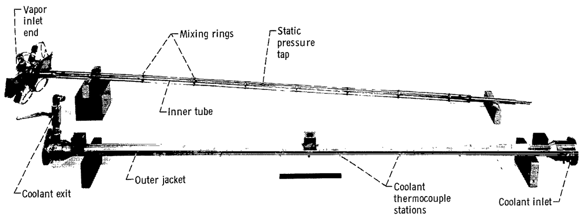
Figure 3. - View of inner tube and outer jacket of test condenser.
