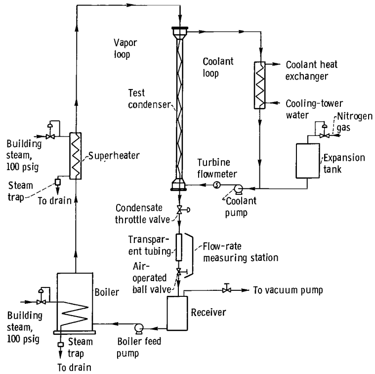
Figure 1. - Schematic drawing of single-tube steam-condensing apparatus.
