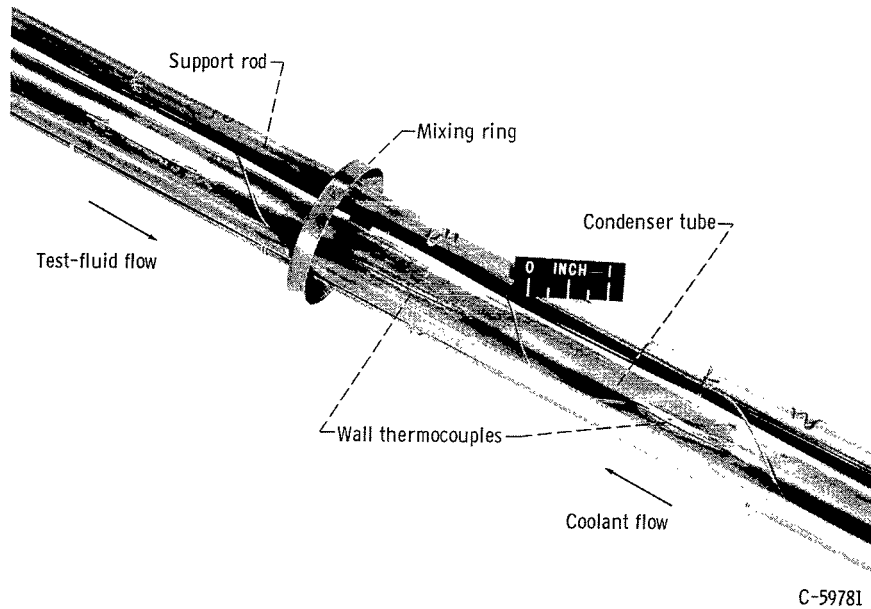
Figure 5. - Condenser tube wall thermocouple installation.
