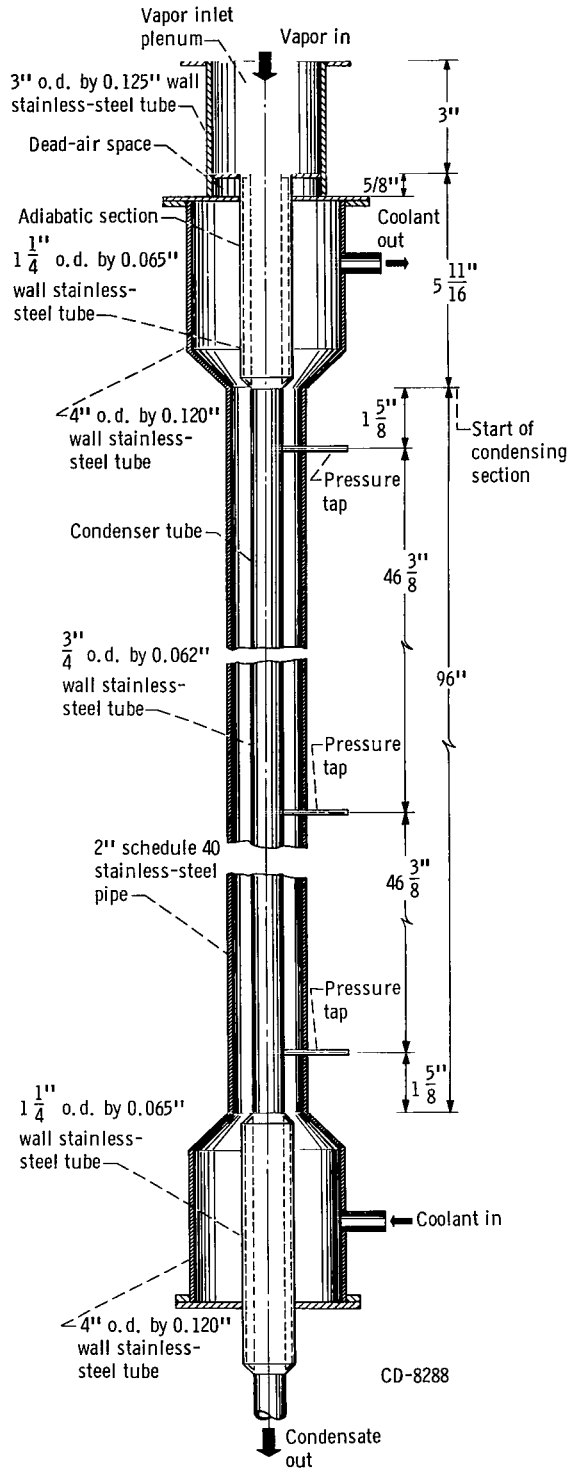
Figure 2. - Schematic drawing of single-tube-condenser test section.
