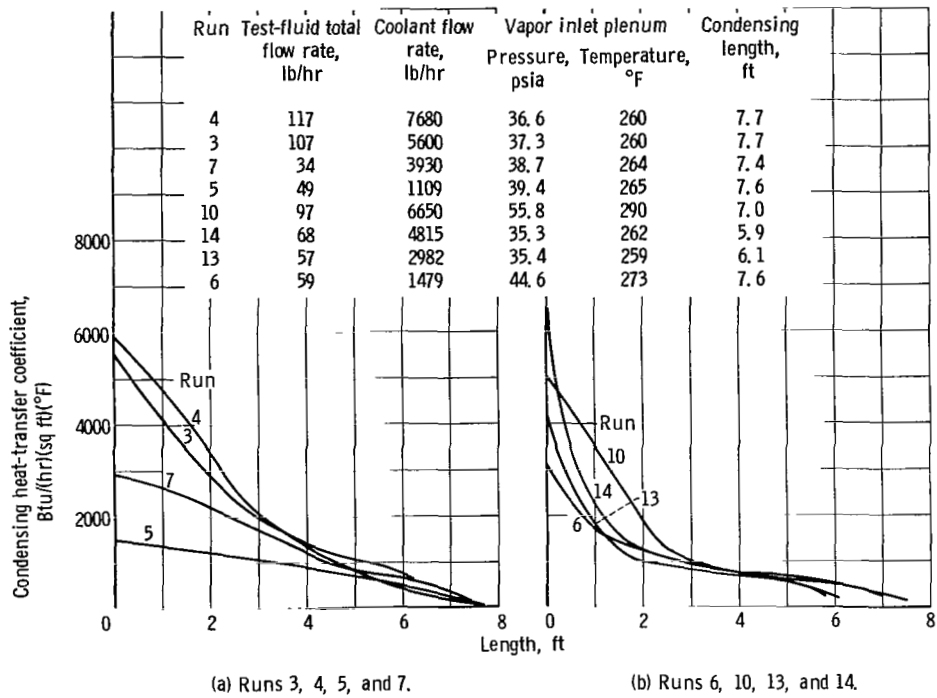
Figure 8. - Variation of condensing heat-transfer coefficient with length for single-tube steam-condensing tests.
