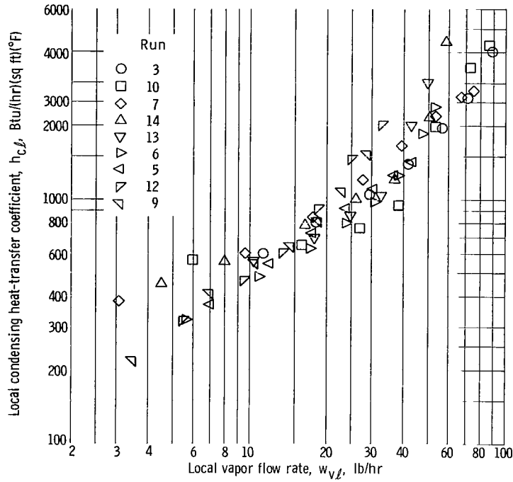
Figure 10. - Local condensing heat-transfer coefficient as function of vapor flow rate.
