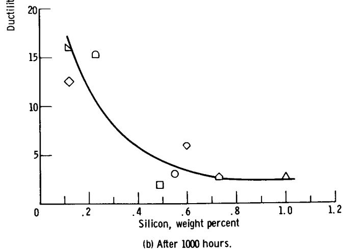
Fig. 3. - Effect of silicon content on average room-temperature ductility after aging at 1600° F.
