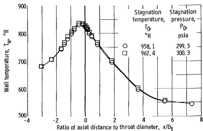
Figure 7. - Nozzle wall temperature distribution. Throat diameter, 1.492 inches.
