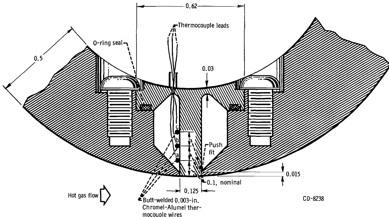
Figure 4. - Inconel heat-flux meter at nozzle throat. (All dimensions in inches.)
