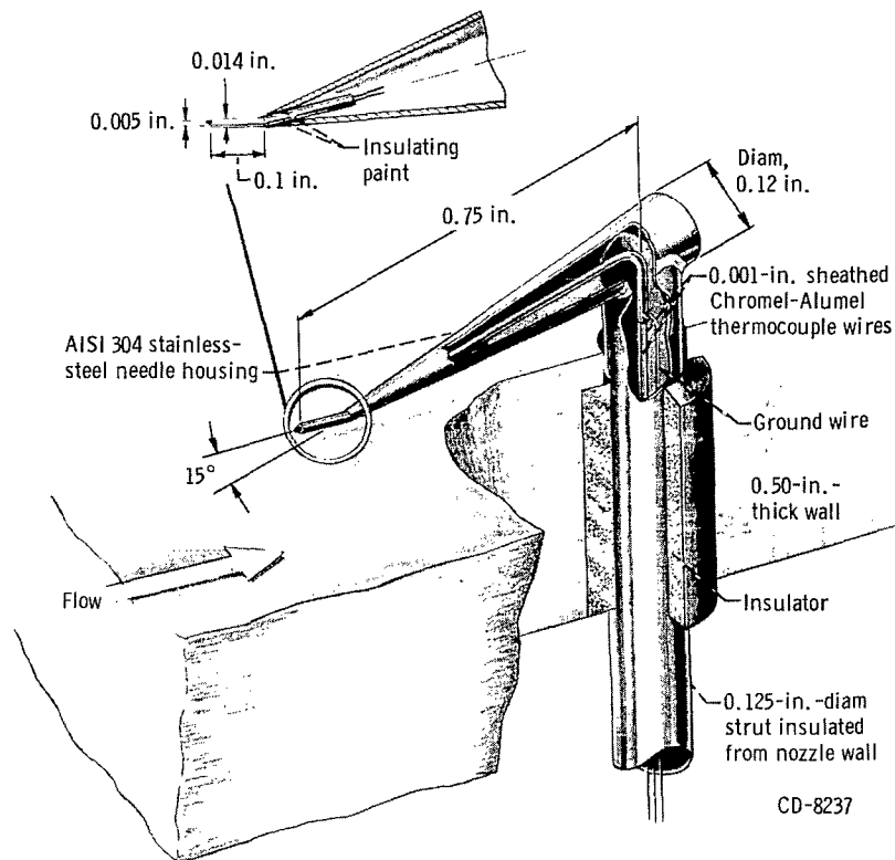
Figure 5. - Boundary layer temperature probe.
