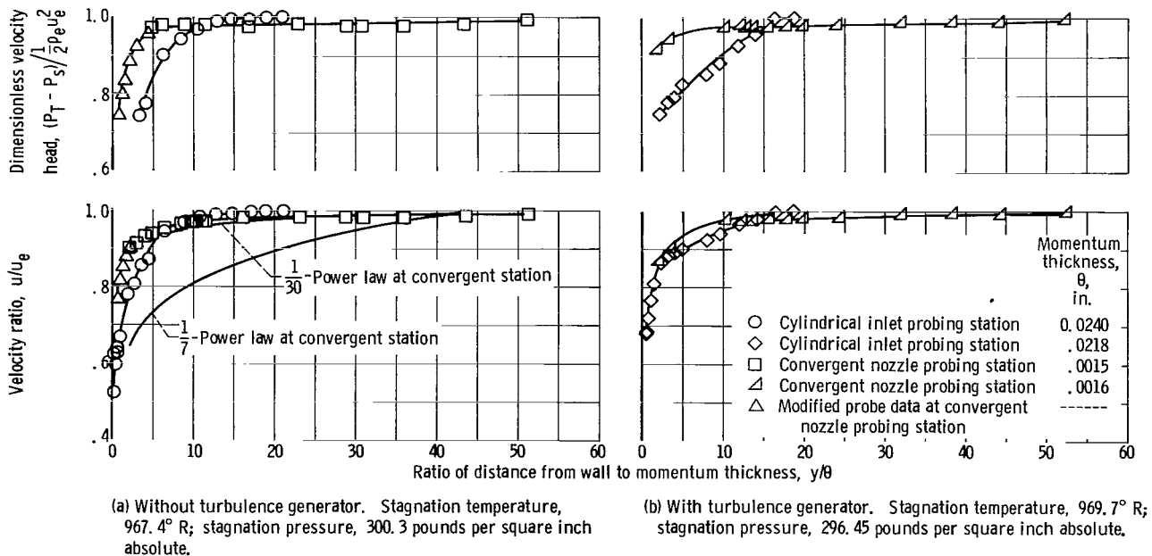
Figure 10. - Velocity profiles at cylindrical inlet and convergent nozzle probing stations.
