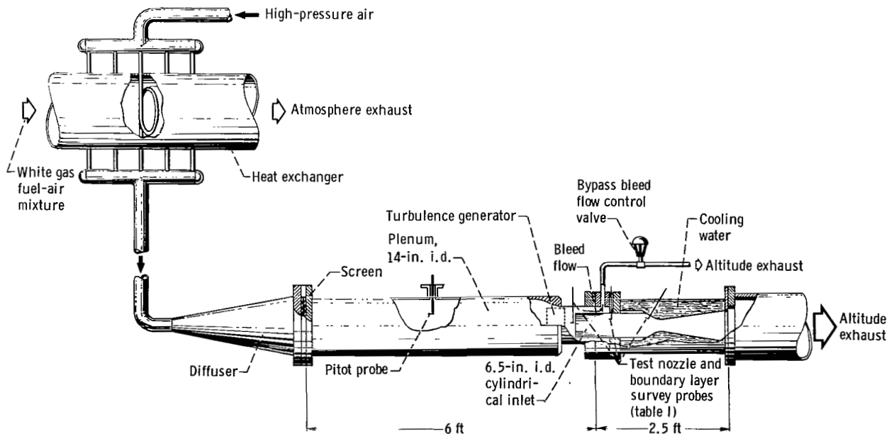
Figure 1. - Schematic diagram of nozzle heat-transfer facility.
