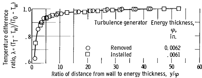
Figure 9. - Temperature profiles at convergent nozzle probing station with and without turbulence generator.
