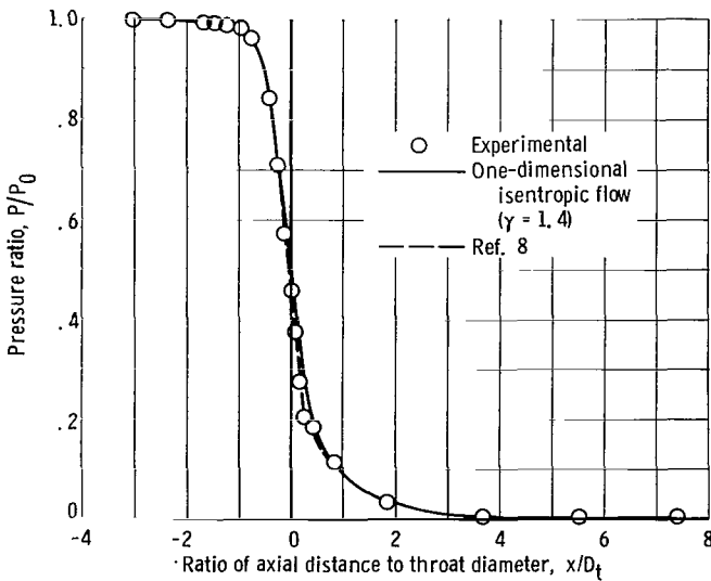
Figure 6. - Pressure ratio for conical nozzle in air. Total pressure, 300 pounds per square inch absolute; total temperature, 967° R; throat diameter, 1.492 inches.
