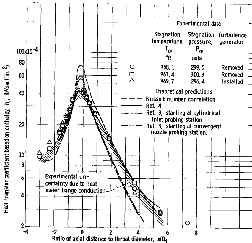
Figure 13. - Variation of experimental heat-transfer coefficient along nozzle and comparison with theoretical predictions. Throat diameter, 1.492 inches.
