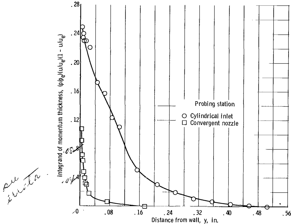
Figure 11. - Variation of integrand of momentum thickness across boundary layer for cylindrical inlet and convergent nozzle probing stations.
