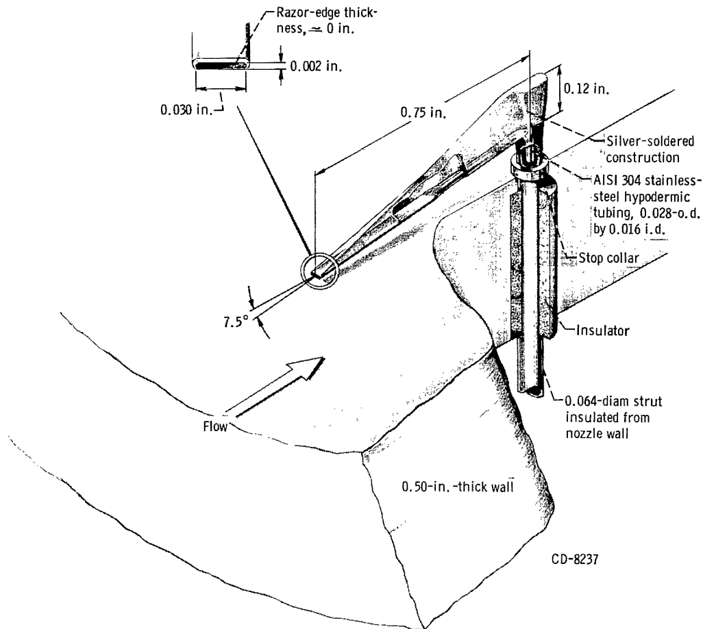
Figure 3. - Boundary layer pressure probe.
