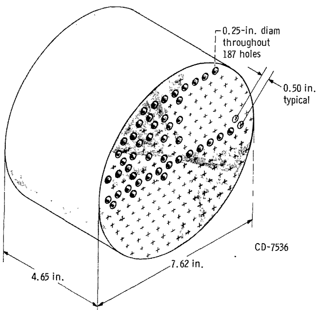
Figure 2. - Upstream turbulence generator (reactor core simulator).
