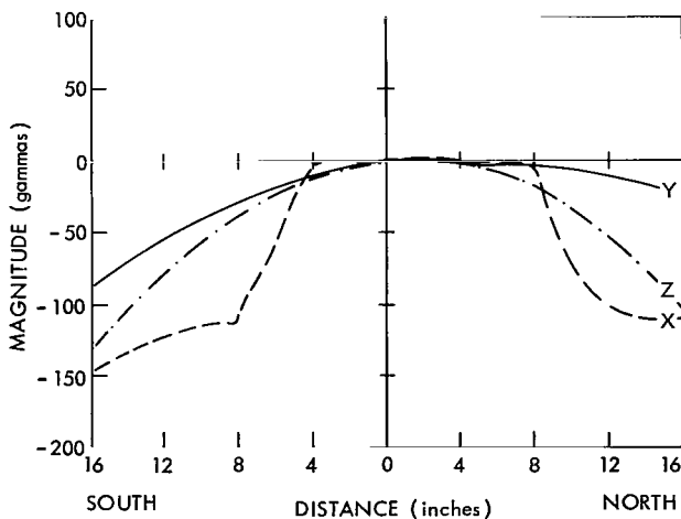
Figure B-4—Zero field - Y coil axis.
