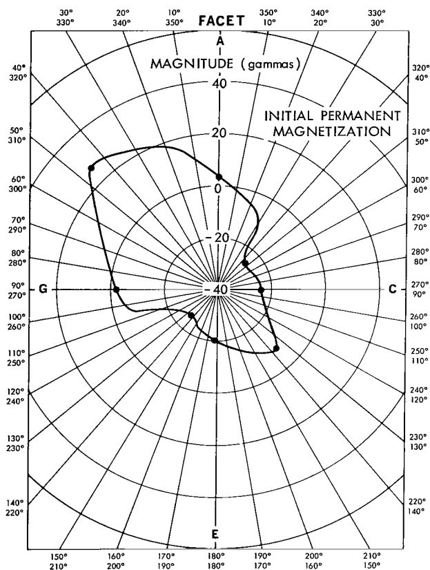
Figure 1—Magnetic field disturbance of spacecraft - Radial component ( H_x ). Initial permanent magnetization in gamma at 27.8 inches.
