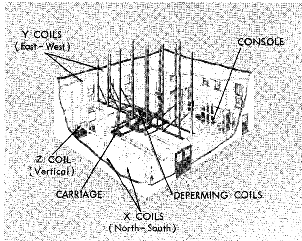
Figure B-9--Naval Ordnance Laboratory - Magnetic Test Facility, Building 206.
