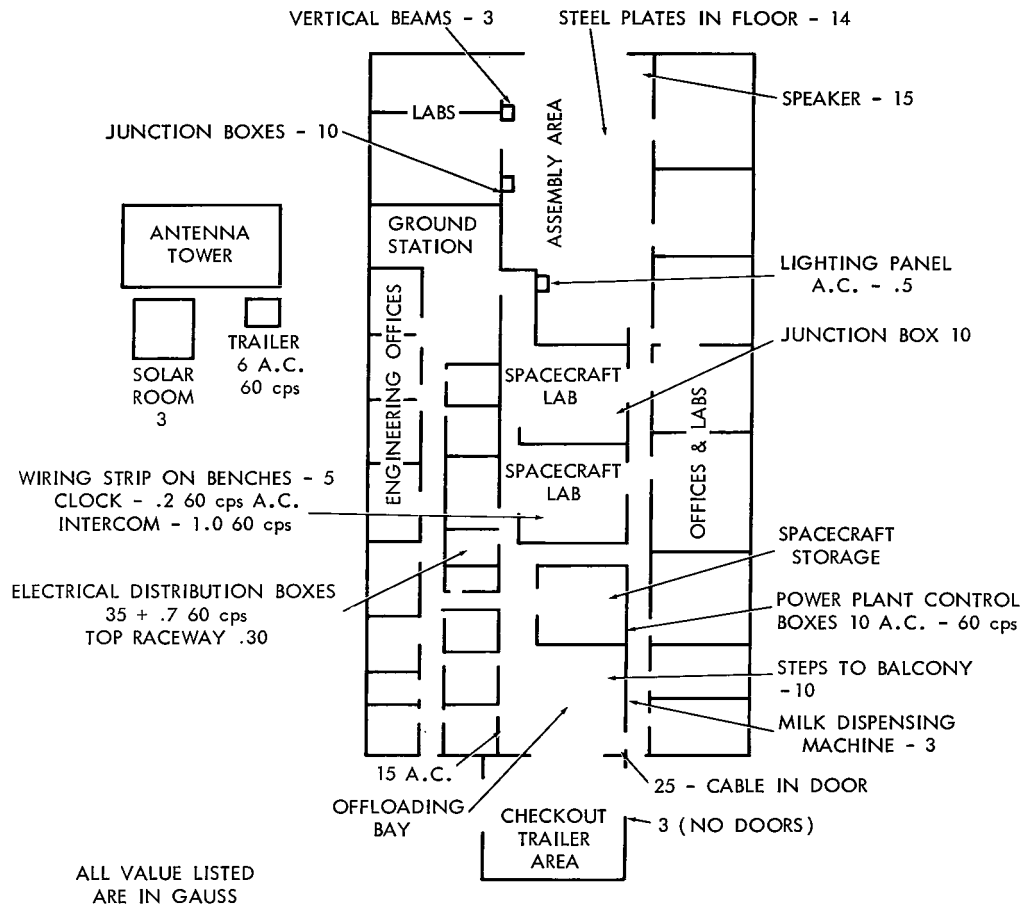
Figure H-3--Spacecraft laboratory Building A-E.
