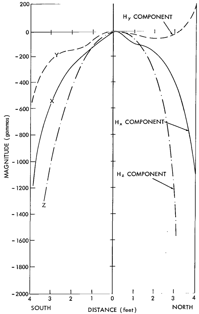
Figure B-7— H_y horizontal axis gradient zero field.
