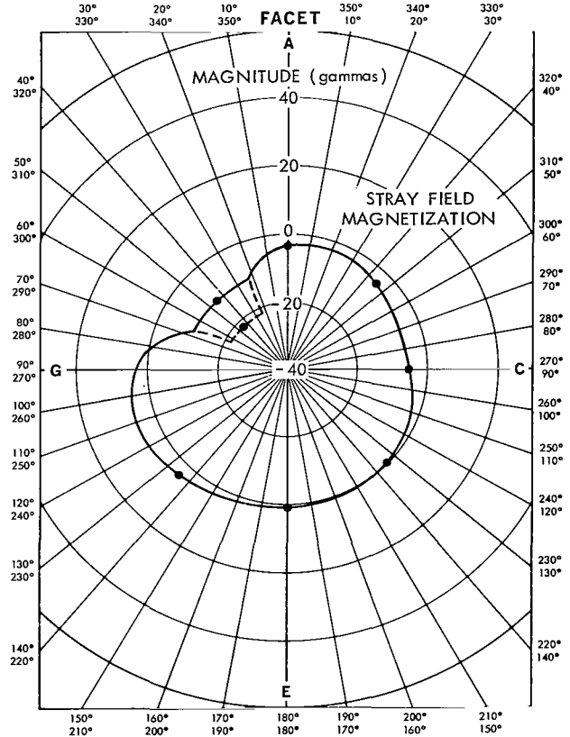
Figure 8—Stray magnetic field disturbance of spacecraft - Radial component ( H_x ). (Magnitude in gamma at 27.8 inches.)
