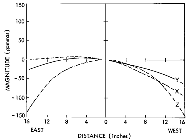
Figure B-5—Zero field - X coil axis.
