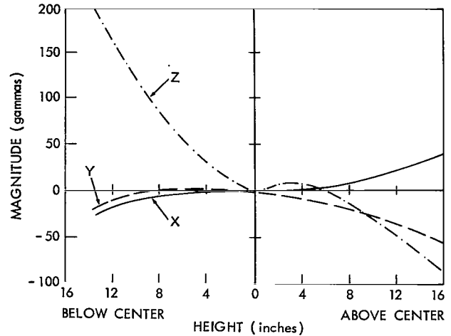
Figure B-3—Zero field - Z coil axis.
