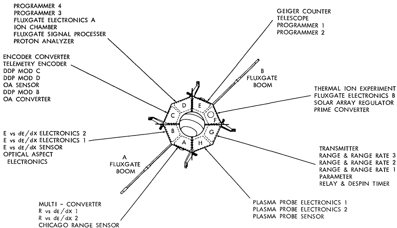
Figure 2—IMP-I (Explorer XVIII) Spacecraft.
