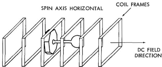
Figure C-3—Test arrangement for exposure and deperming of spacecraft.
