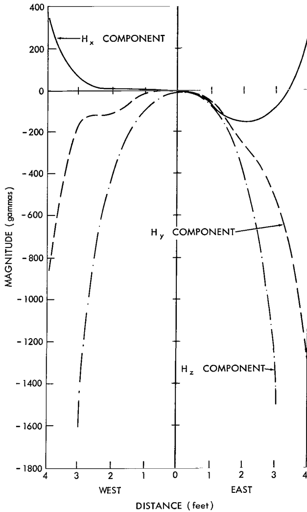
Figure B-6— H_x horizontal axis gradient zero field.
