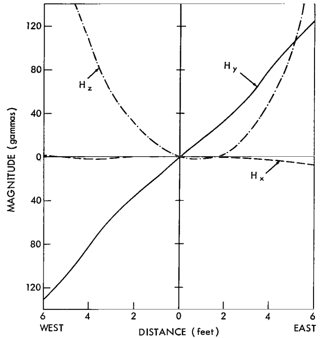
Figure B-11—Zero field - Y coil axis.
