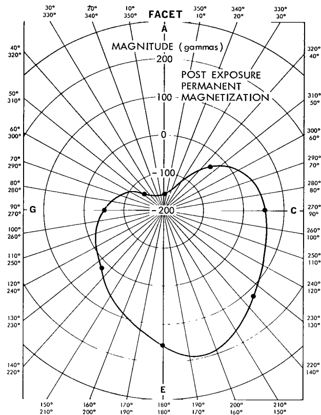
Figure 5—Magnetic field disturbance of spacecraft - Radial component ( H_x ). Post exposure in gamma at 2.7 inches.
