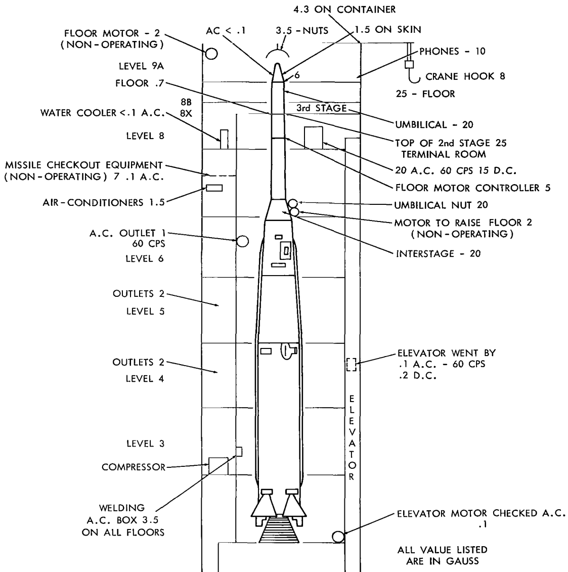
Figure H-2—Thor-Delta tower.
