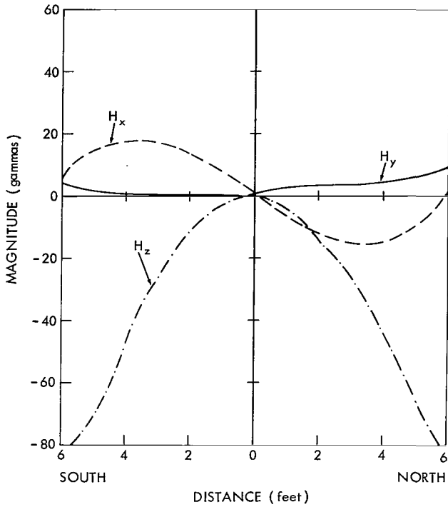
Figure B-10—Zero field - X coil axis.
