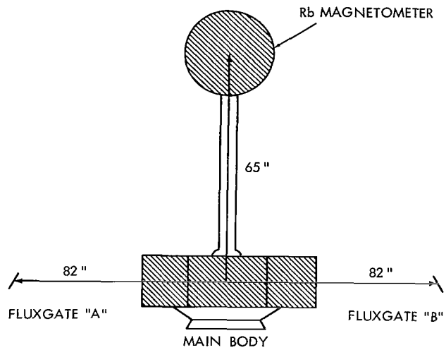
Figure A-2—Sketch of the IMP Spacecraft illustrating location of fluxgate and rubidium magnetometer sensor.
