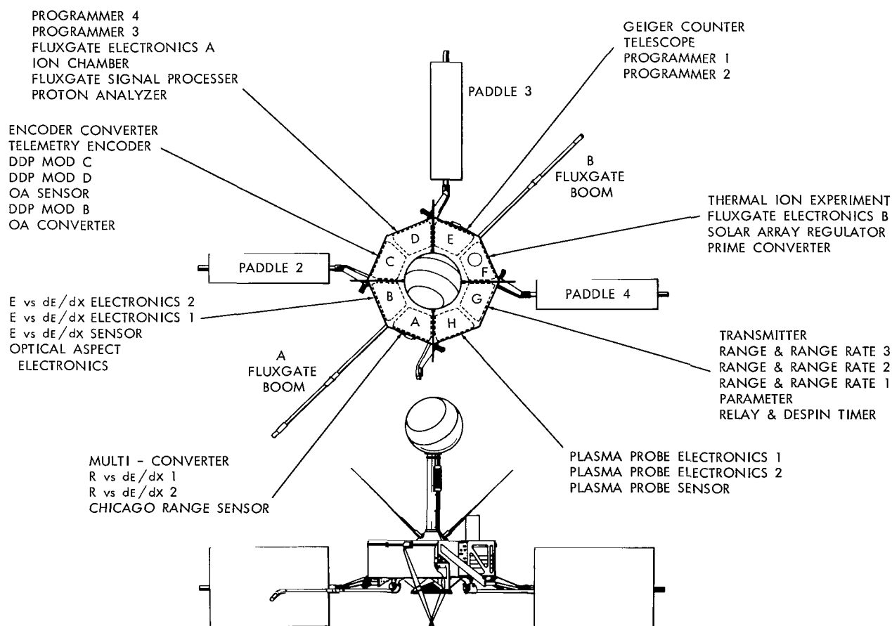
Figure A-1—Interplanetary Monitoring Probe (IMP, S-74).
