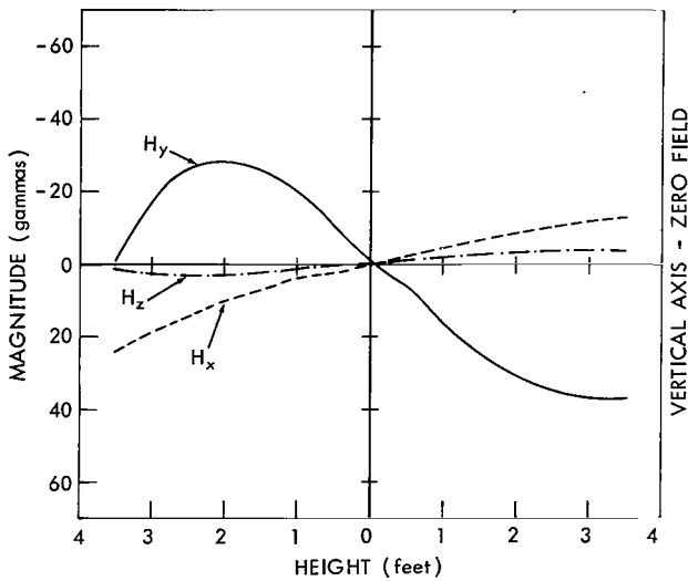
Figure B-12—Zero field - Z coil axis.
