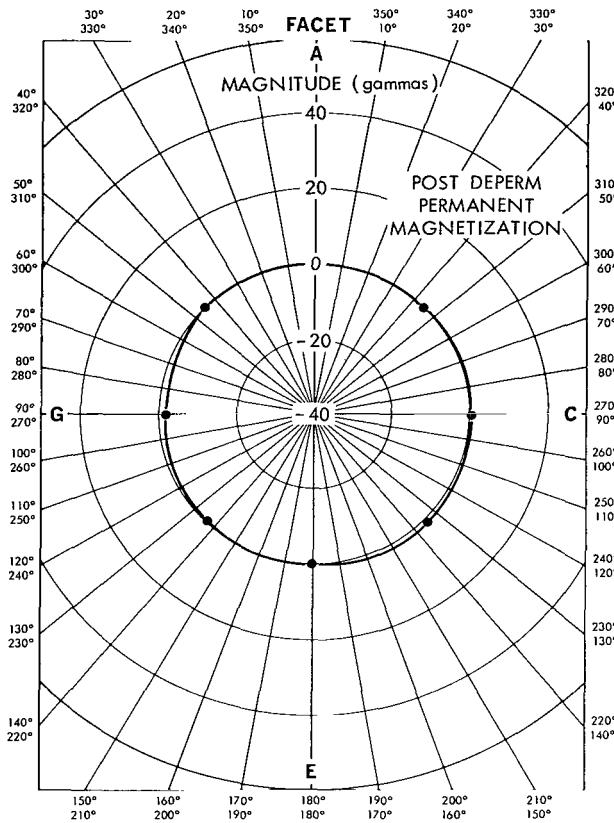
Figure 3—Magnetic field disturbance of spacecraft - Radial component ( H_x ). Post deperm permanent magnetization in gamma at 27.8 inches.
