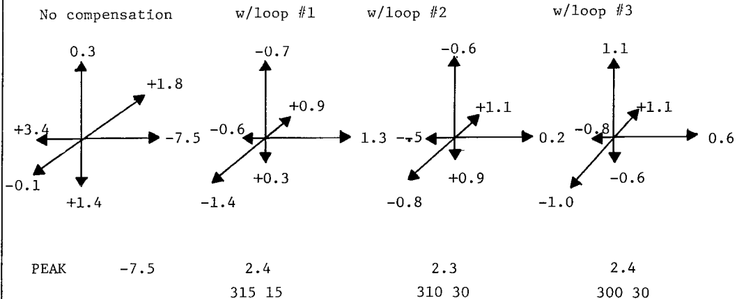
RADIAL COMPONENT OF MAGNETIC FIELD IN GAMMA AT 18 INCH
