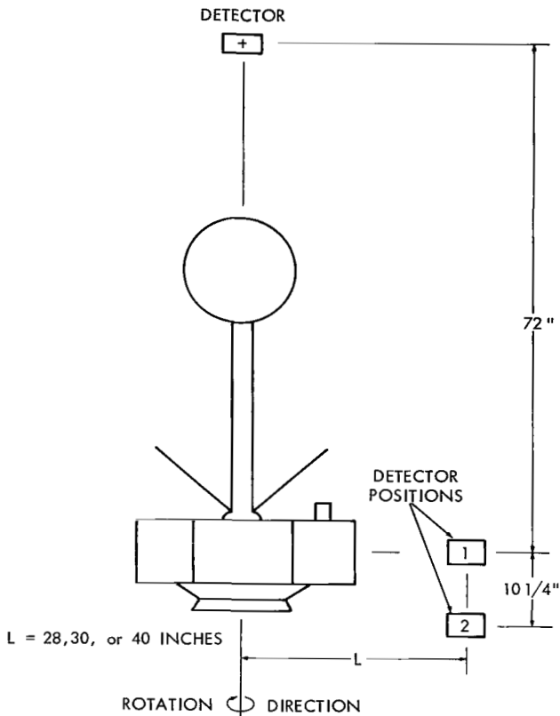
Figure C-1—Test arrangement for vertical spin axis rotation of spacecraft.
