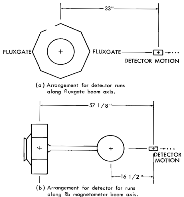
Figure C-2—Test arrangement for fall-off with distance along spin and boom axis.
