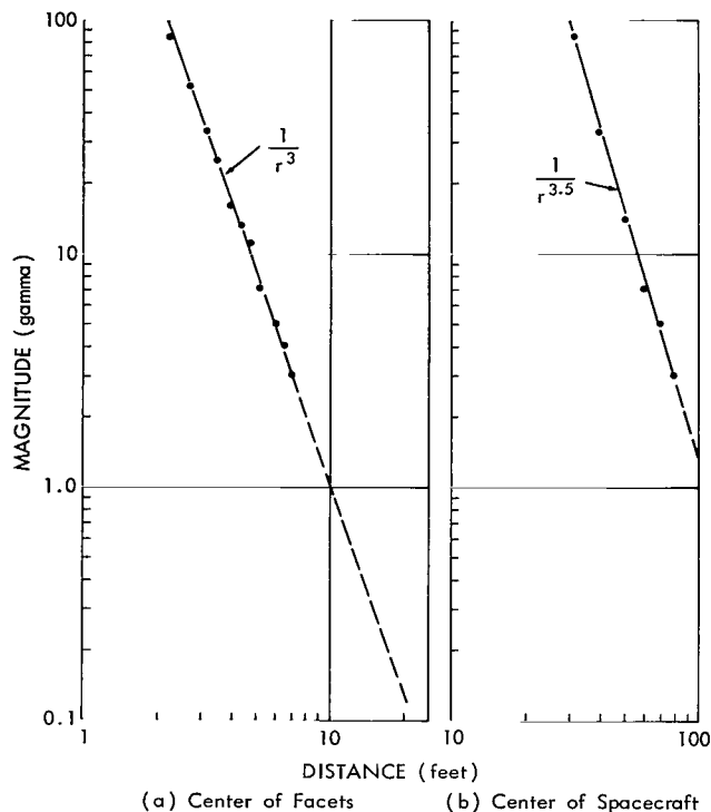
Figure 6—Magnetic field change versus distance (fall-off) along fluxgate-A boom Axis. Post exposure.
