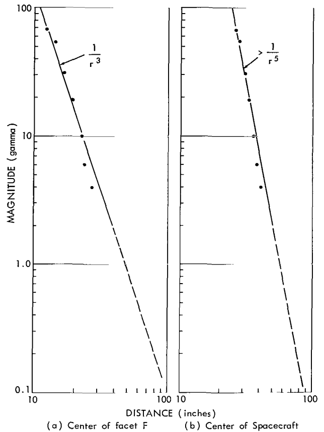
Figure 4—Magnetic field change versus distance (fall-off) from Facet F. Initial perm.
