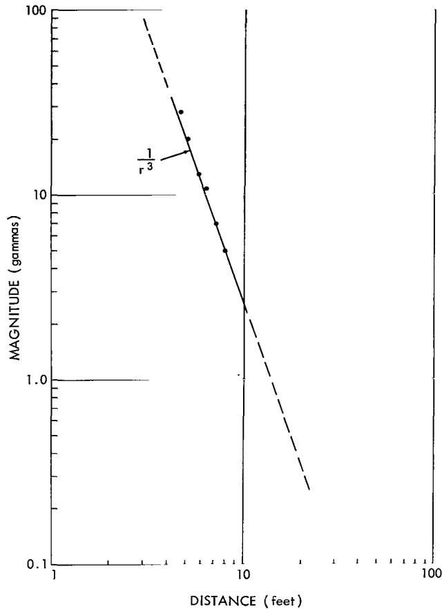
Figure 7—Magnetic field change versus distance (fall-off) along spin axis. Post exposure.
