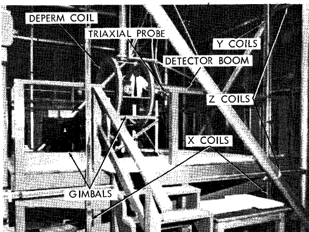
Figure B-2—Component Magnetic Test Facility.
