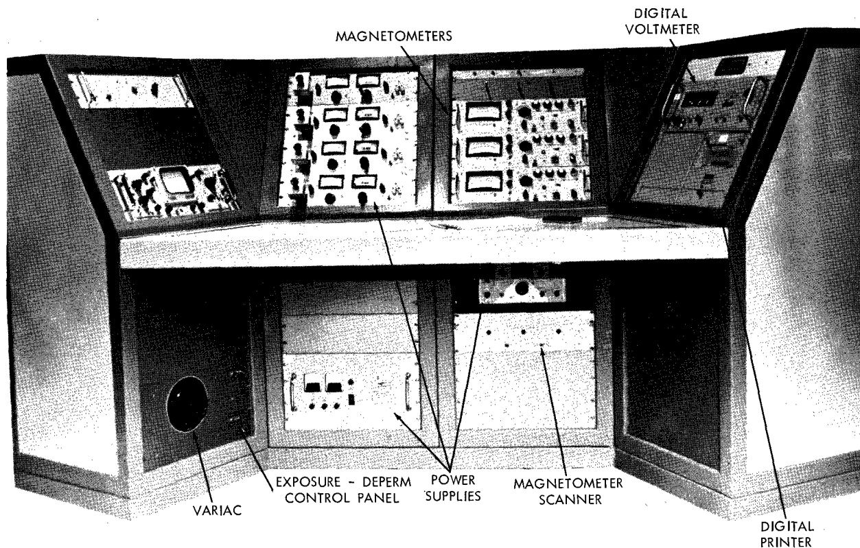
Figure B-8—Control console.
