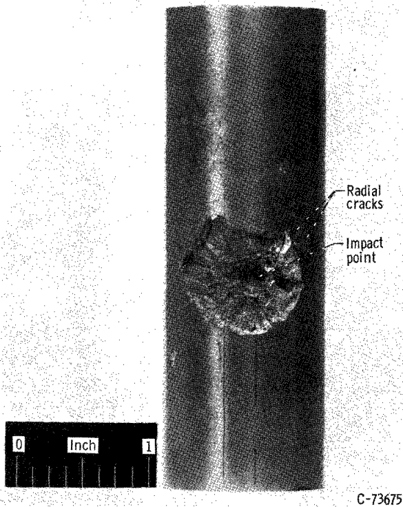
Figure 7. - Fiber-reinforced beryllium-armed tube after impact (target 3). Test conditions: projectile, 3/32-inch-diameter pyrex sphere; impact velocity, 24 000 feet per second; target temperature, 1300° F.
