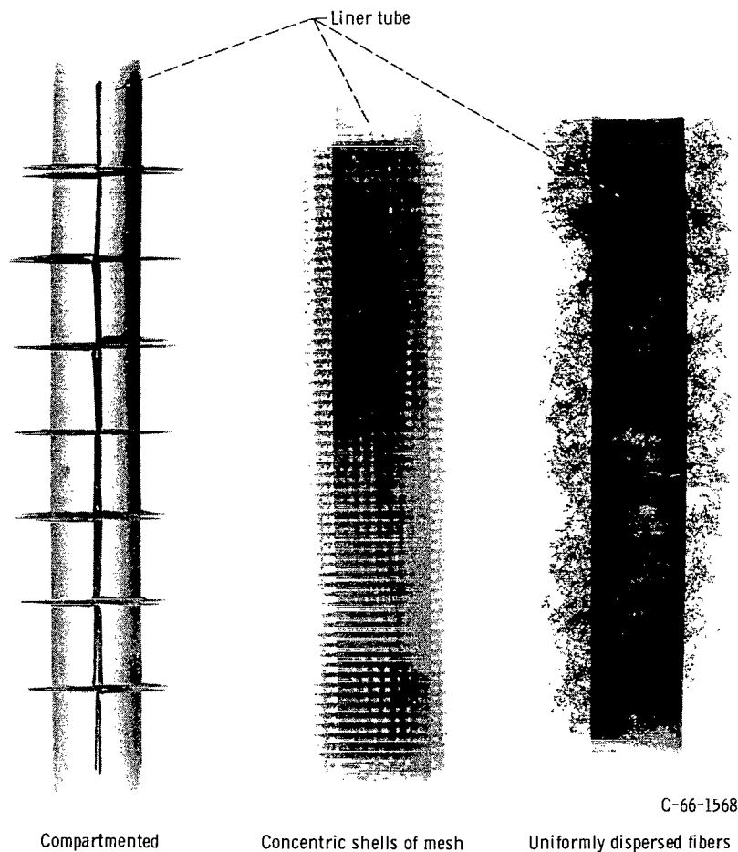
Figure 3. - X-ray prints of AISI 316 stainless-steel reinforcements in beryllium-armored tubes.
