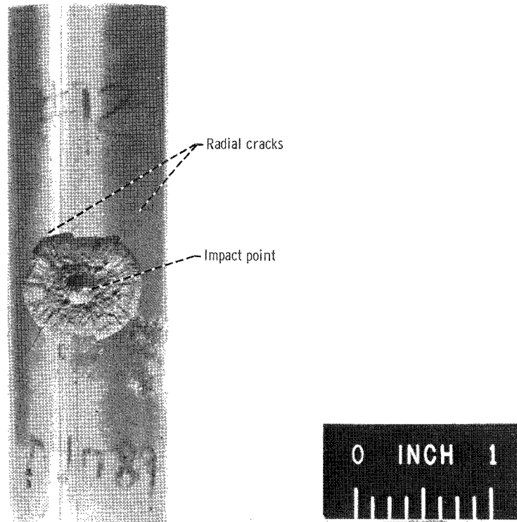
Figure 6. - Mesh-reinforced beryllium-armored tube after impact (target 2). Test conditions: projectile, 3/32-inch-diameter pyrex sphere; impact velocity, 23 600 feet per second; target temperature, 1300° F.
