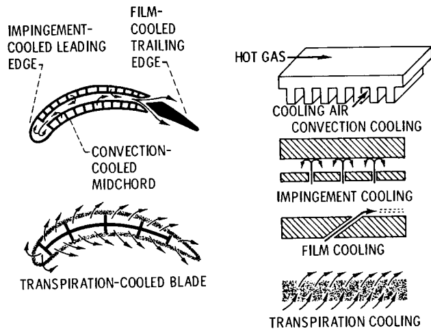
Figure 3. - Methods of turbine-blade cooling.
