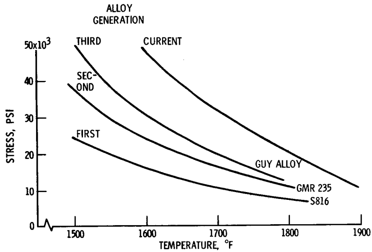
Figure 1. - 100-Hour stress-rupture life of various alloys.
