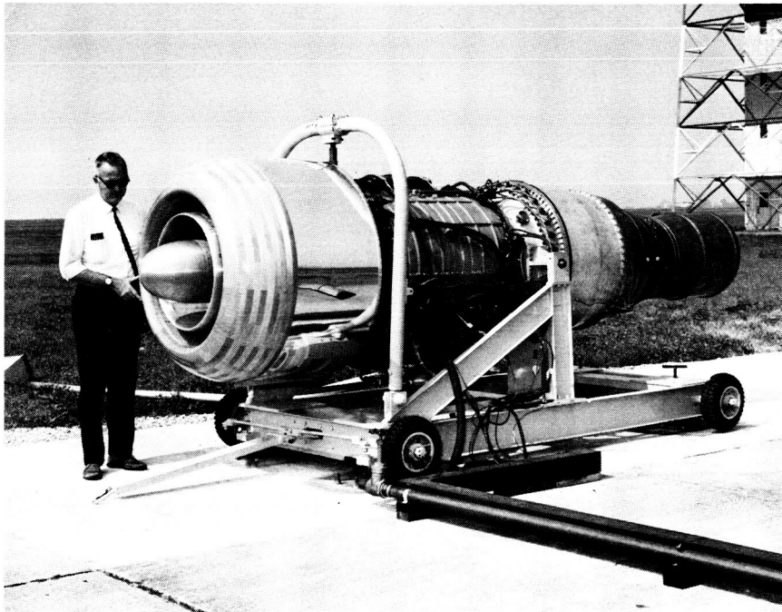
Figure 13. - Noise reduction cowl installed on J-65 engine.
