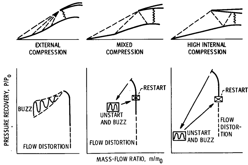
Figure 6. - Inlet characteristics.
