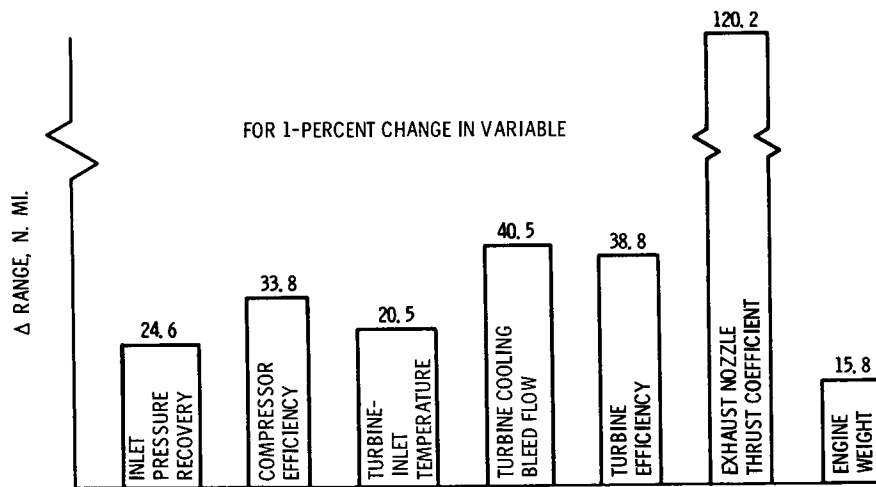
Figure 8. - Effect of engine characteristics on range for large turbojet-powered aircraft; Mach 3.
