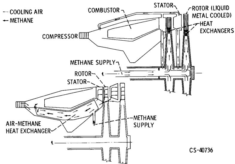
Figure 10. - Alternate turbine cooling methods with methane fuel.
