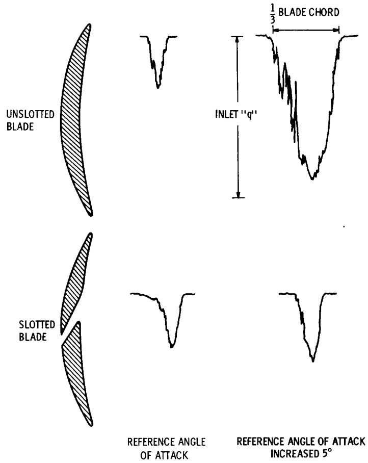
Figure 15. - Wake profiles of compressor blades.
