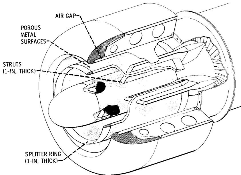
Figure 12. - Engine cowling modified to reduce noise.
