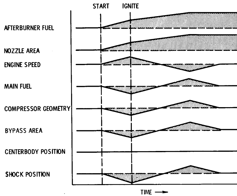
Figure 7. - Typical start transient.
