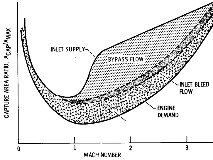
Figure 5. - Airflow matching.
