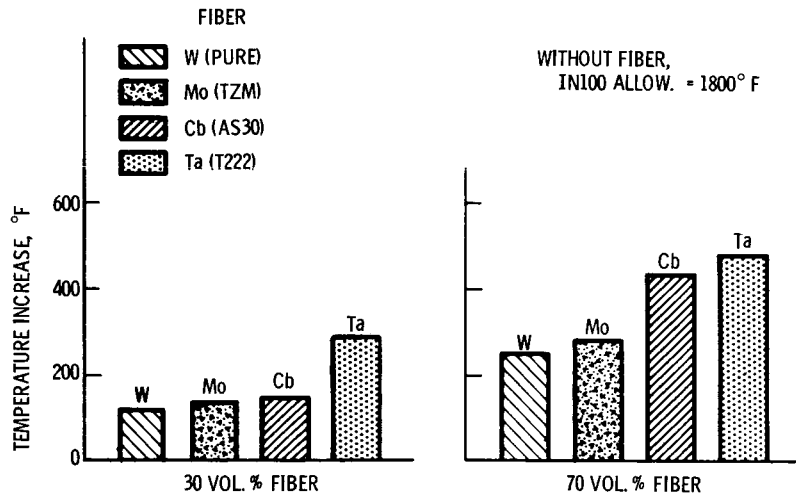
Figure 2. - Increase in allowable temperature by addition of refractory fibers to super-alloy (IN100) (calculated). Strength/density, 52 500 inches for 1000 hours.
