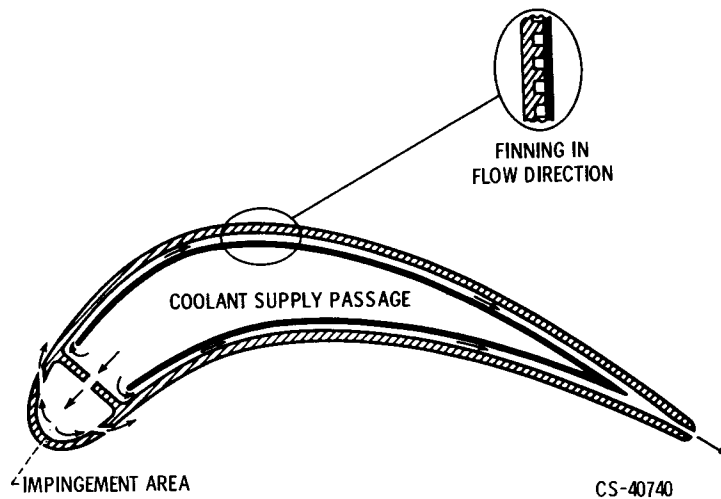
Figure 4. - Advanced cooled-blade configuration.
