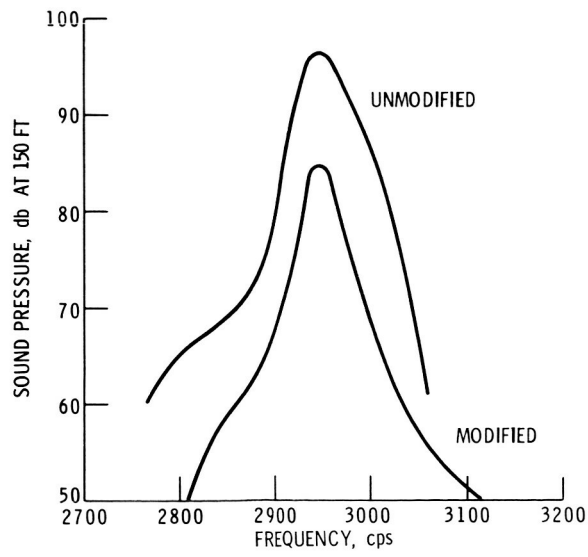
Figure 14. - Noise level with modified cowling.
