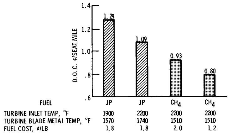
Figure 9. - Methane may reduce operating costs.
