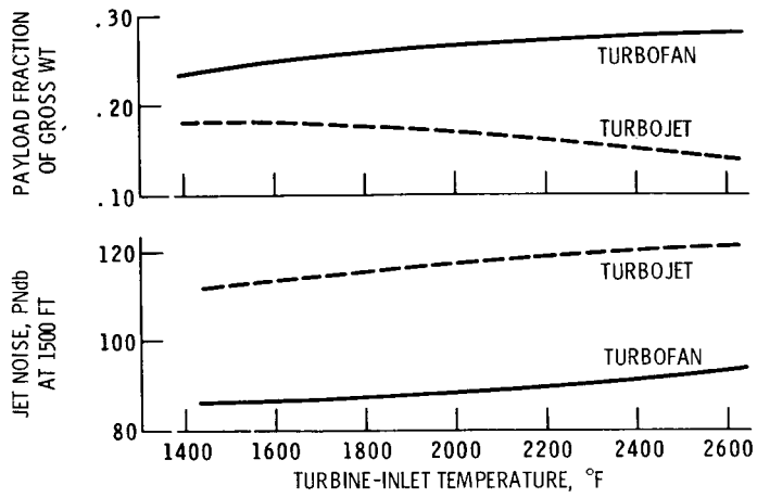
Figure 11. - Subsonic turbofan and turbojet airplane performance - noise level and payload. Mach 0.82; range, 4000 miles.
