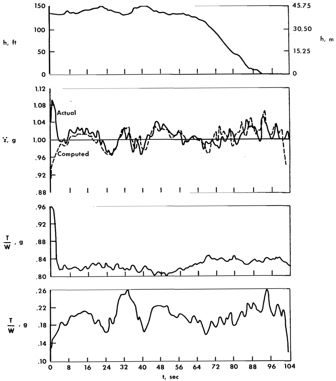
Figure 21.— Flight time history of LLRV automatic-throttle operation.
