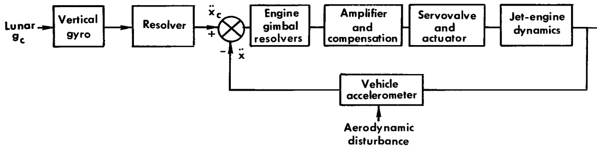
Figure 31.— Block diagram of lunar-gravity jet-engine stabilization system (pitch axis).
