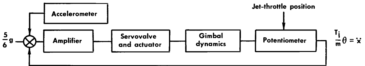
Figure 10.— Simplified block diagram of ground test setup for the pitch-axis jet-engine stabilization system closed-loop evaluation (similar diagram for roll axis).
