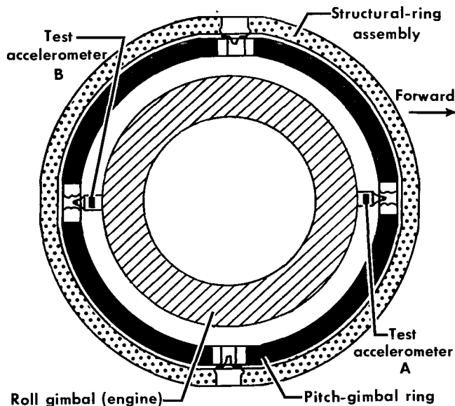
Figure 6.- Locations of accelerometers for jet stability tests.
