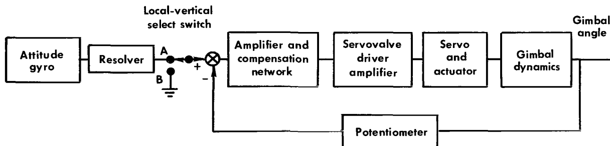
Figure 30.— Simplified block diagram of jet-engine attitude system, local-vertical and engine-centered modes.
