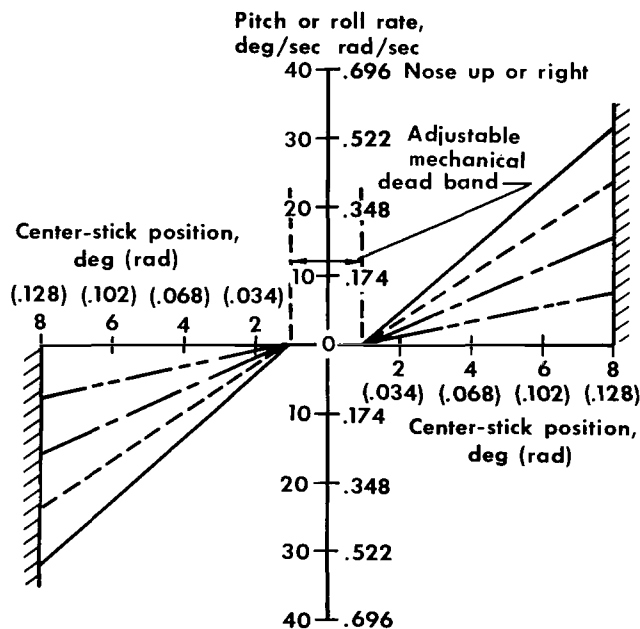
Figure 18.— LLRV angular rate command as a function of stick position.
