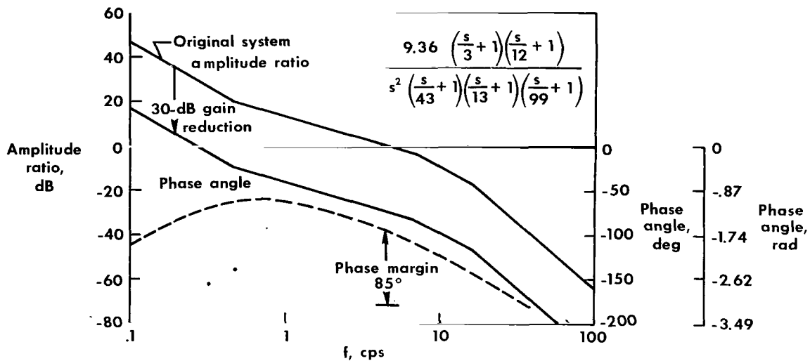
Figure 13.— Open-loop frequency response of the original jet-engine stabilization system.
