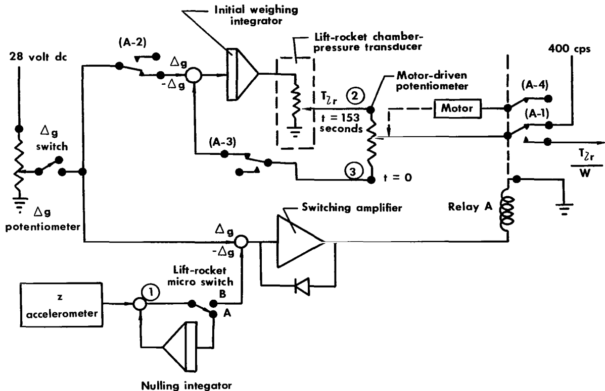
Figure 34.— Block diagram of \frac{T_{lr}}{W} computer and initial weighing circuitry.
