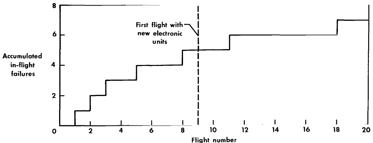
Figure 23.— In-flight failure history of LLRV electronics.
