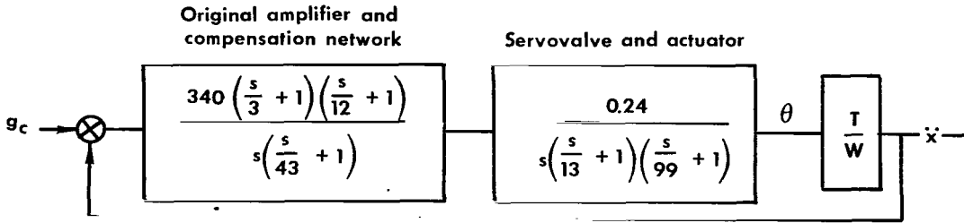
Figure 12.— Block diagram of original lunar-gravity simulation system (typical for pitch and roll).
