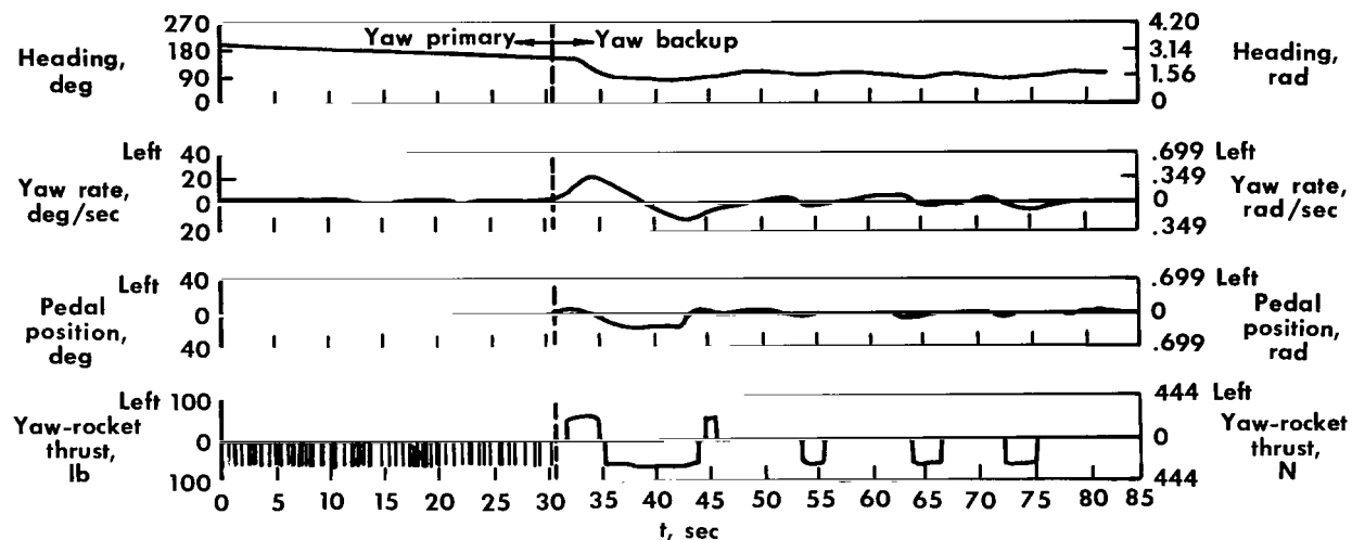
Figure 20.— Time history showing a yaw-damper failure.
