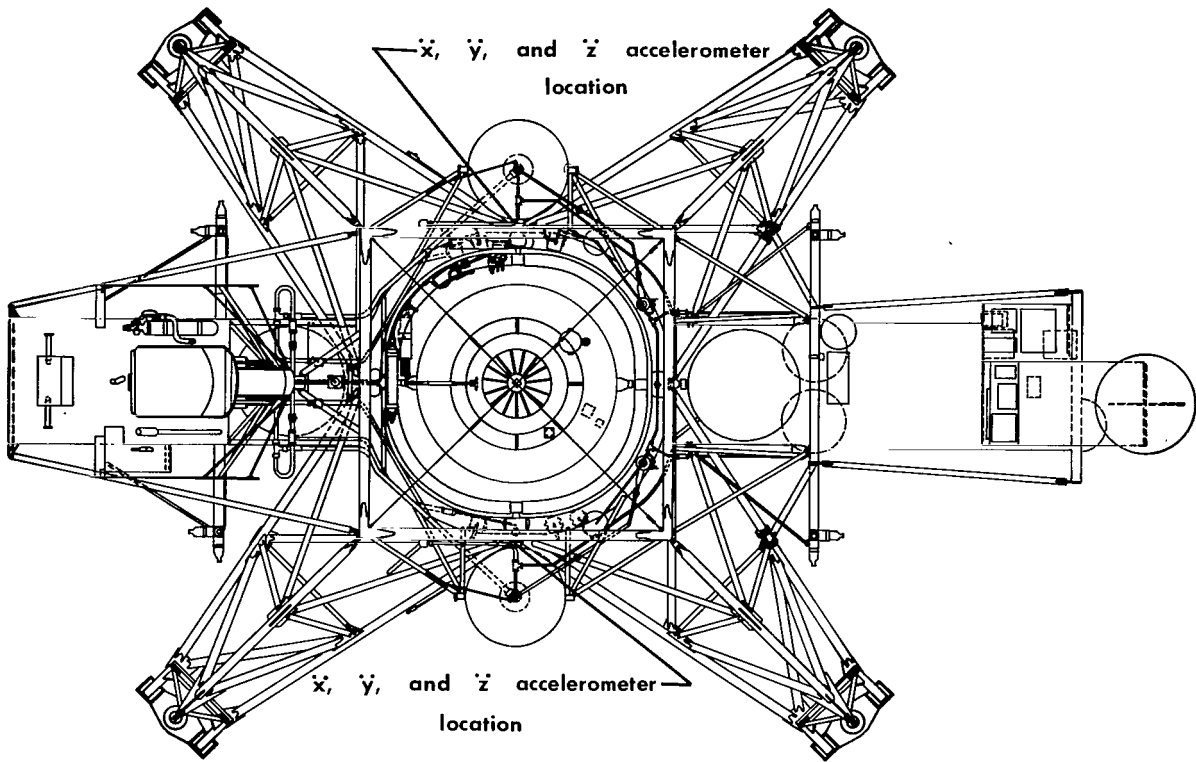
Figure 32.— Jet-stabilization-system accelerometer locations.
