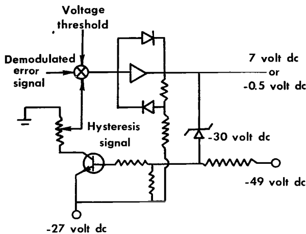
Figure 25.— Circuit diagram of switching amplifier.
