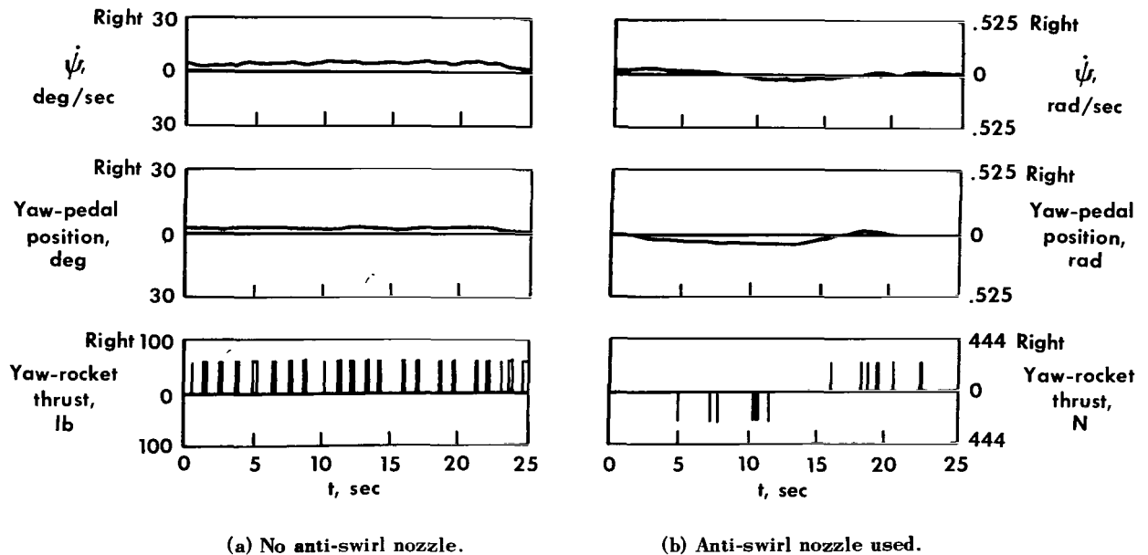
Figure 19.— Effect of jet fluid-air anti-swirl nozzle on yawing-moment compensation.
