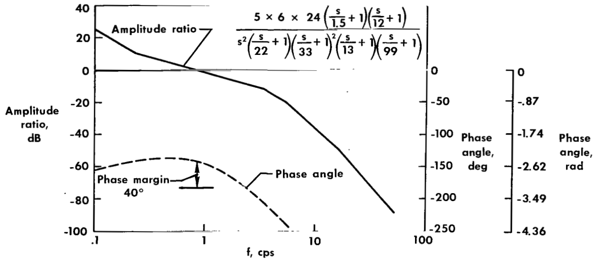
Figure 14.— Computed open-loop response of modified lunar-simulation system.
