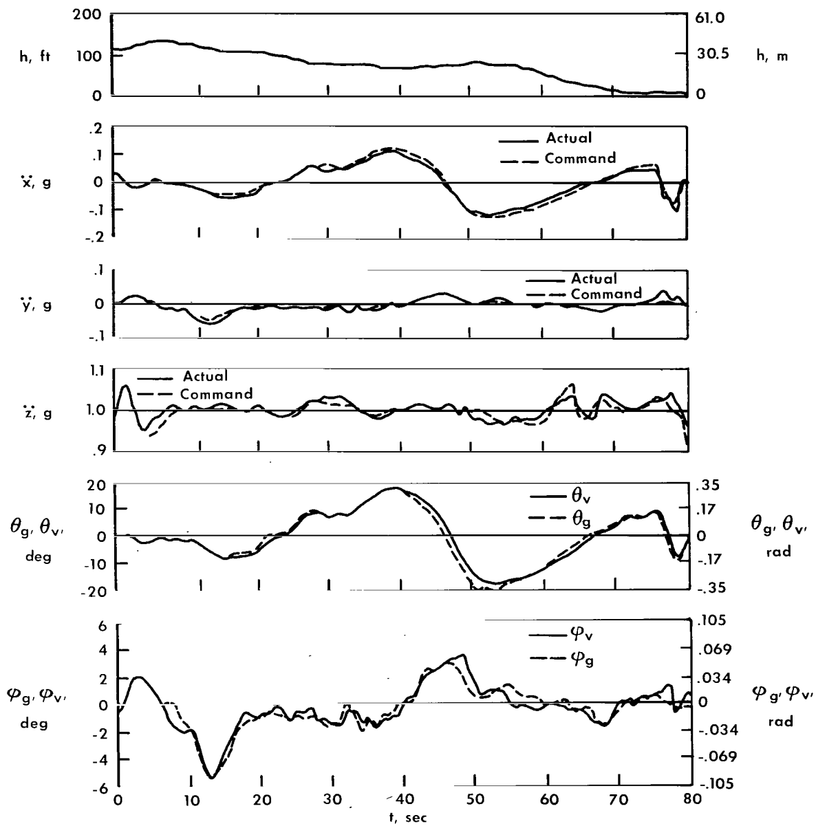
Figure 22.— Flight time history of LLRV lunar-simulation-system operation during a landing maneuver.
