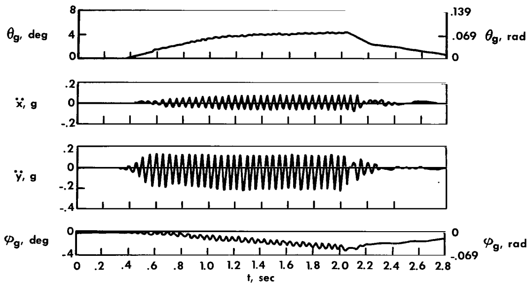
Figure 11.— Response of jet-engine stabilization system showing instability from structural vibration.
