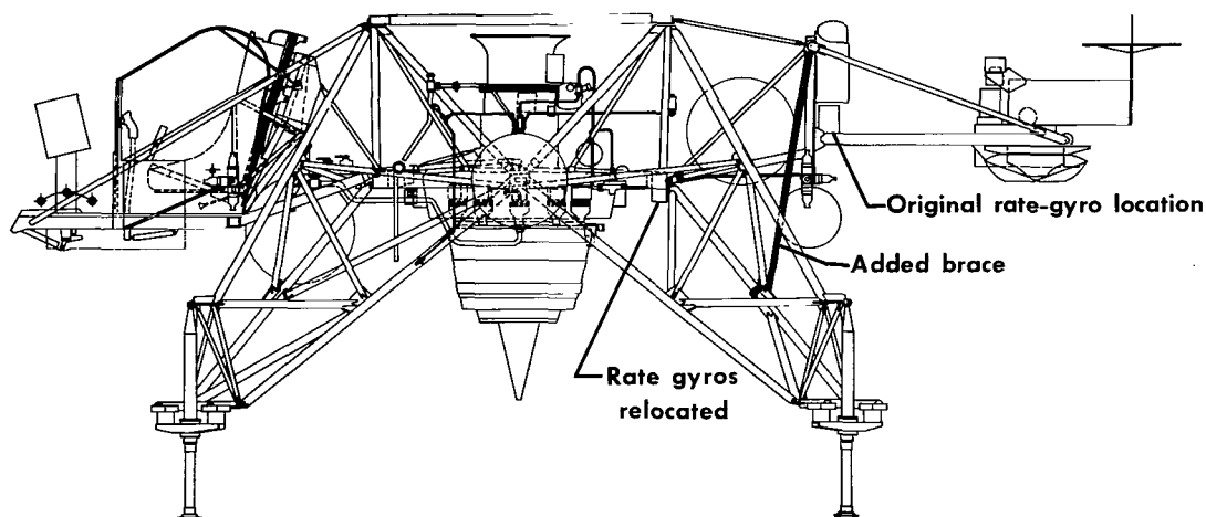
Figure 8.— Rate-gyro relocation.
