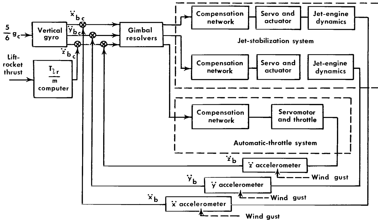
Figure 4.— Simplified block diagram of the LLRV lunar-simulation system.
