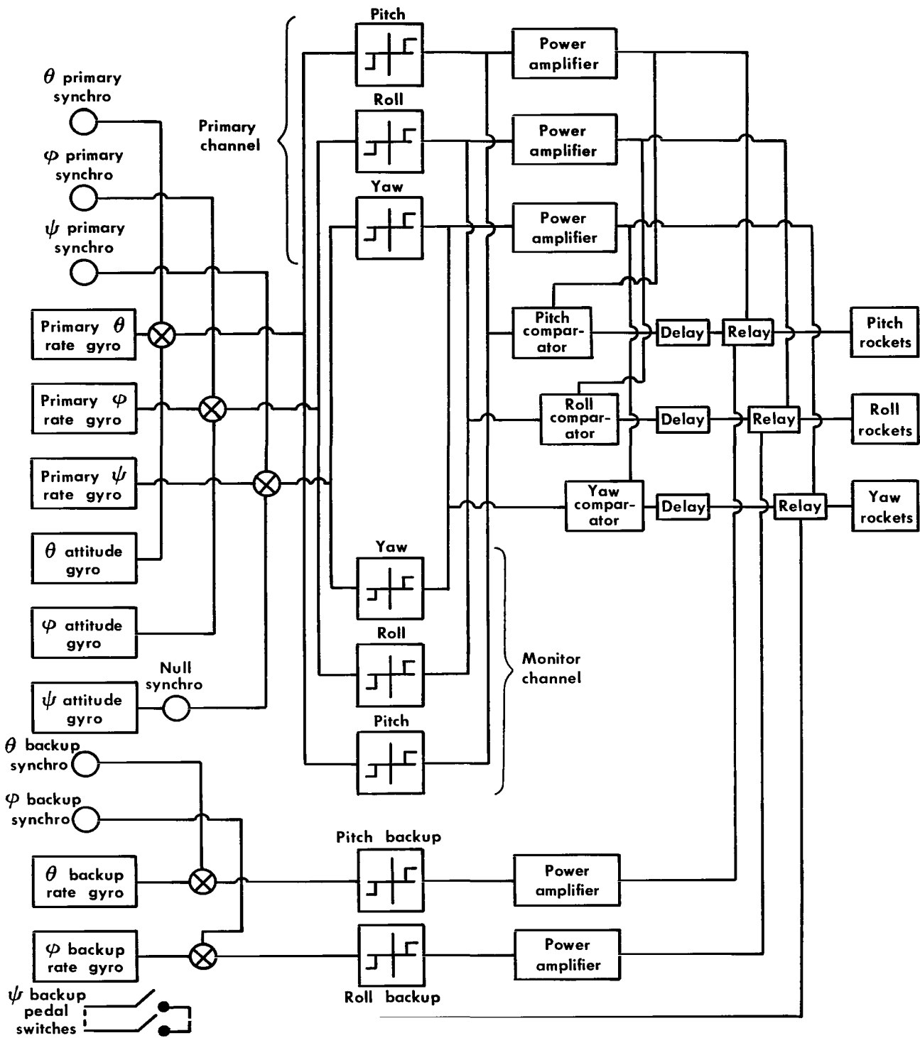
Figure 28.— Block diagram of primary and monitor circuitry of LLRV attitude control system.
