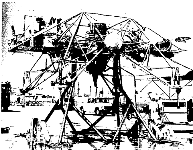
Figure 17.— LLRV attached to ground test fixture.
