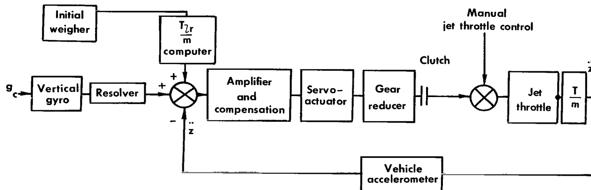
Figure 33.— Block diagram of lunar-gravity automatic-throttle system.
