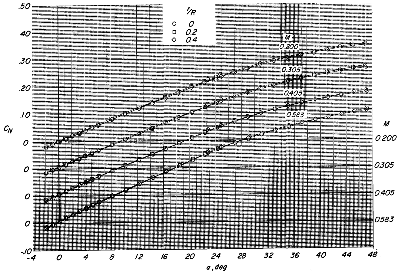
(a) Variation of C_N with \alpha .
