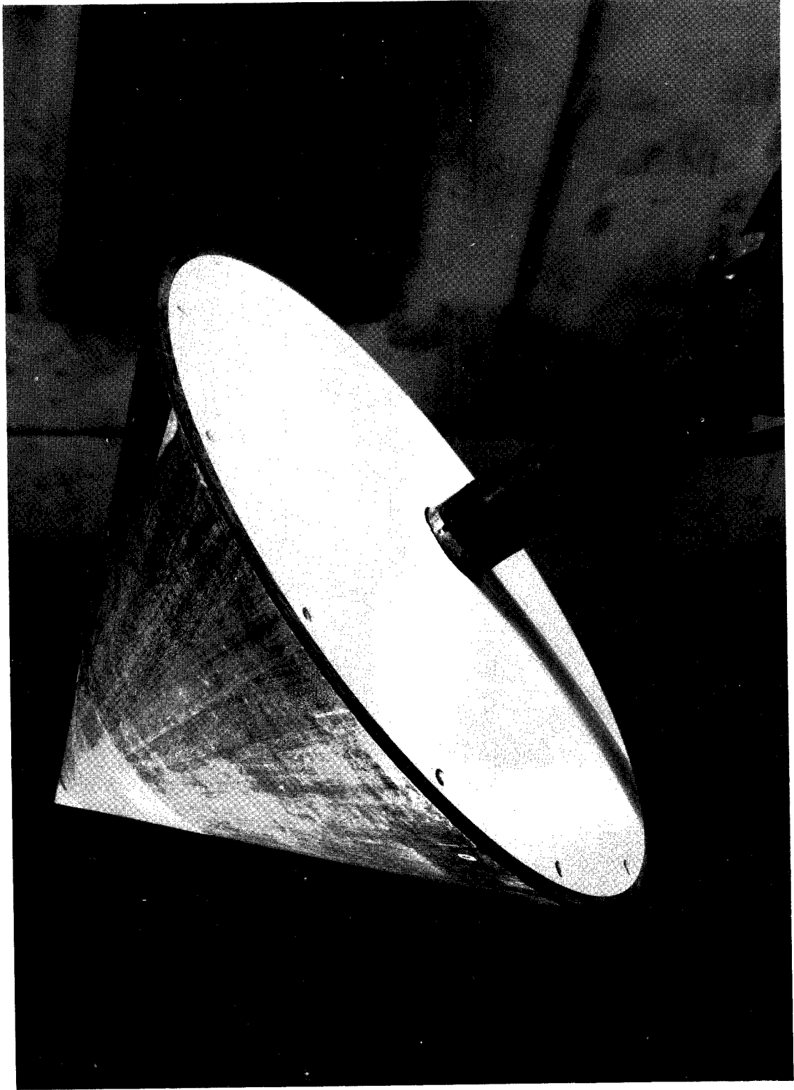
Figure 2.- Three-quarter side view of 80° cone model having r/R = 0 .
