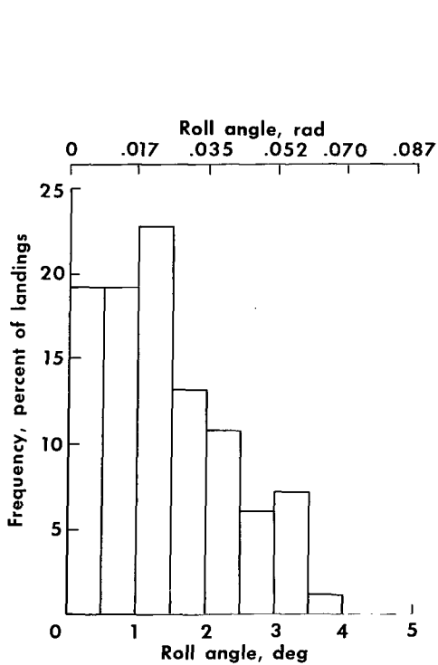
Figure 12.— Histogram of absolute roll angle at touchdown.
