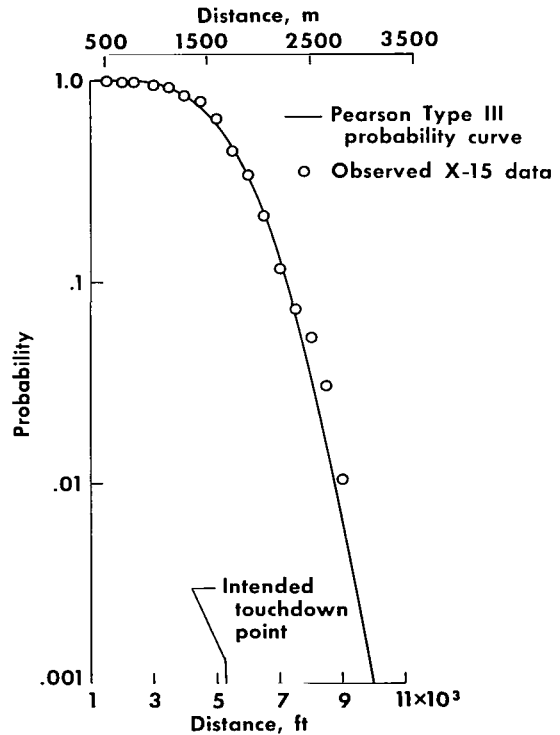
Figure 15.—Probability of equaling or exceeding various values of distance to touchdown point from 1-mile marker.
