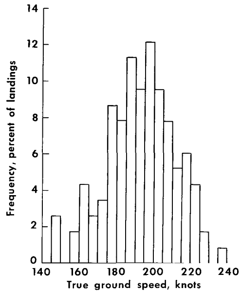
Figure 8.— Histogram of true ground speed at contact.
