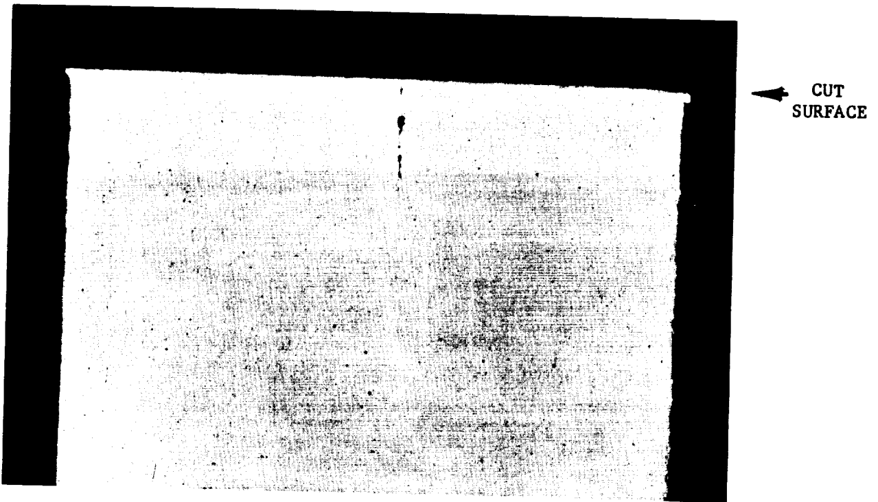
FIGURE 43. CROSS-SECTION OF SURFACE CUT DRY ON ABRASIVE WHEEL. FEED RATE 4.0 IPM AT 8,240 SFM
