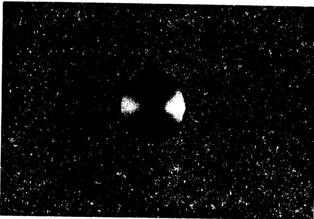
FIGURE 27. CORRECTLY DRILLED HOLE USING RECOMMENDED PROCEDURES. EXIT SIDE (UNETCHED)
