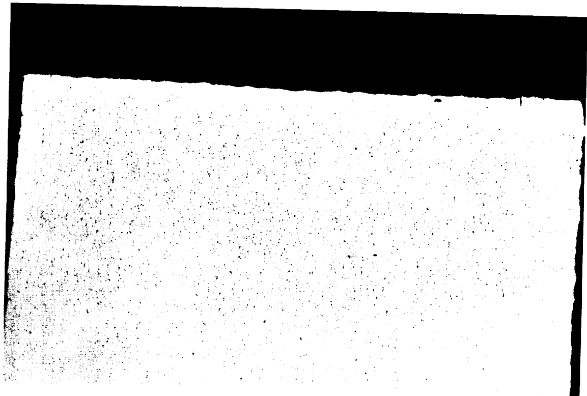
FIGURE 68. CROSS-SECTION OF EDM FINISH CUT AT 130,000 CPS. METAL REMOVAL RATE 0.125 CU. IN./HR.
