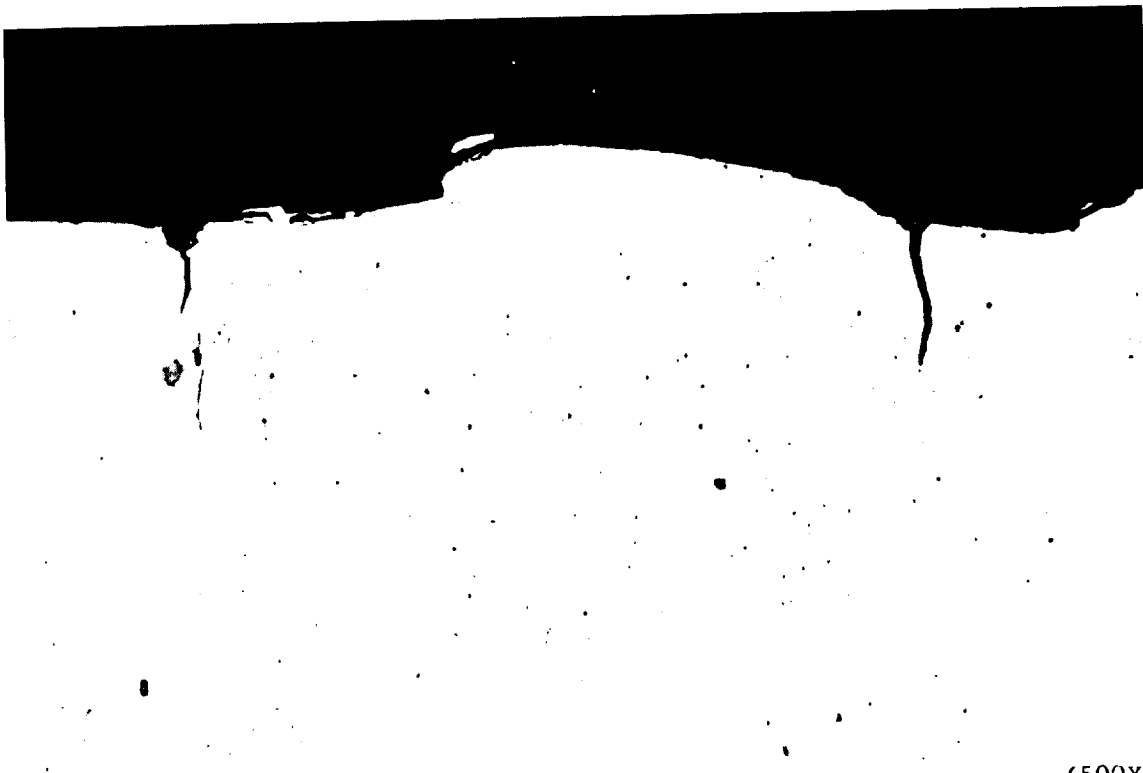
FIGURE 63. CROSS-SECTION OF EDM FINISH CUT AT 2,000 CPS. METAL REMOVAL RATE 1.140 CU. IN./HR.
