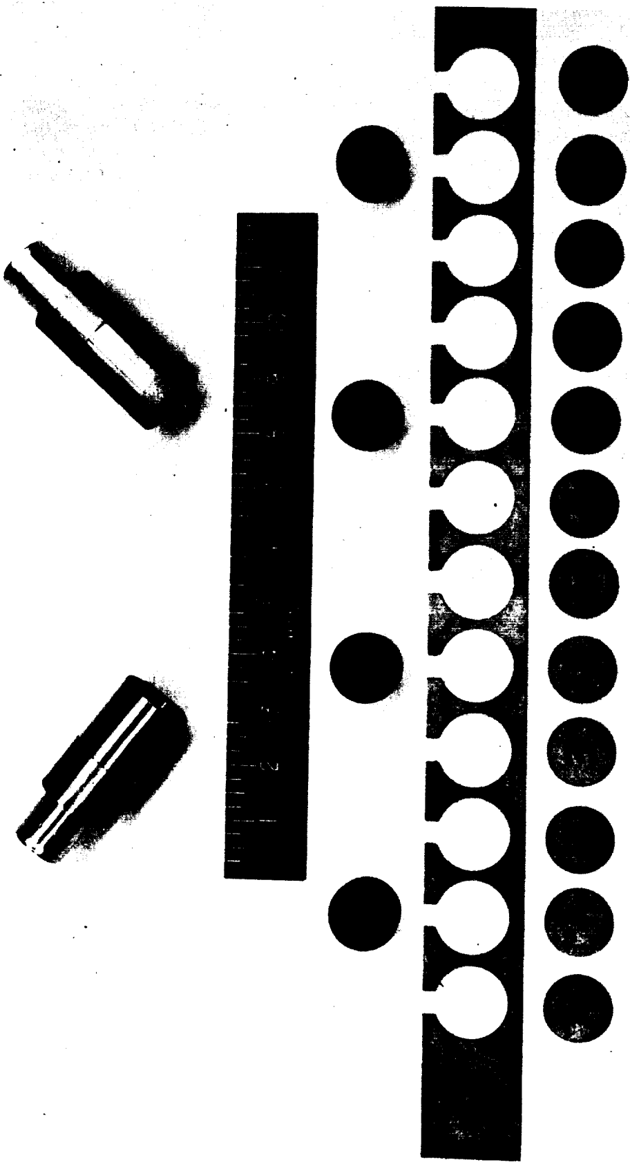
FIGURE 59. TEST COUPONS AND EDM ELECTRODES. ROUGHING ELECTRODE ON RIGHT AND FINISH ELECTRODE ON LEFT
