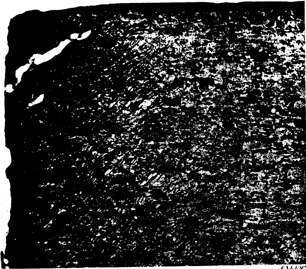
FIGURE 9. CROSS-SECTION THROUGH PUNCHED HOLE SHOWING EXTENT OF SURFACE DAMAGE AND TWINNING
