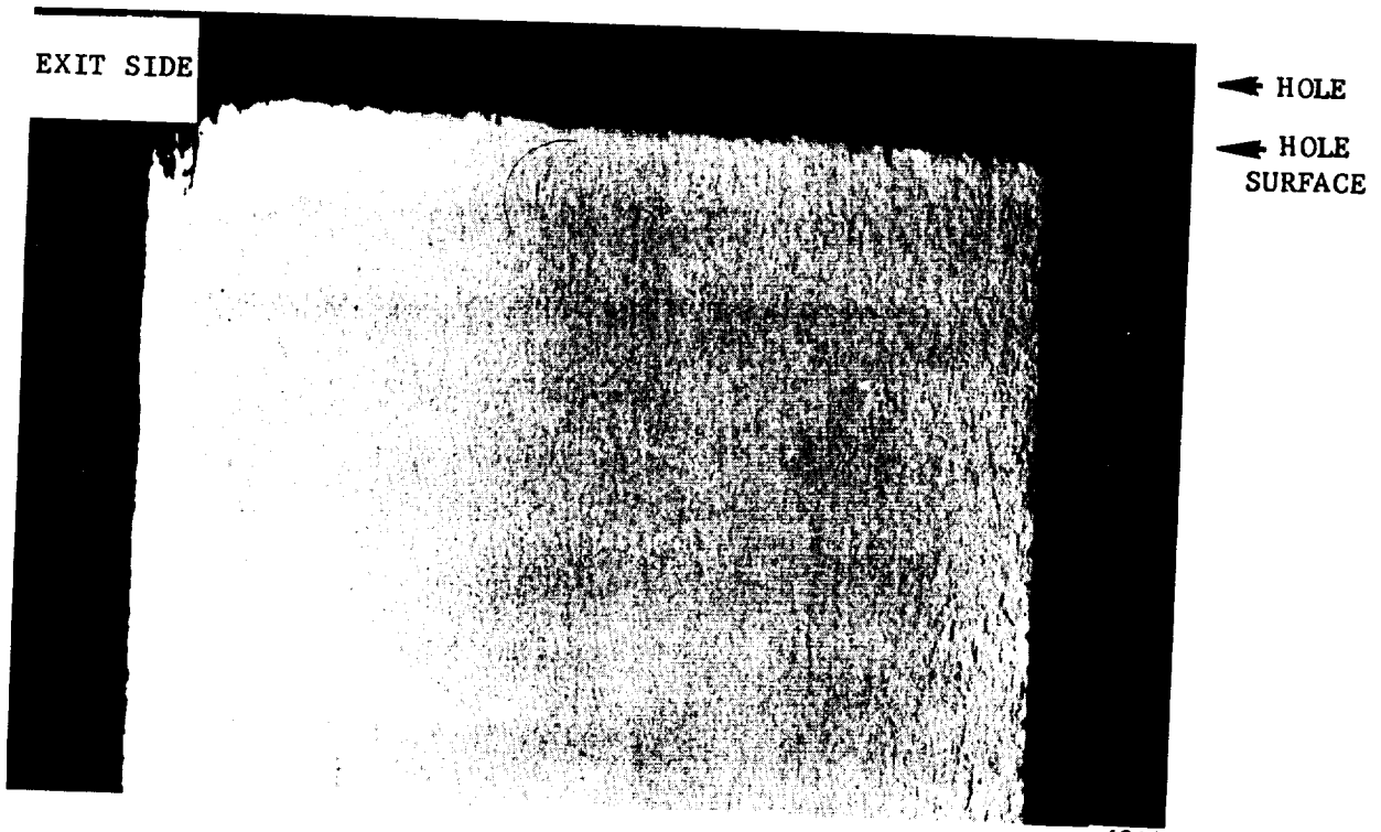
FIGURE 34. CROSS-SECTION OF HOLE DRILLED WITH DULL DRILL (UNETCHED)
