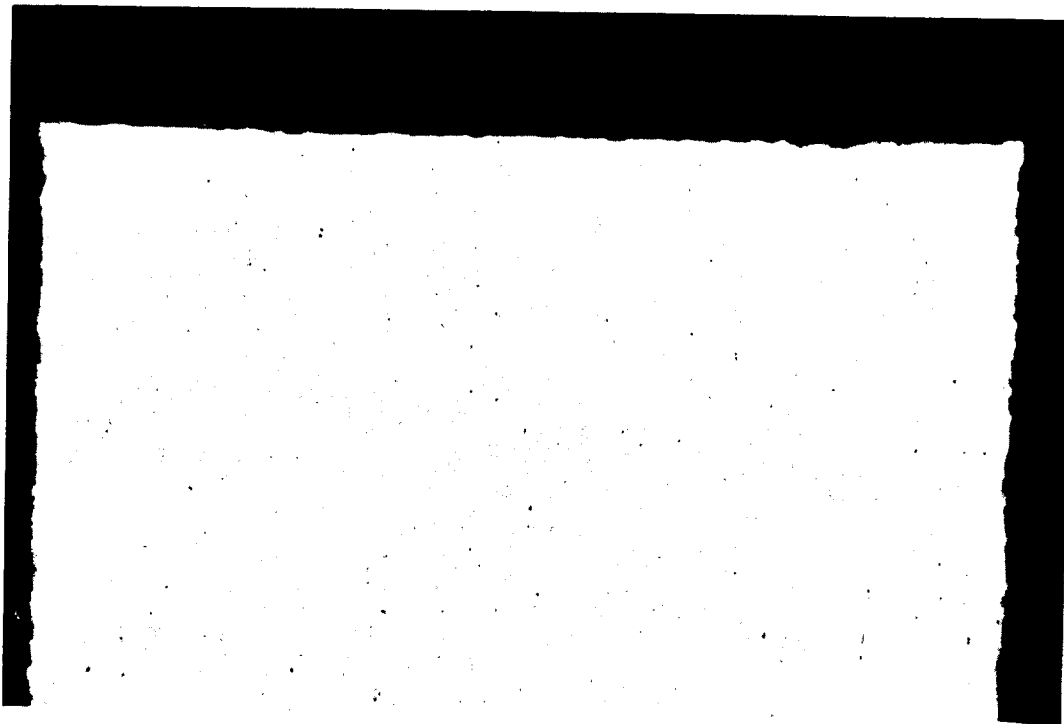
FIGURE 28. CROSS-SECTION THROUGH GOOD HOLE USING RECOMMENDED PROCEDURES (UNETCHED)
