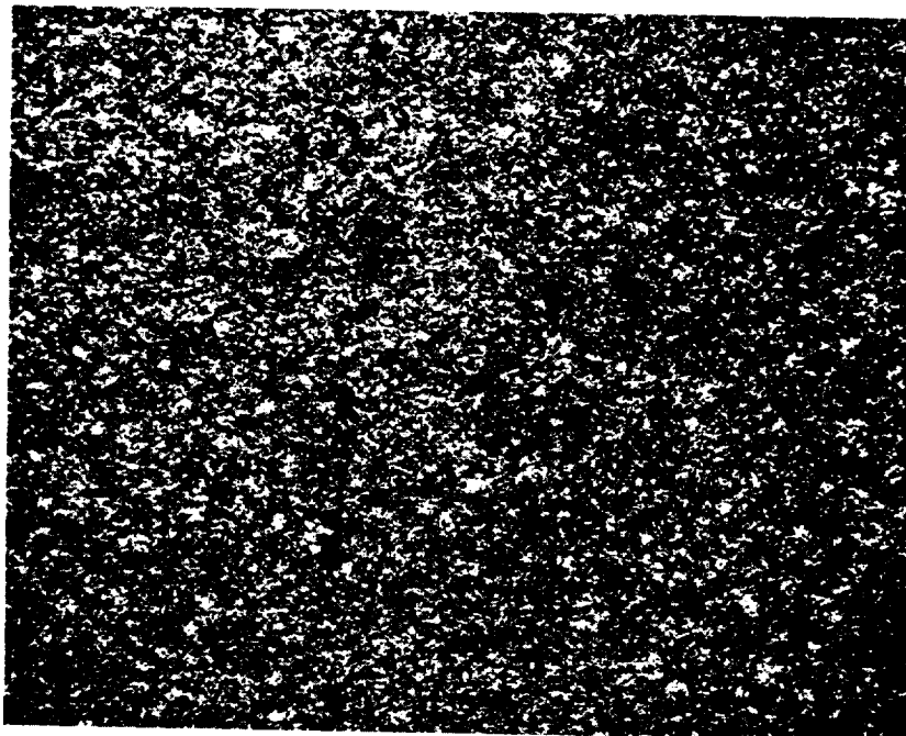
FIGURE 78. MACROPHOTOGRAPH OF AREA CHEMICALLY MILLED WITH A 7.5% SOLUTION OF SULFURIC ACID (SPECIMEN NO. 16)
