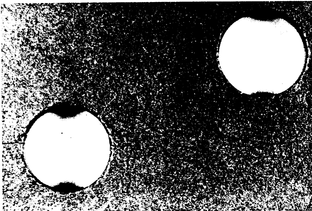
FIGURE 31. HOLE DRILLED WITH DULL DRILL SHOWING RADIAL CRACKING AND BRIDGING FROM HOLE TO HOLE
