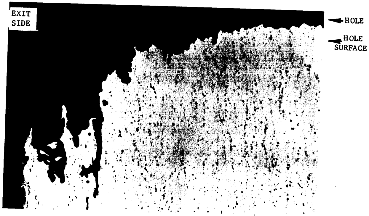
FIGURE 35. CROSS-SECTION OF HOLE DRILLED WITH DULL DRILL SHOWING SPALLED EDGE (UNETCHED)
