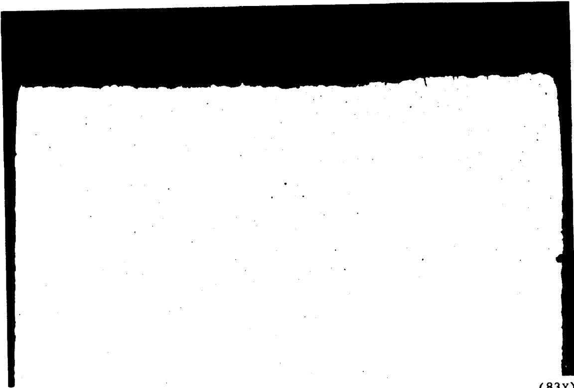
FIGURE 66. CROSS-SECTION OF EDM FINISH CUT AT 130,000 CPS. METAL REMOVAL RATE 0.285 CU. IN./HR.
