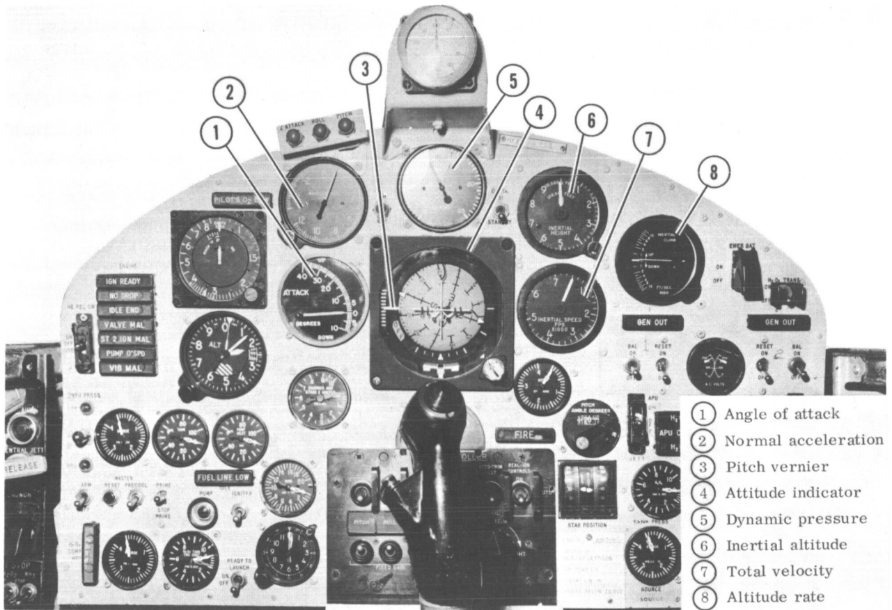
Figure 2.— Operational instrument panel.
