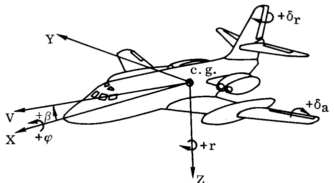
Figure 1.— Body-axis system and sign conventions.
