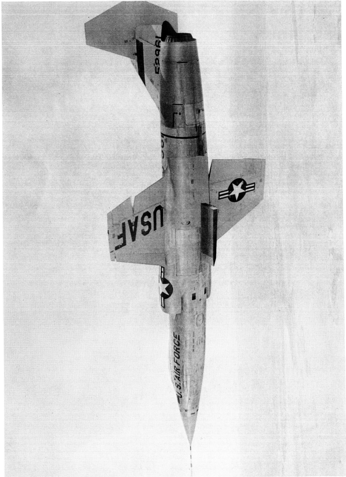
Figure 1. — F-104 airplane with flight-test fixture installed.
