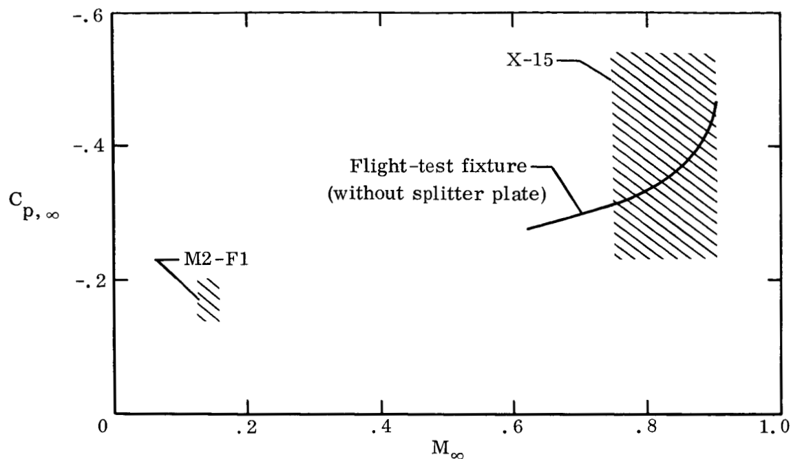
Figure 7. - Comparison of base pressure coefficients from the flight-test fixture with flight results from fins and fin-like projections of two aircraft. Turbulent flow.
