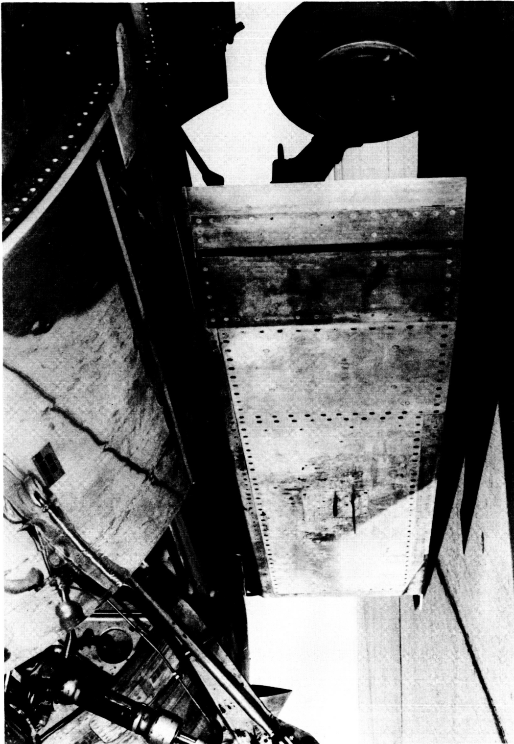
(a) View from 2 o'clock position. (Vertical strip behind leading edge is boundary-layer trip.)
