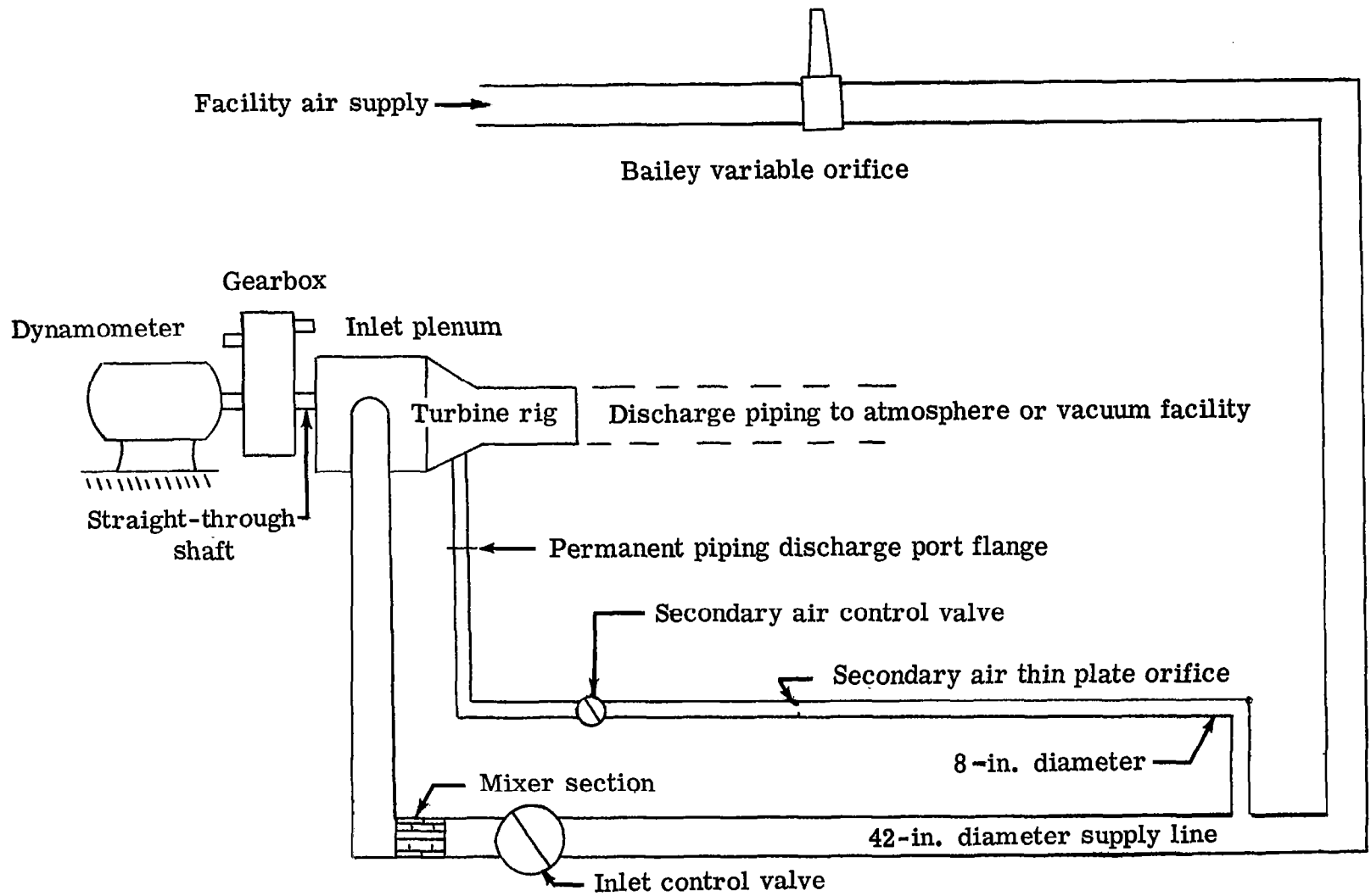
Figure 75. Schematic of test stand air supply system.
