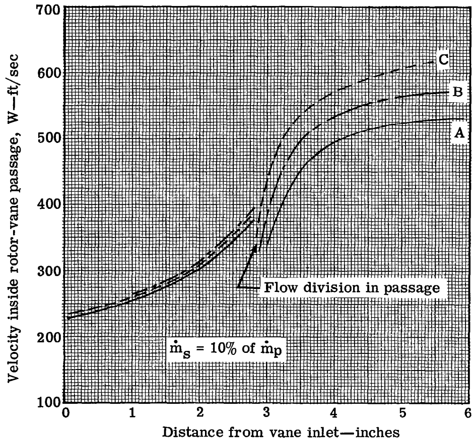
Figure 21. Velocity distribution inside rotor-vane based on P_{T_I}/\delta_0 = 14.7 psia and T_{T_I}/\sqrt{\theta_{cr}} = 518.7^\circ\text{R} .
