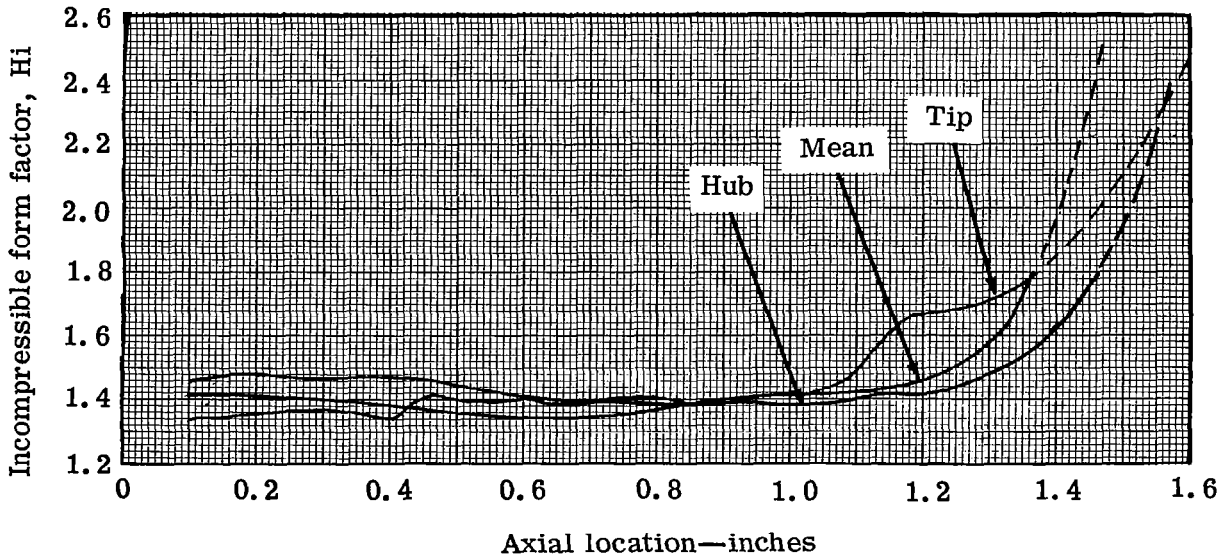
Figure 12. Plain rotor-blade suction surface incompressible form factor.
