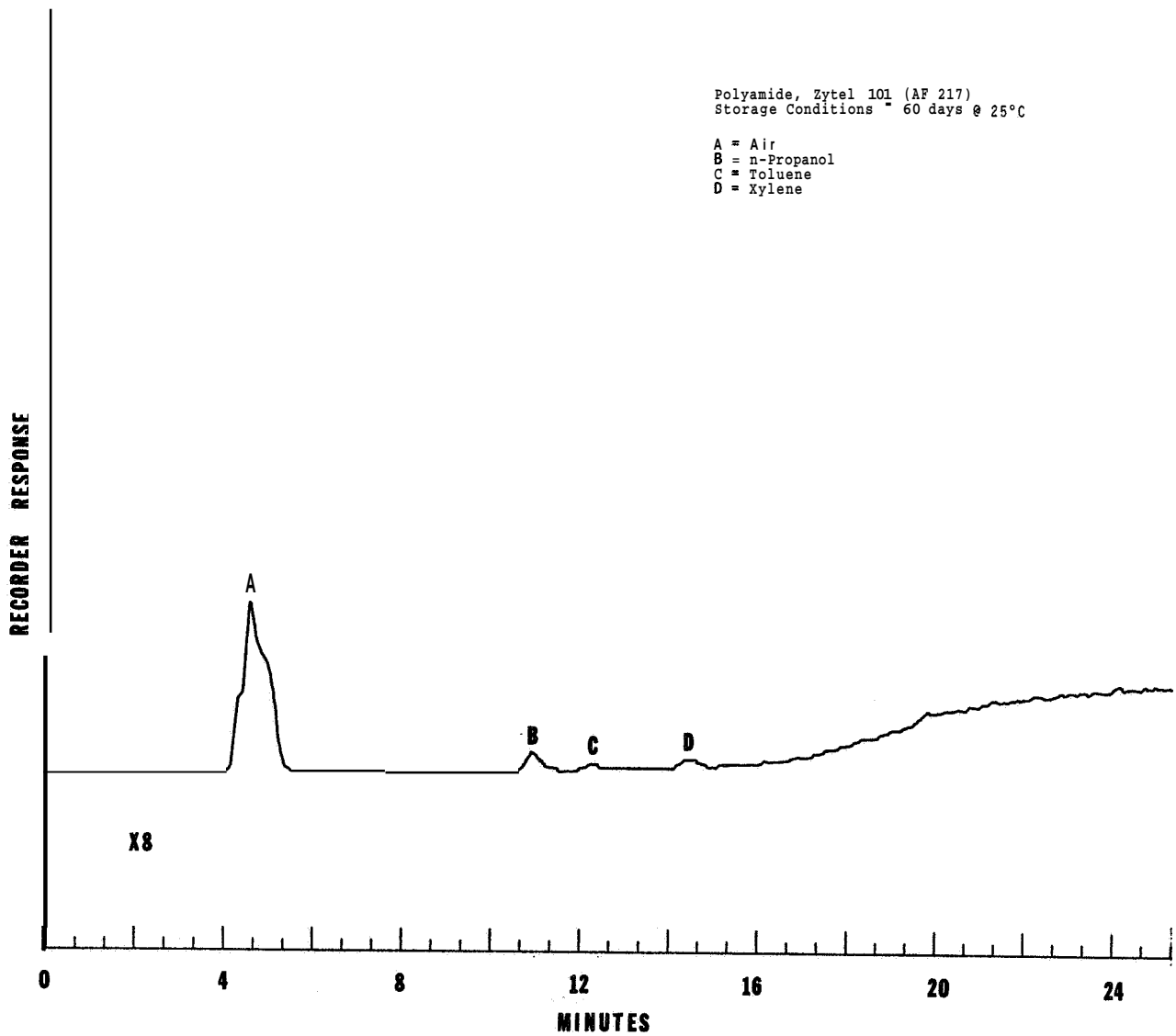
Figure 63. Gas Chromatogram of Gas-Off Products from Polyamide, Zytel 101 (AF 217) (60 days @ 25°C).
