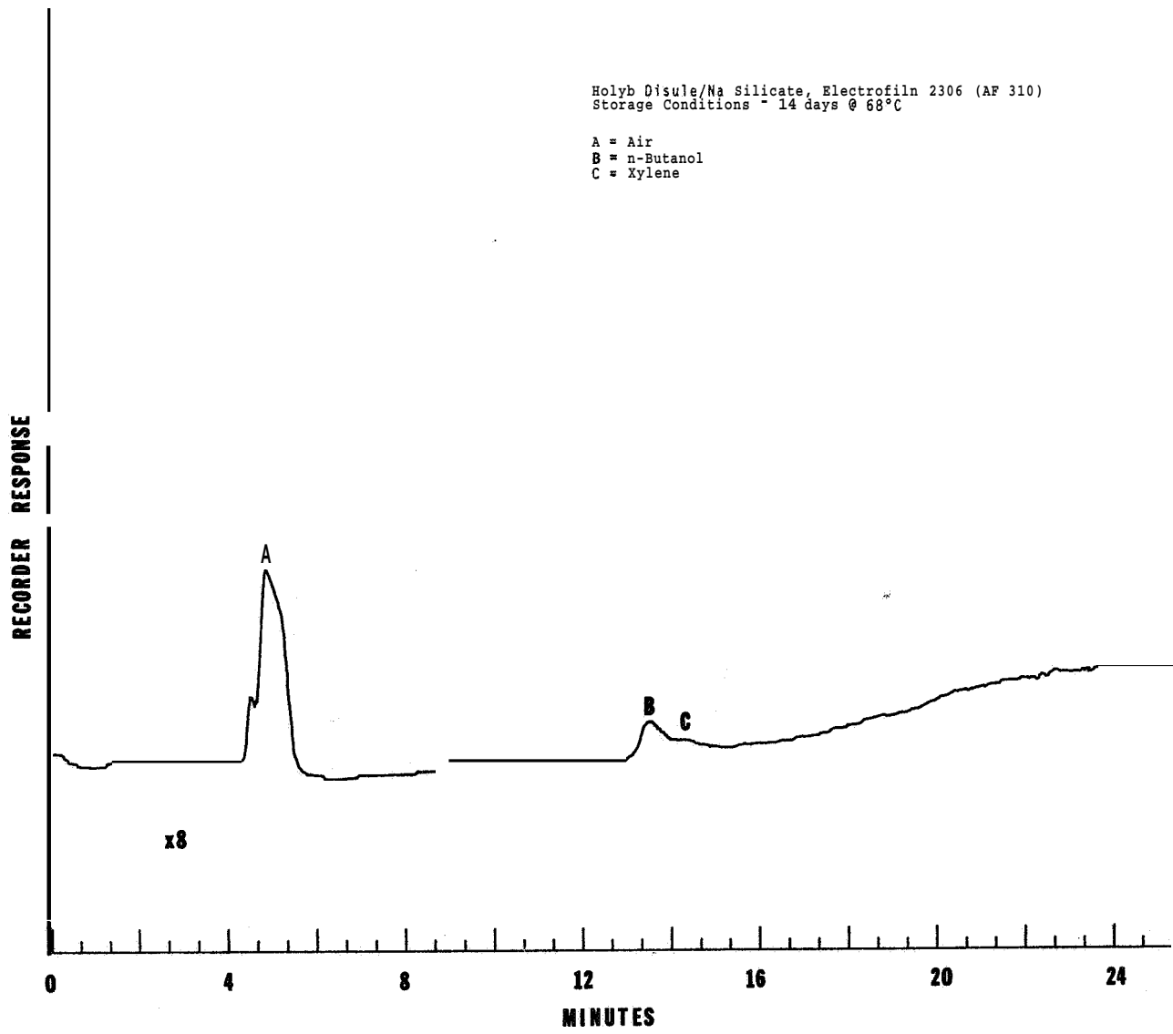
Figure 76. Gas Chromatogram of Gas-Off Products from Molyb Disulfide/Na Silicate, Electrofilm 2306 (AF 310) (14 days @ 68°C).
