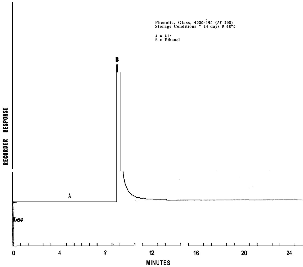
Figure 60. Gas Chromatogram of Gas-Off Products from Phenolic, Glass, 4030-190 (AF 208) (14 days @ 68°C).
