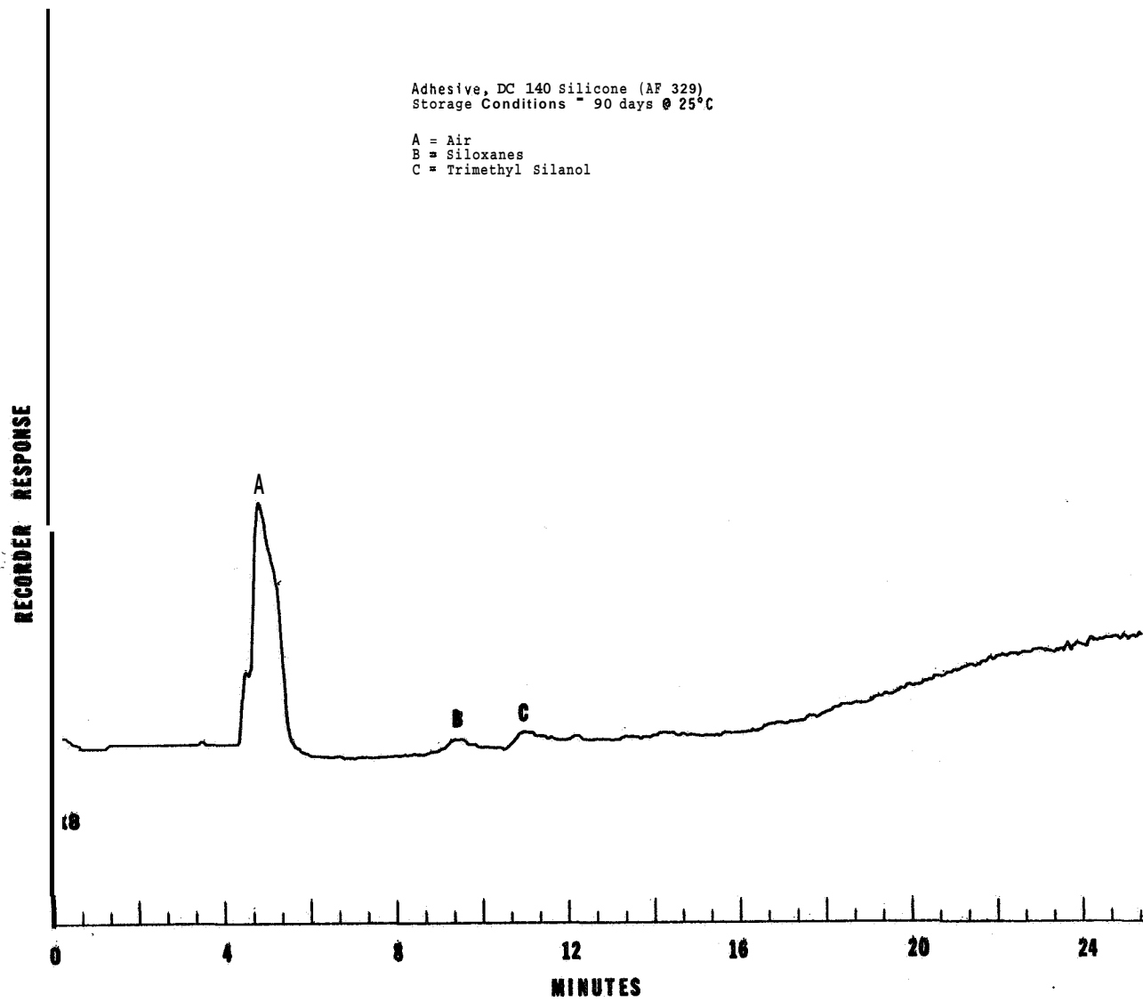
Figure 82. Gas Chromatogram of Gas- Off Products from Adhesive, DC 140 Silicone (AF 329) (90 days @ 25°C).
