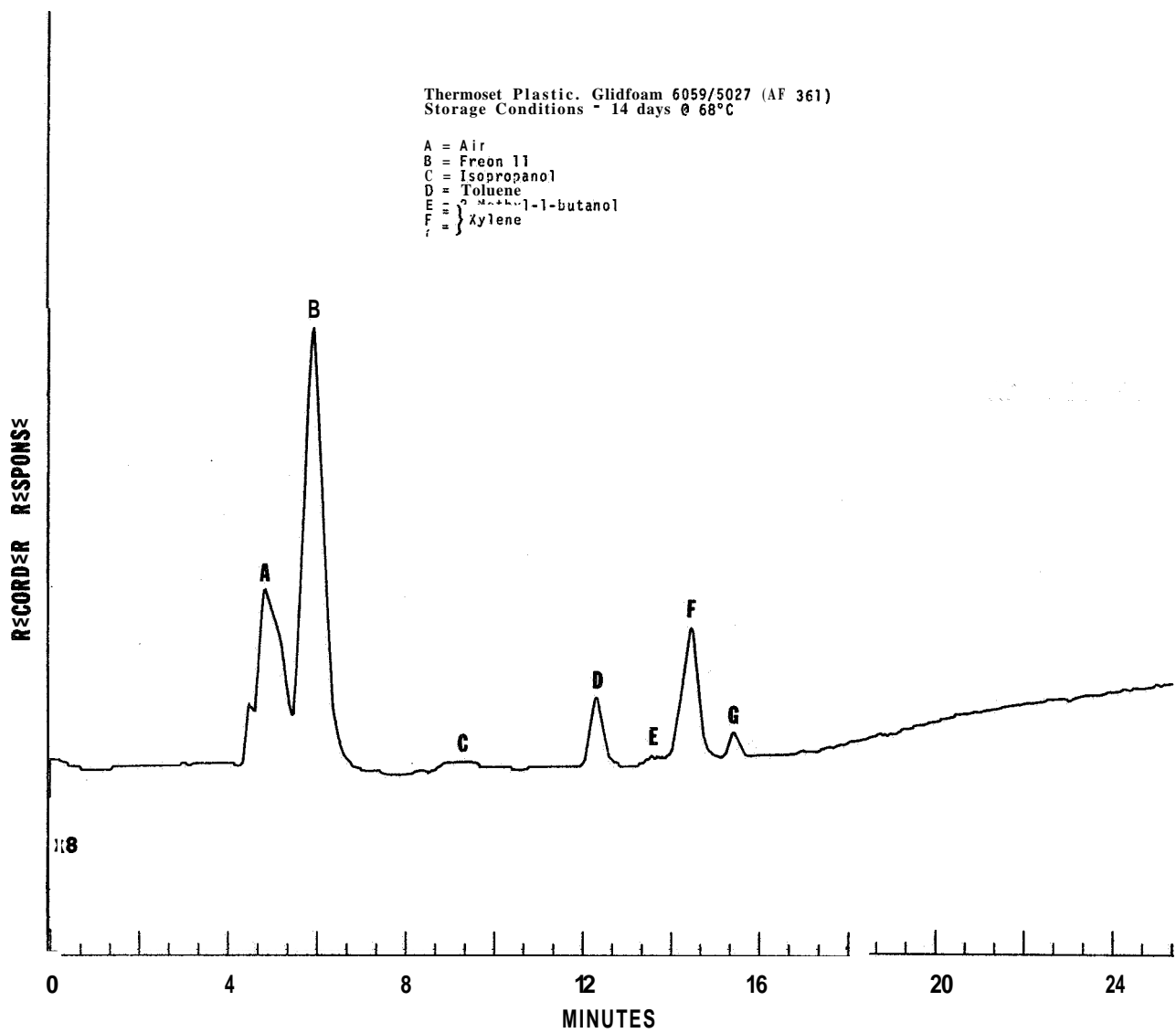
Figure 87. Gas Chromatogram of Gas-Off Products from Thermoset Plastic, Glidfoam 6059/5027 (AF 361) (14 days @ 68°C).
