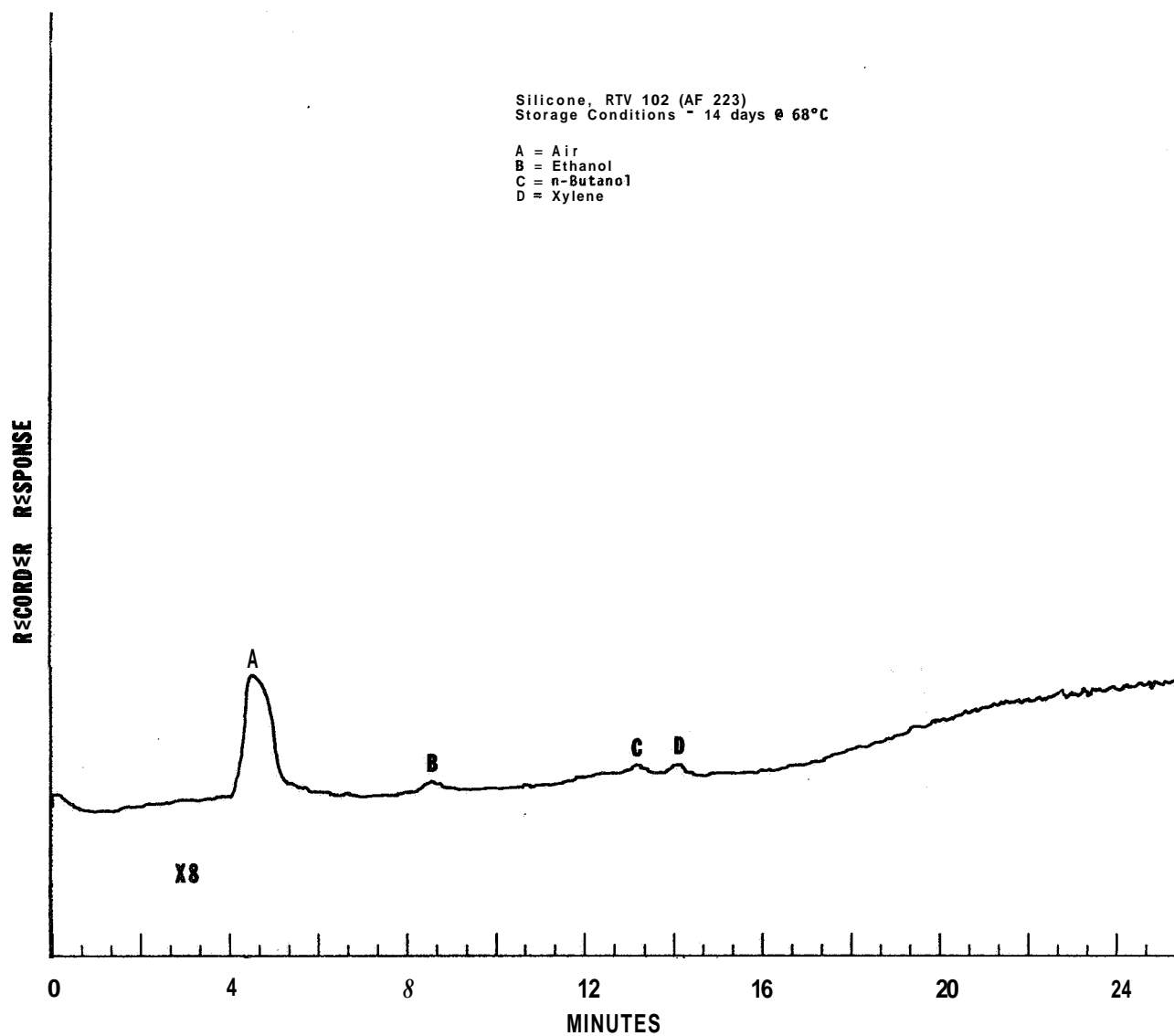
Figure 65. Gas Chromatogram of Gas-Off Products from Silicone, RTV 102 (AF 223) (14 days @ 68°C).
