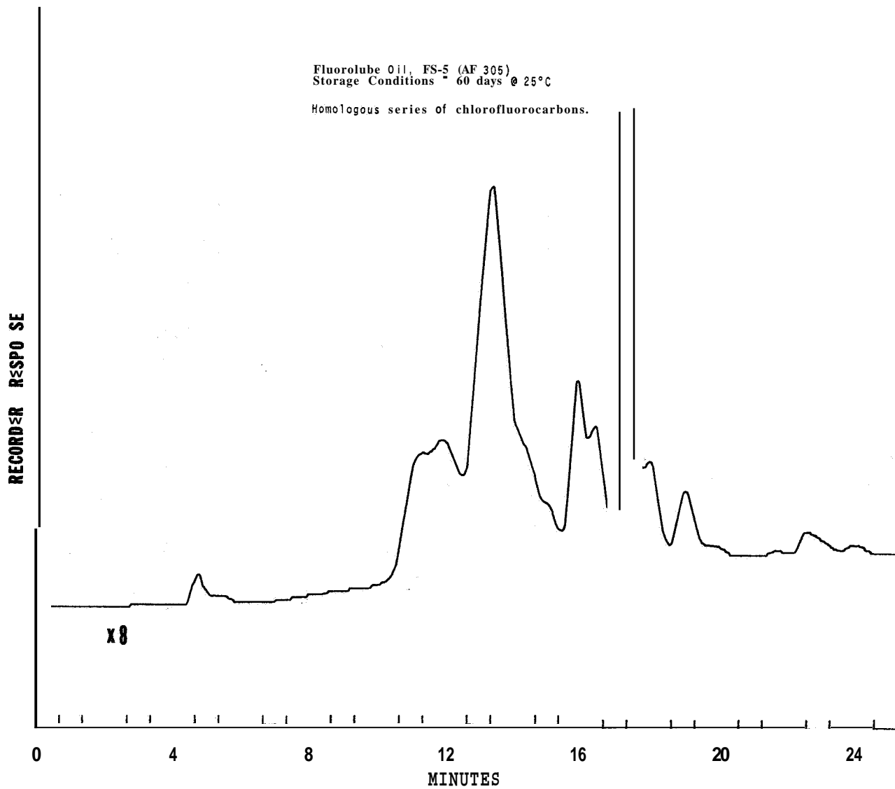
Figure 73. Gas Chromatogram of Gas-Off Products from Fluorolube Oil, FS-5 (AF 305) (60 days @ 25°C).
