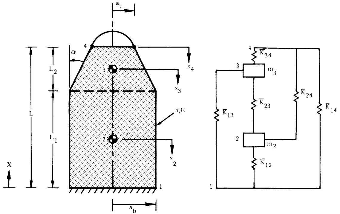
Figure 19. Two-Mass Cone-Cylinder Model
