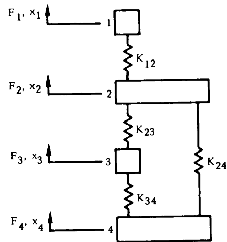
Figure 25. Spring-Mass Model
