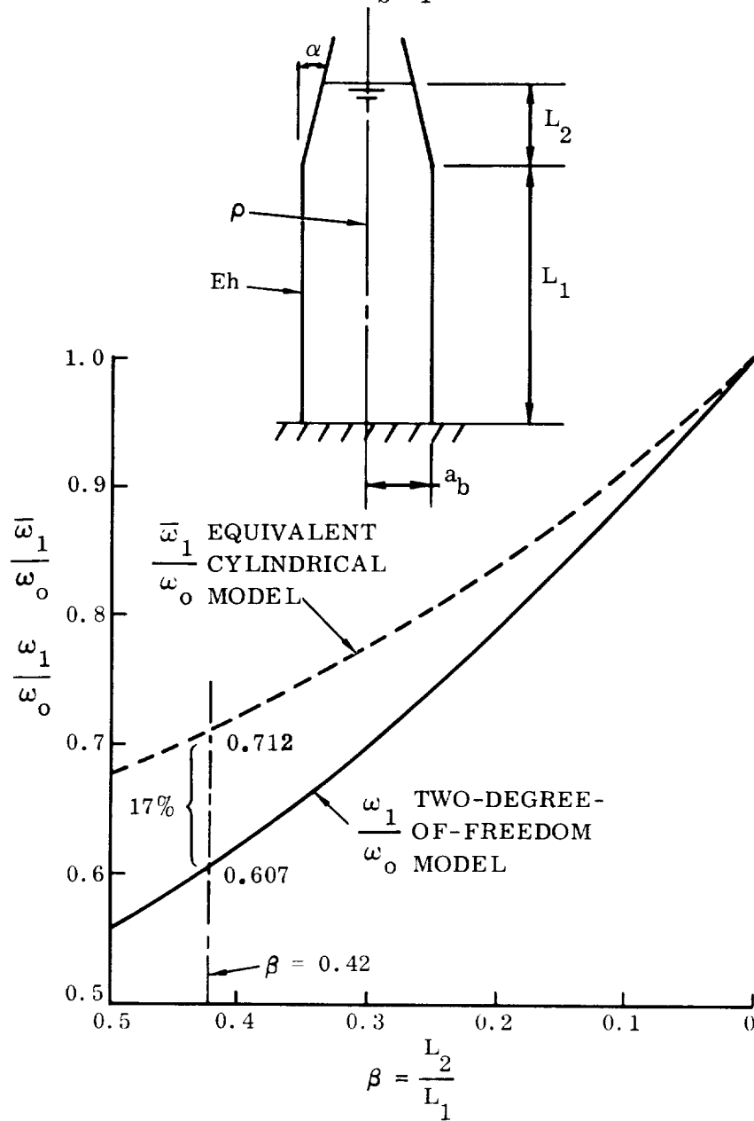
Figure 21. Natural Frequency of Cone-Cylinder Tank
