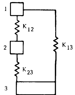
Figure 26. Model Corresponding to Stiffness Matrix
