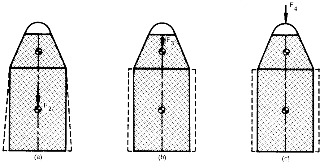
Figure 20. Radial Deformations in Two-Mass Cone-Cylinder Model
