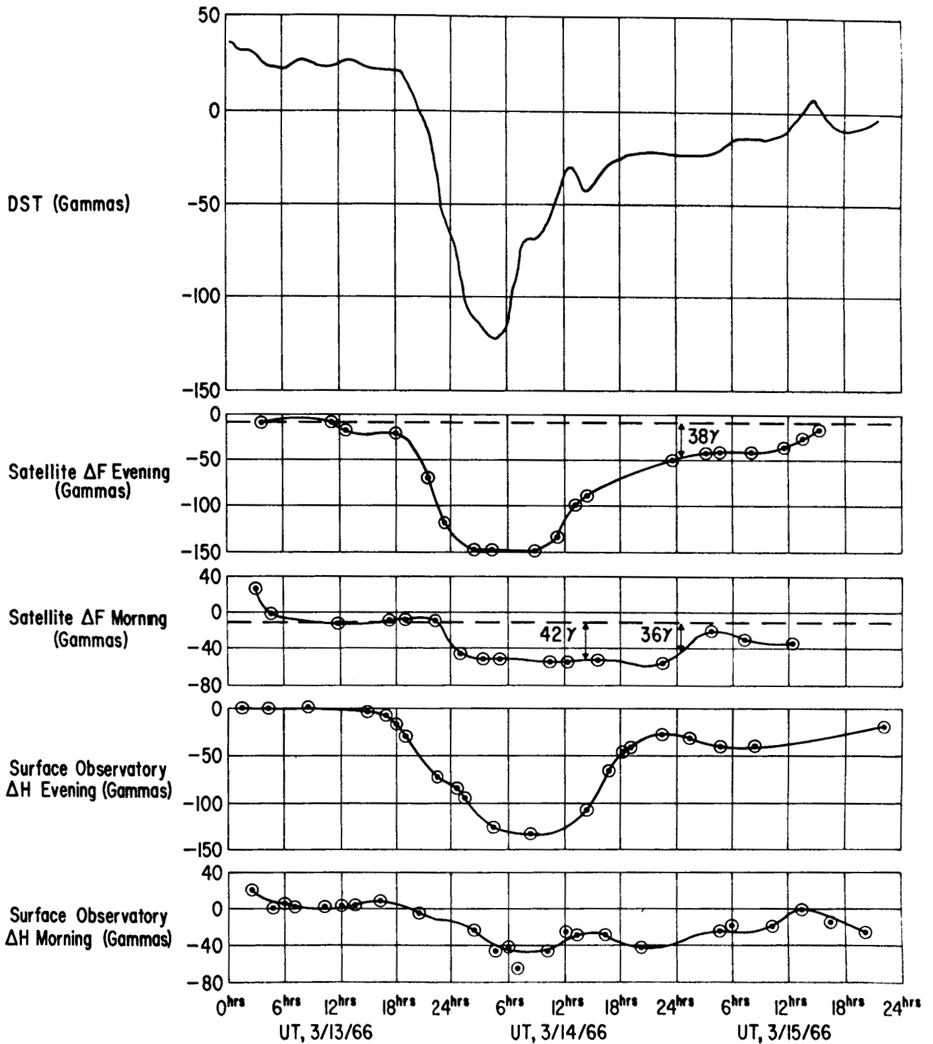
FIGURE 9: Comparison of Dst, Satellite and Surface Observatory Data. The satellite data are the points of maximum deviation between +30° and -30° latitude. The morning satellite data is 0440 local time and the evening is at 1630 local time. The observatory data are the 0600 and 1800 local time values of D(H) at seven low latitude observatories.
