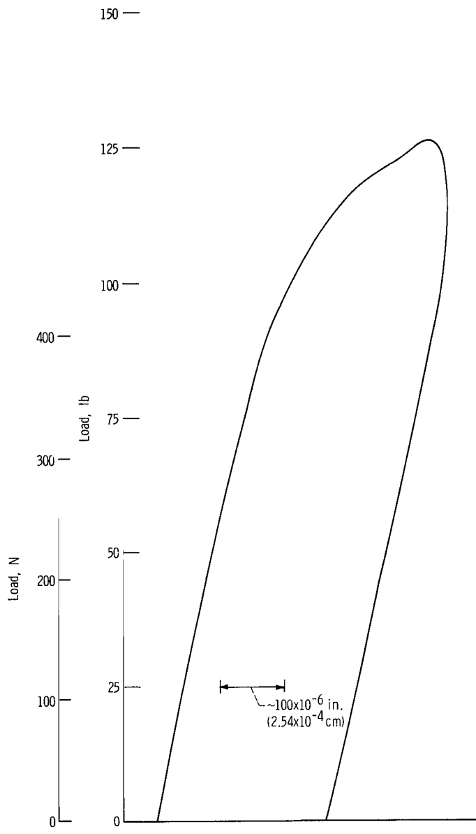
(a) Measured by capacitance gauge.
