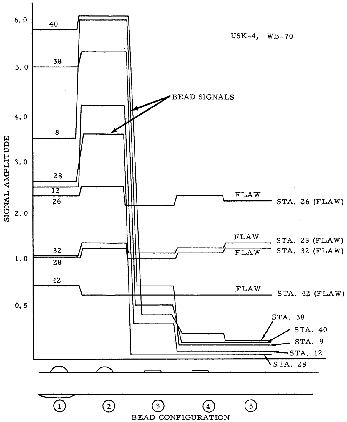
Figure B-1. Weld Bead Interference - 0.80 Inch Weld
