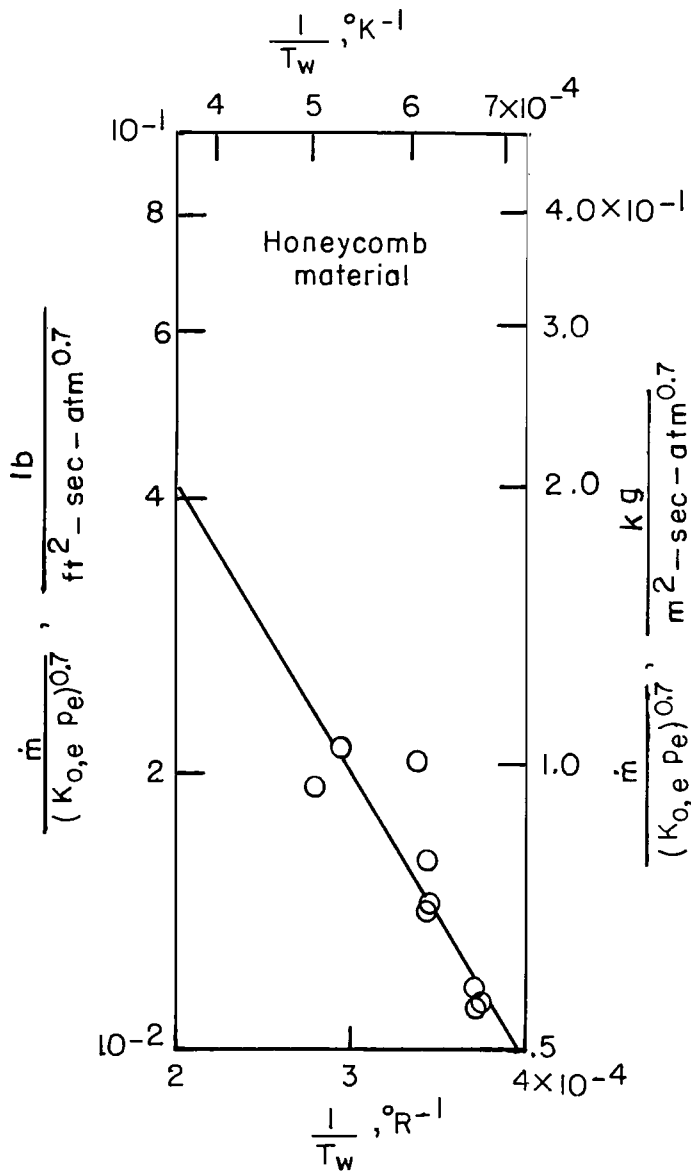
Figure 21.- Arrhenius plots of arc-jet test data for molded- and composite-ablator materials.
