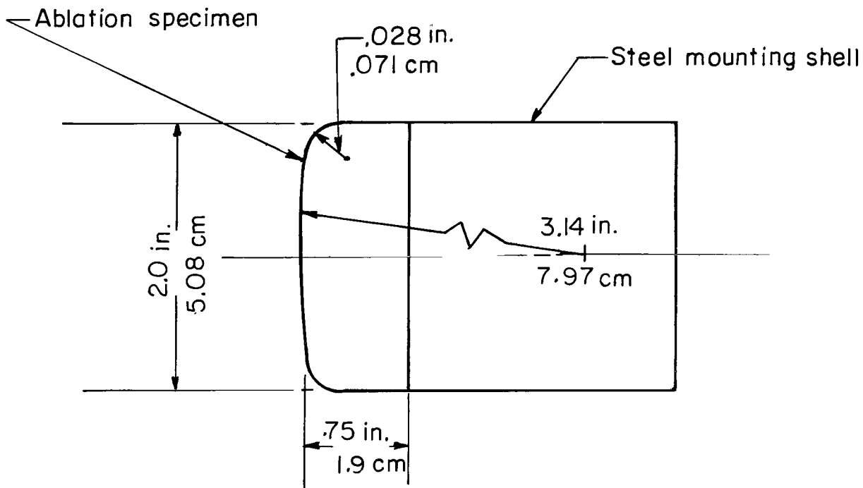
Figure 20.- Sketch of arc-jet test models.
