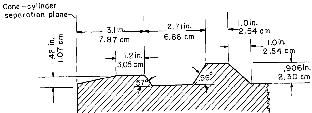
Figure 5.- Sketch of ramp-umbilical simulation on Pacemaker spacecraft.
