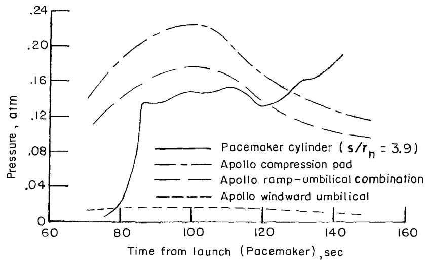
(a) Time histories of heating, shear, and pressure.
