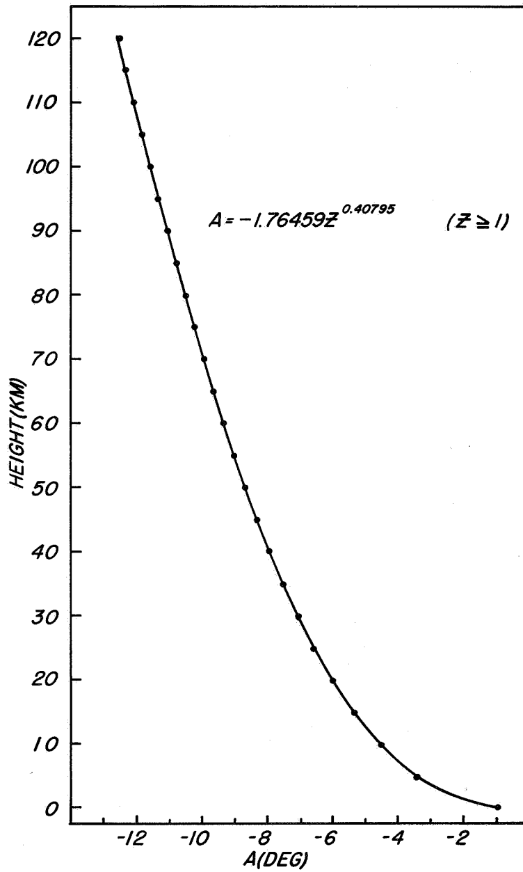
Figure 2. Variation with height of solar elevation angle, relative to the earth's surface, at sunrise and sunset. Equation was obtained by least-squares fit to points at 5-km intervals.
