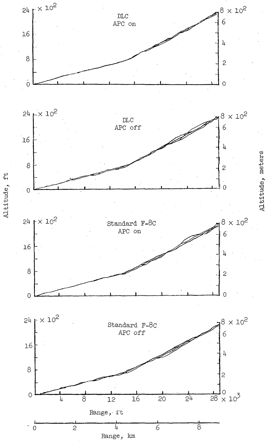
Figure 12.- Comparison of approach performance on the two-segment 60 into 30 profile for the four configurations. APC denotes autothrottle.
