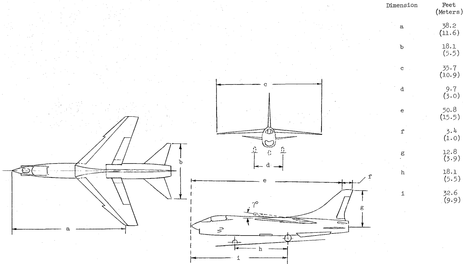
Figure 1.- Three-view sketch of test airplane.
