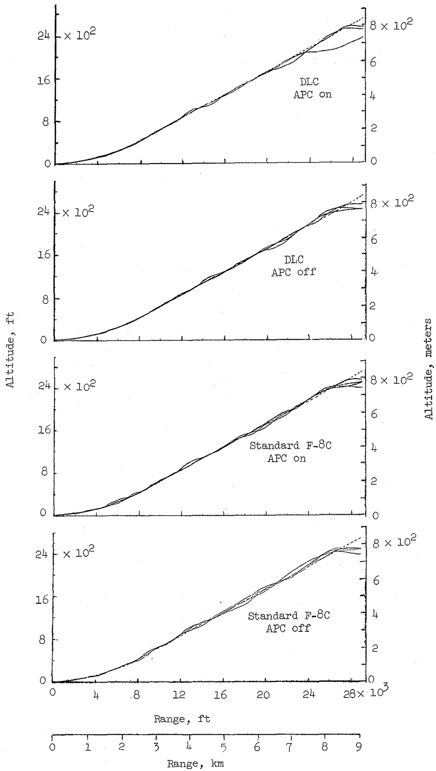
Figure 11.- Comparison of approach performance on the 6 0 single-segment profile for the four configurations. APC denotes autothrottle.
