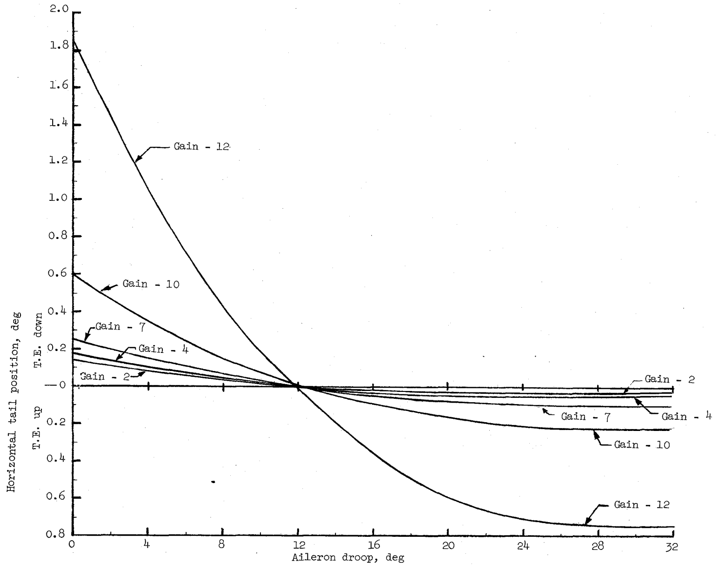
Figure 3.- Variation of horizontal-tail position with aileron droop for different interconnect gain settings.
