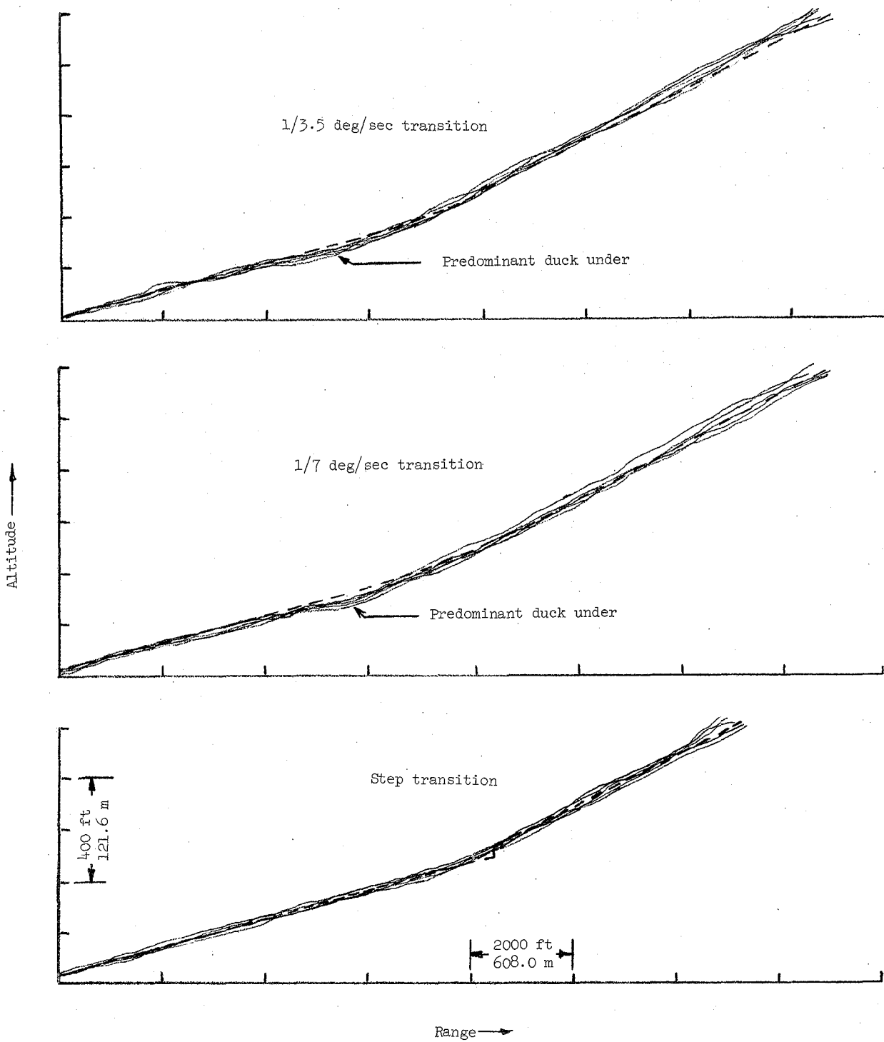
Figure 13.- Radar plots of flight-path deviations for two curved transitions and a step transition.
