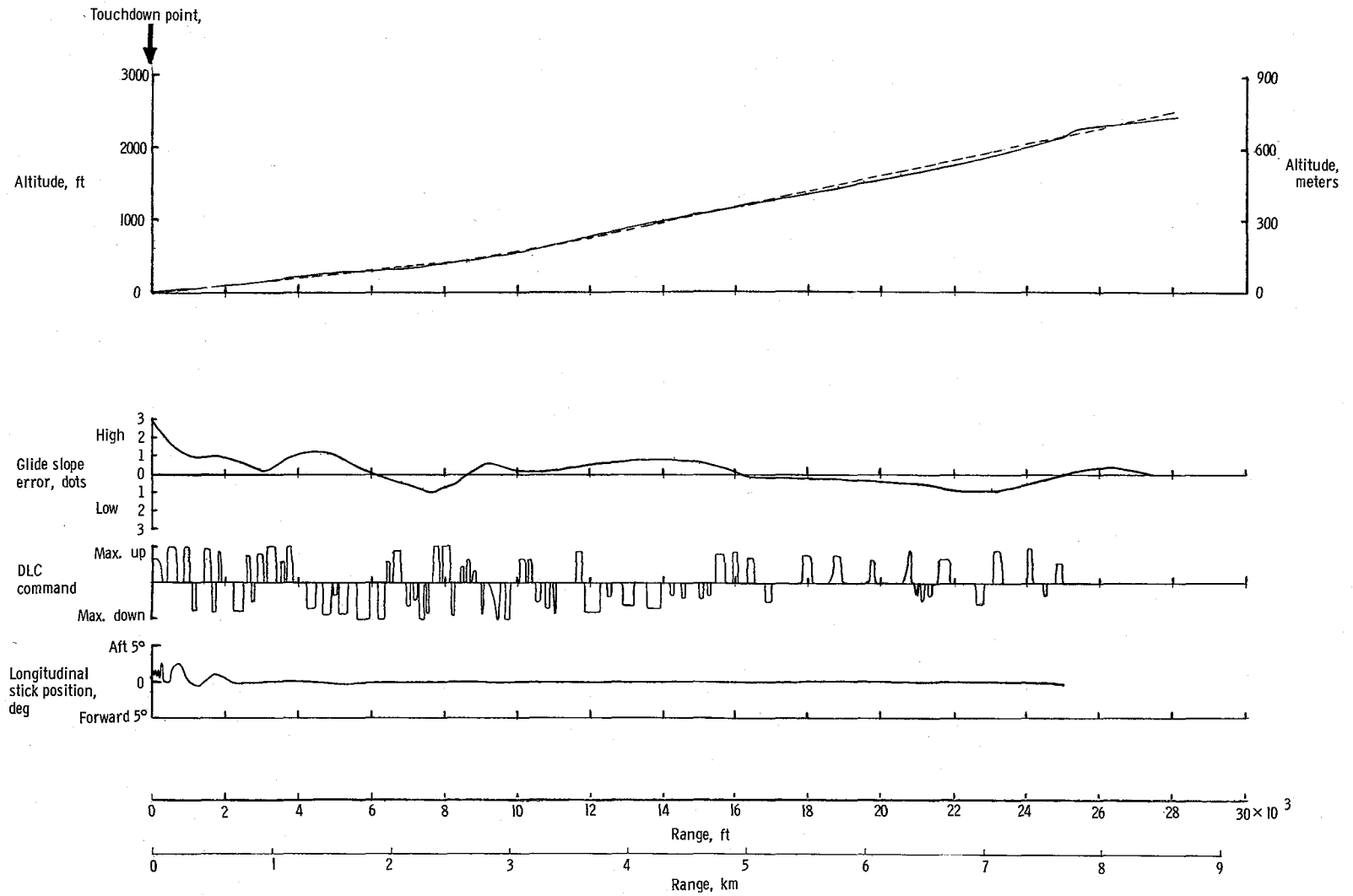
Figure 9.- Example of approach performance and longitudinal control activity with stick lock connected.
