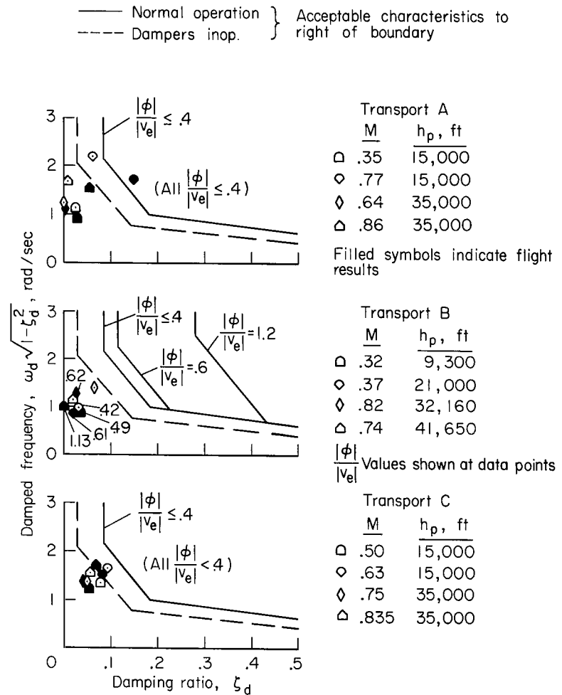
Figure 16.- Lateral oscillatory characteristics of the additional flight conditions compared with the proposed requirements of reference 6.
