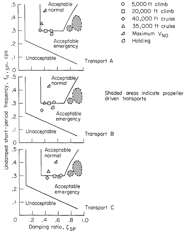
Figure 4.- Longitudinal short-period natural frequency and damping ratio compared with suggested boundaries of reference 6. Basic flight conditions.
