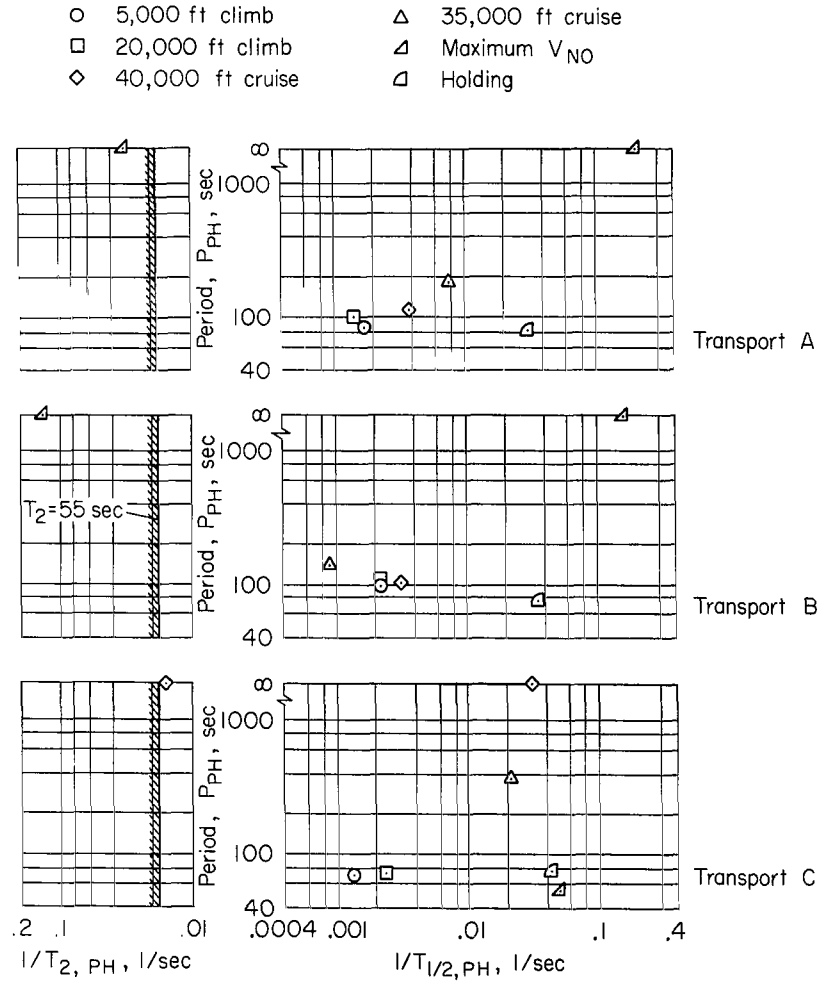
Figure 8.- Phugoid period and damping. Basic flight conditions.
