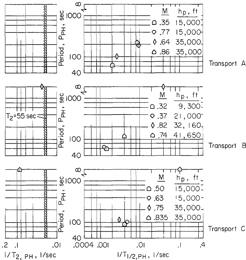
Figure 9.- Phugoid period and damping. Additional flight conditions.
