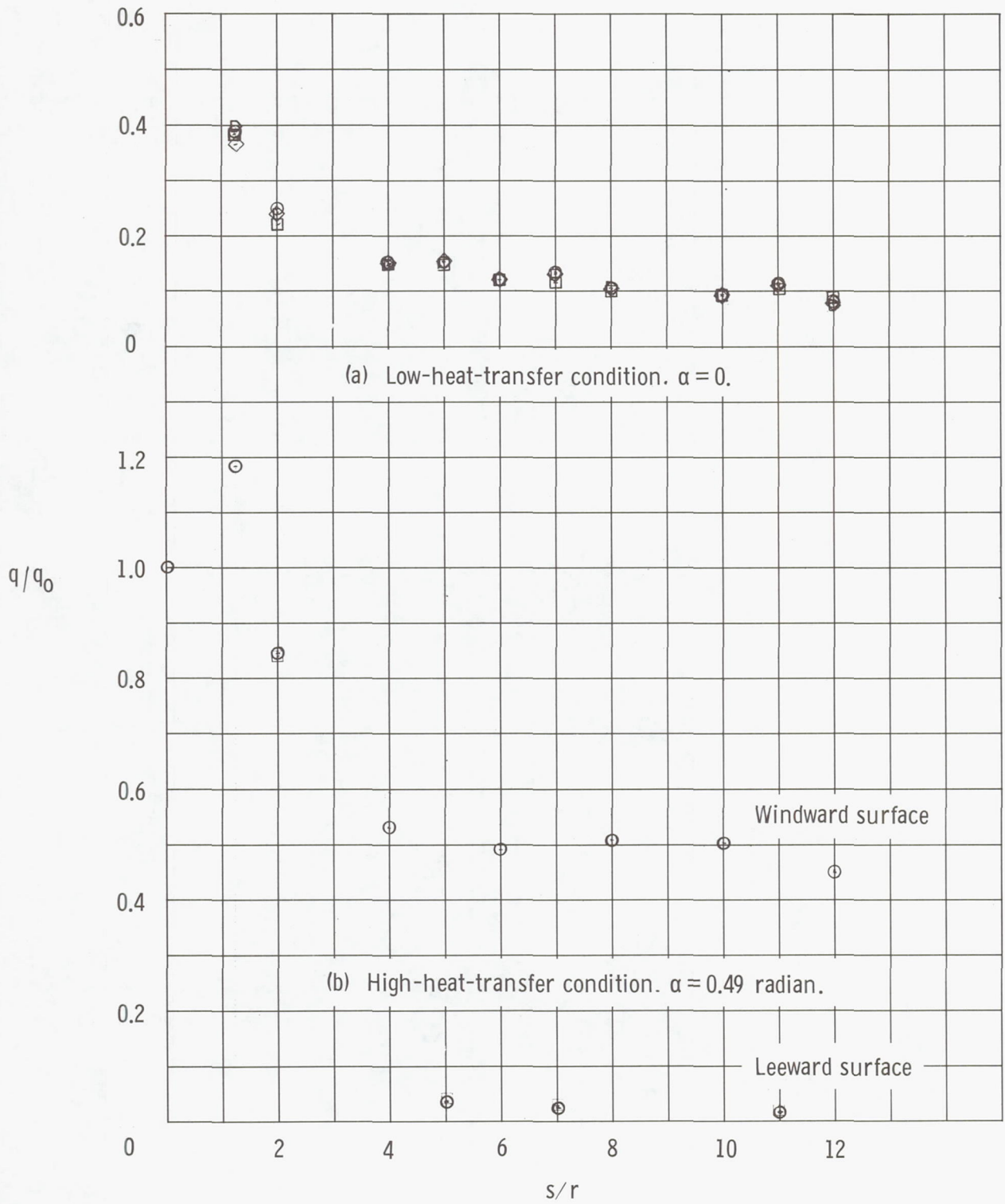
Figure 5.- Heat-transfer distribution on 0.65-radian wedge.
