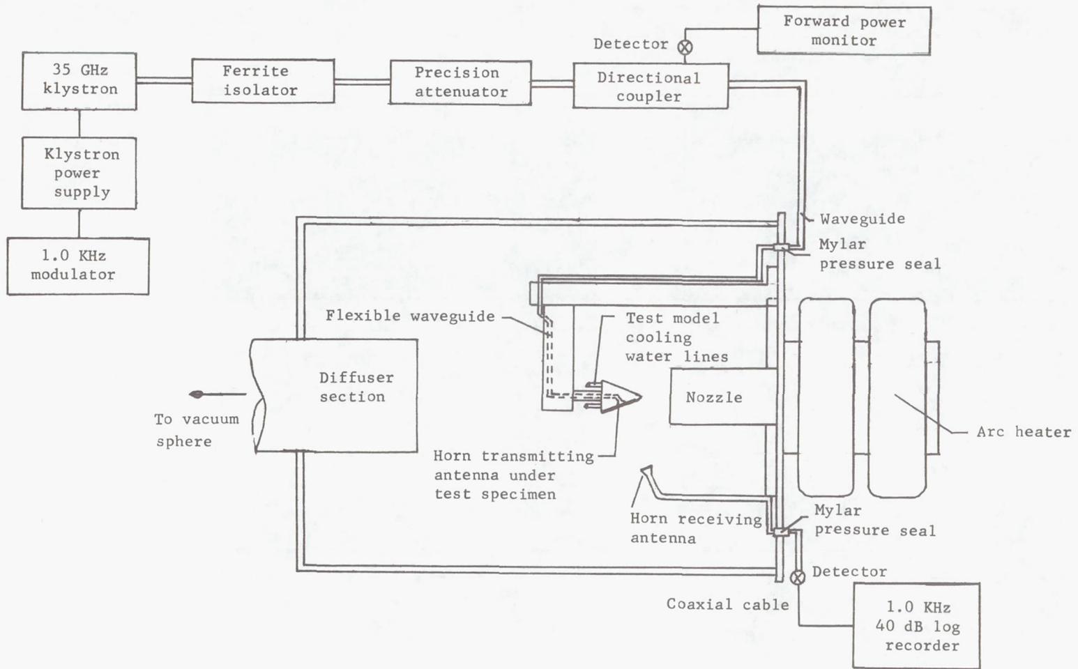
Figure 9.- Block diagram of instrumentation setup for transmission-loss measurements in arc tunnel.
