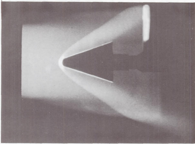
(a) Low-heat-transfer condition. \alpha = 0 .
