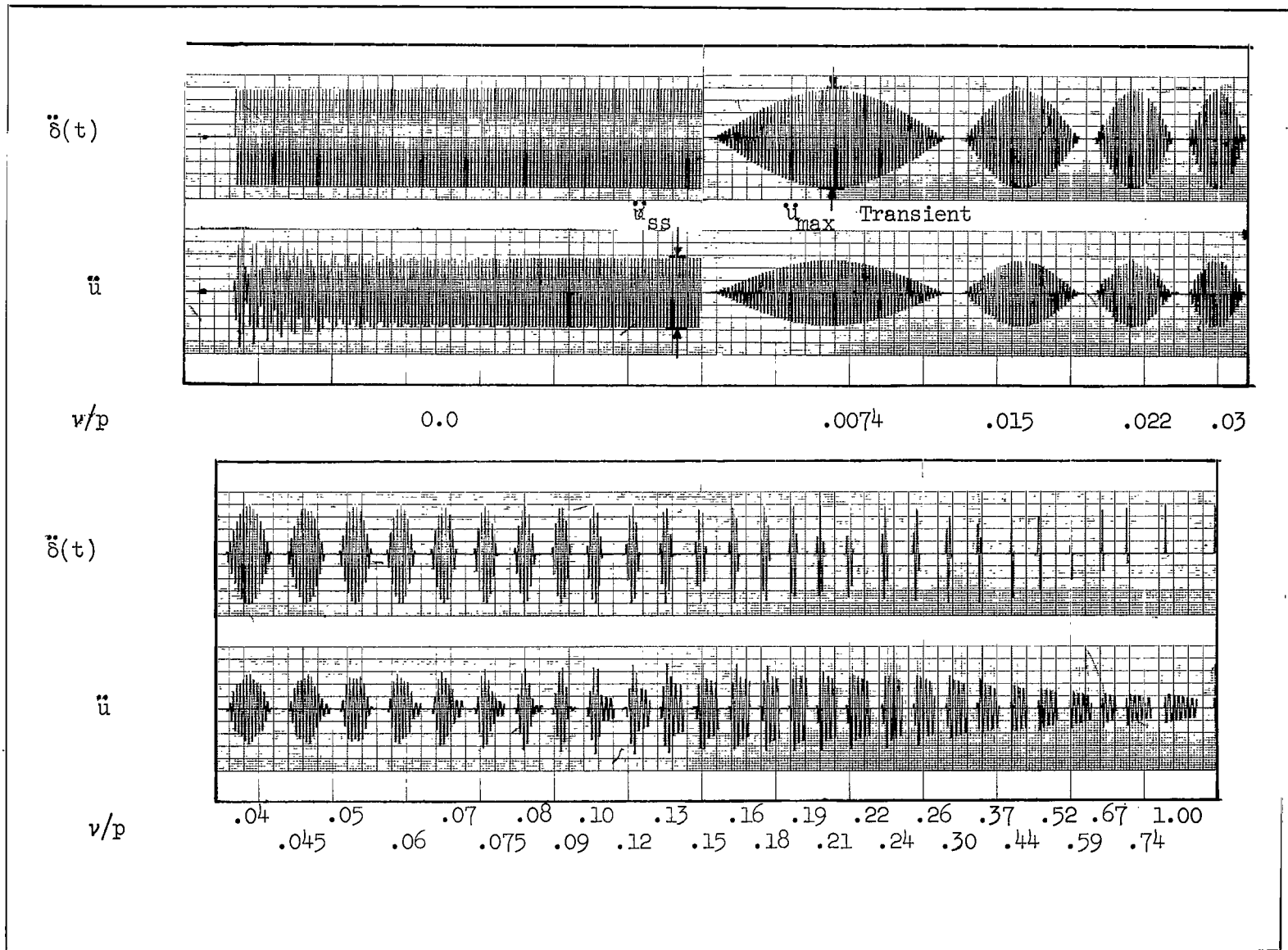
Figure 1.- Typical analog response curves for a simple mass system forced by a modulated sine function for \zeta = 0.01 and \rho/\omega = 1.35 . \ddot{\delta}(t) = A \sin pt \sin vt .
