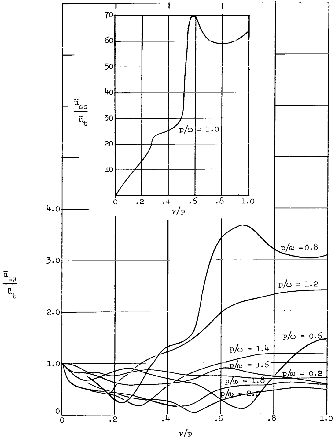
Figure 2.- Response ratios for modulated sine excitation showing effects of \nu/p and p/\omega . \zeta = 0.01 .
