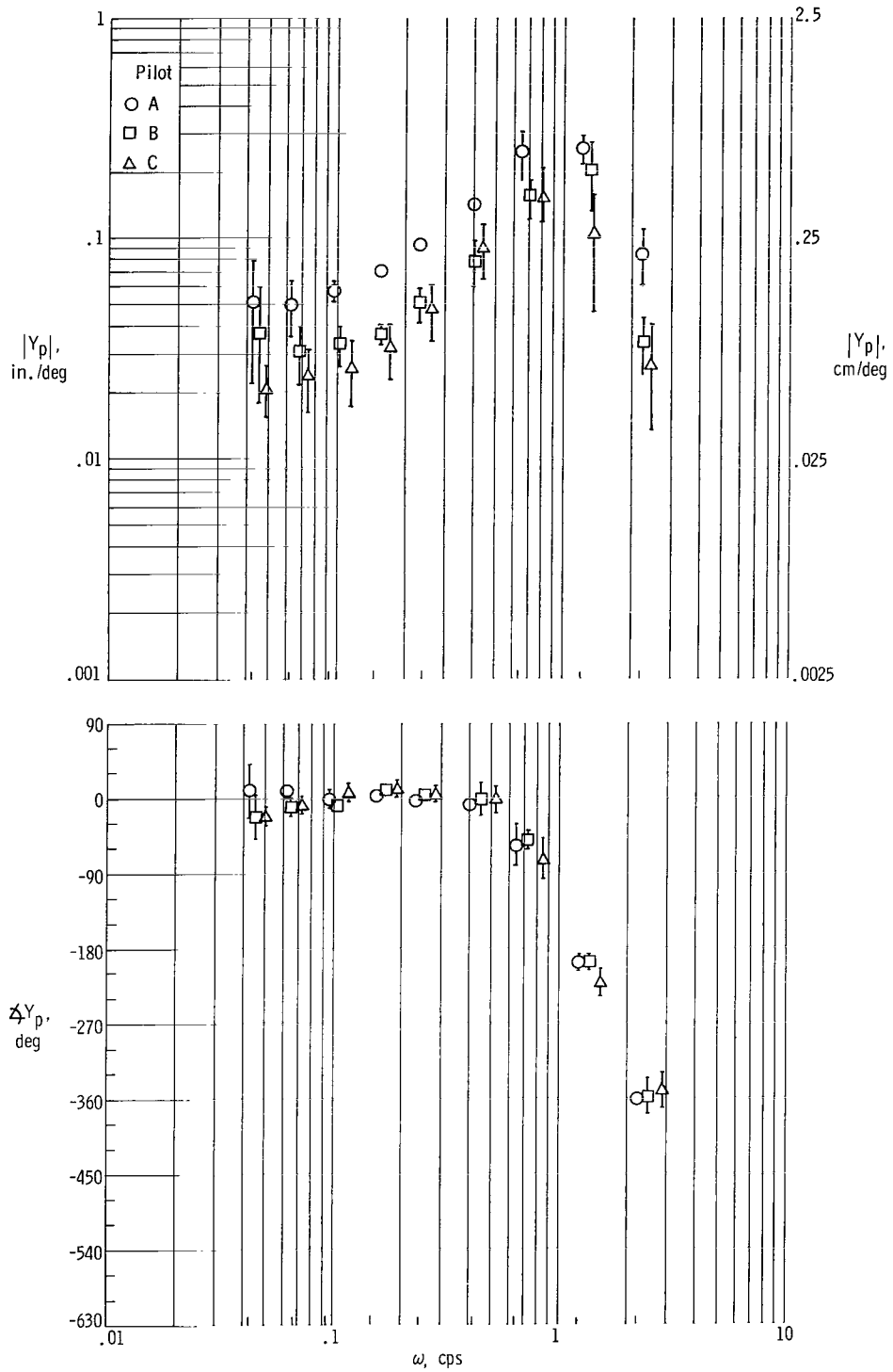
(e) Controlled element A-2, T-33 ground.
