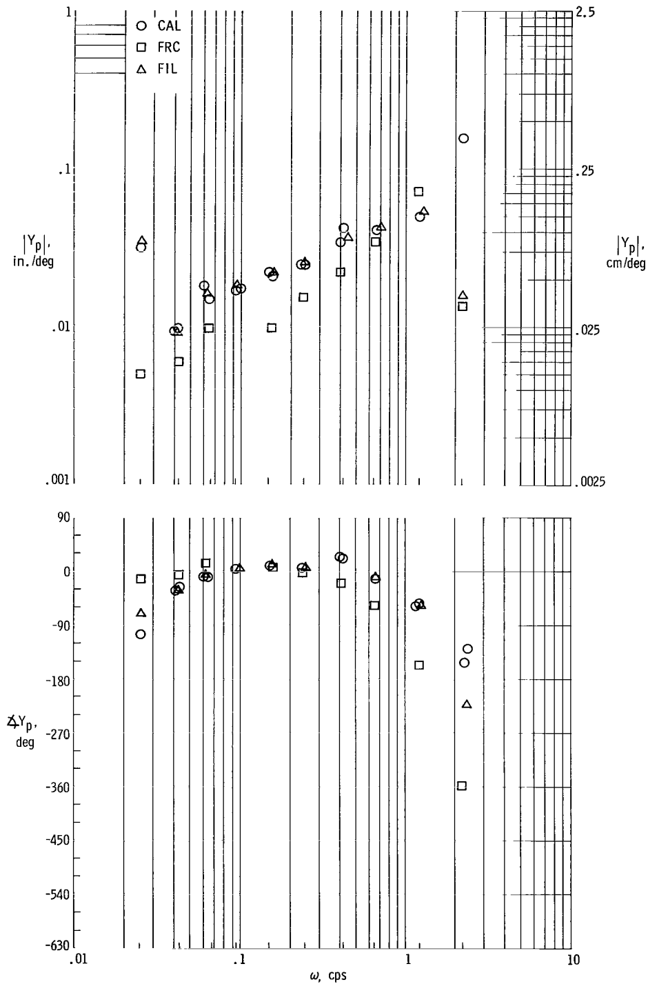
(g) Controlled element A-2 flight, run 97.
