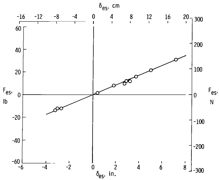
(b) Elevator stick force.
