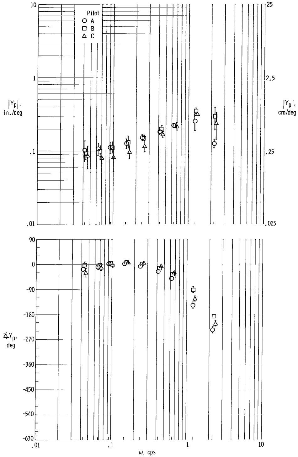
(g) Controlled element A-2*, contact analog.
