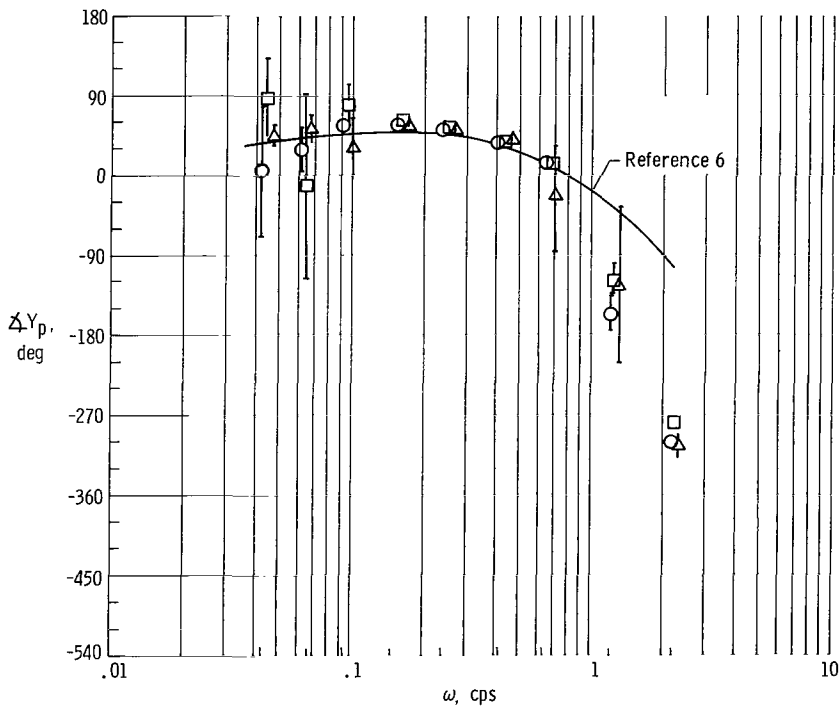
(c) Controlled element \frac{K}{s(s - \frac{1}{T})} , T-33 ground.
