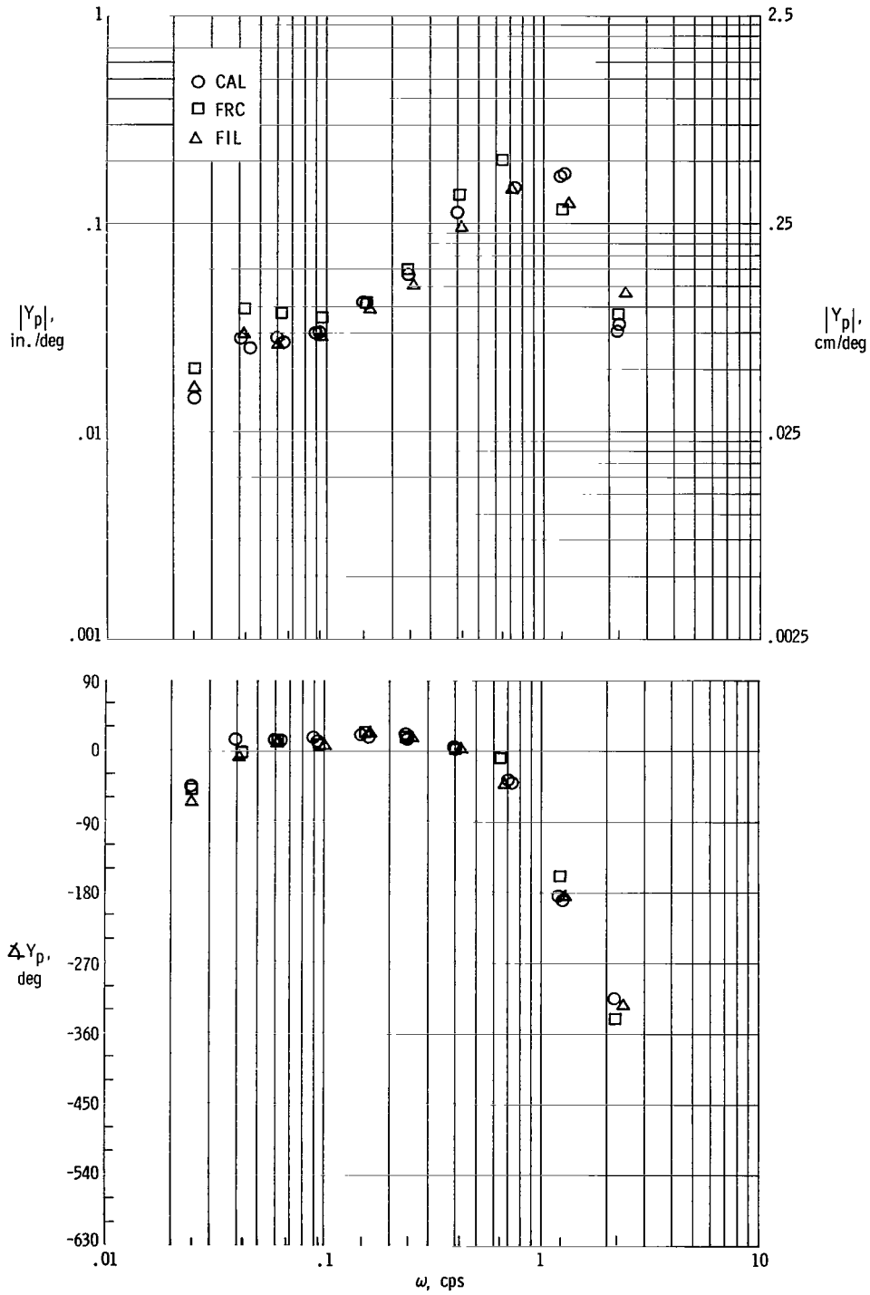
(e) Controlled element A-2* ground, run 69.
