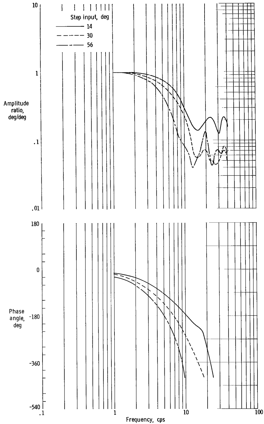
Figure 6.— Frequency response of T-33 bank-angle indicator.
