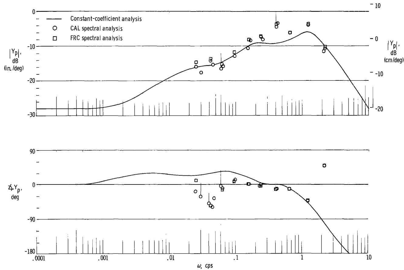
Figure 15.— Comparison of pilot transfer characteristic Y_p obtained from constant-coefficient analyses with those obtained from spectral analyses for controlled element A-2 flight, run 106.
