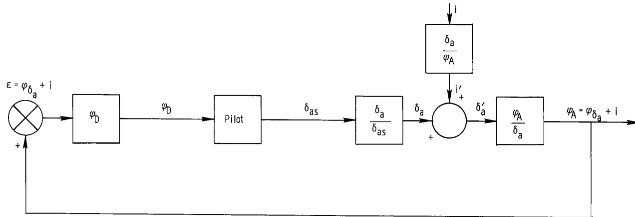
Figure 3. - Block diagram of compensatory tracking task with shaped input i' (for configuration A-2).
