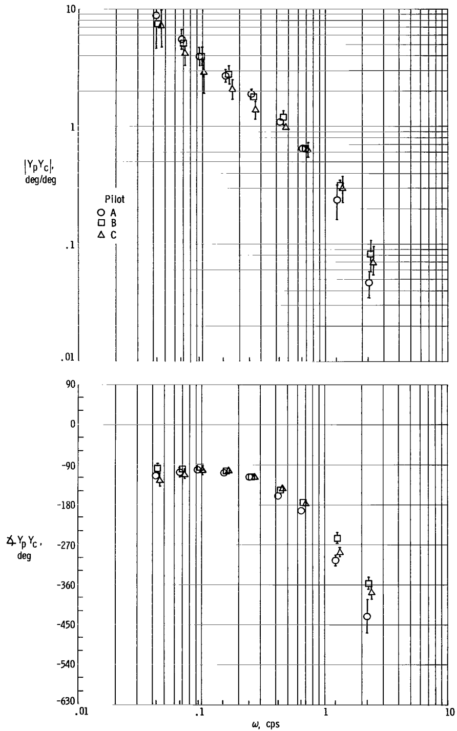
(f) Controlled element A-2*, contact analog.
