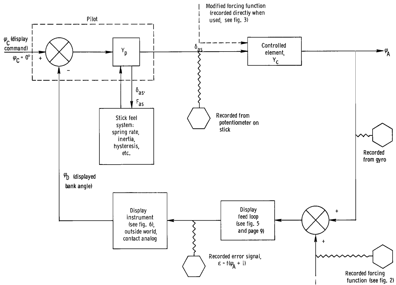
Figure 1. - General block diagram of the experiment.
