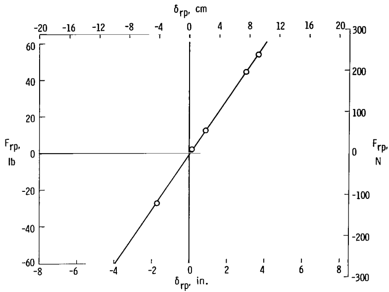
(a) Rudder pedal force.
