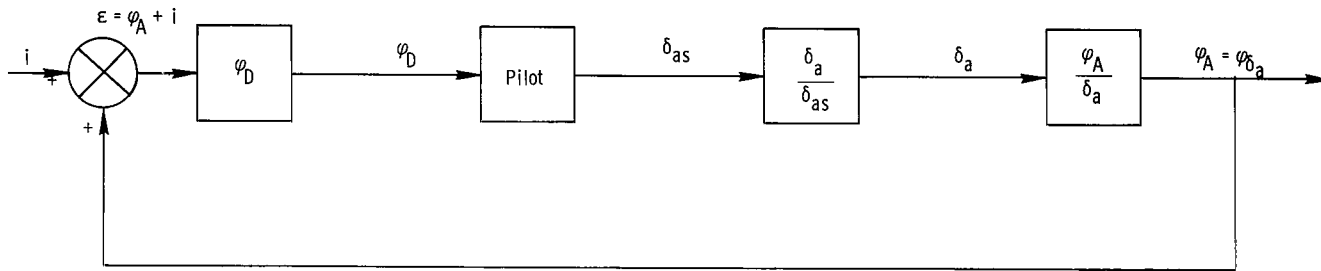
Figure 2. - Block diagram of compensatory tracking task with unshaped input i (for configuration A-2*, \frac{K}{s} , and \frac{K}{s(s - \frac{1}{T})} ).
