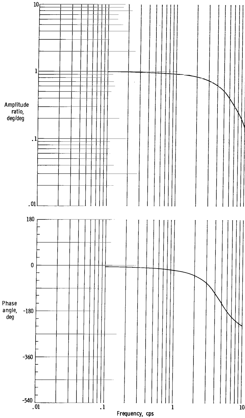
Figure 5. — Frequency response of bank-angle servo in computer interface equipment (T-33).
