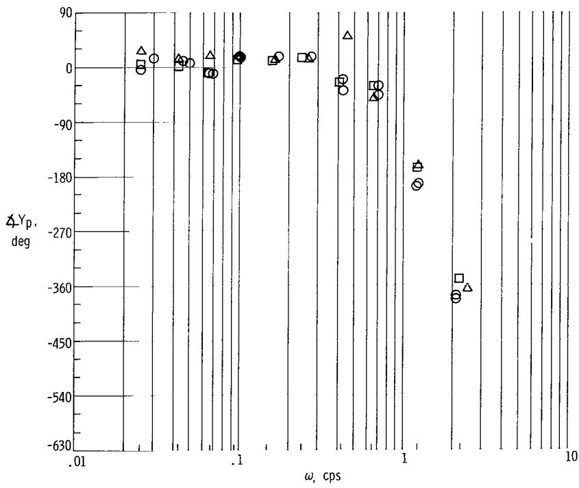
(h) Controlled element A-2 flight, run 118.
