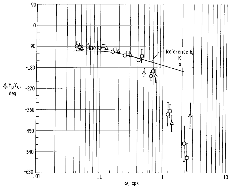
(g) Controlled element A-2*, T-33 flight.
