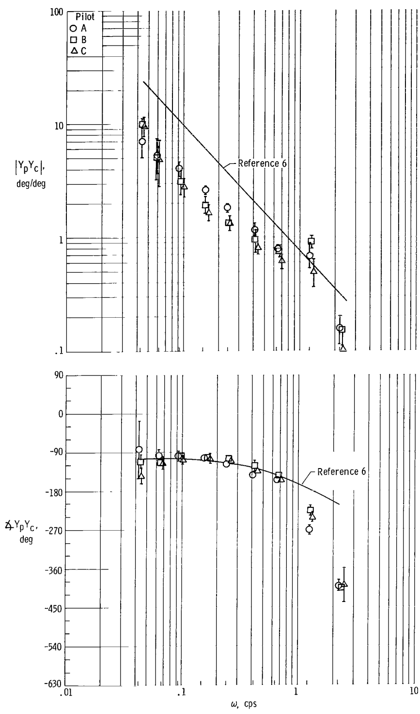
(a) Controlled element \frac{K}{s} , T-33 ground.
