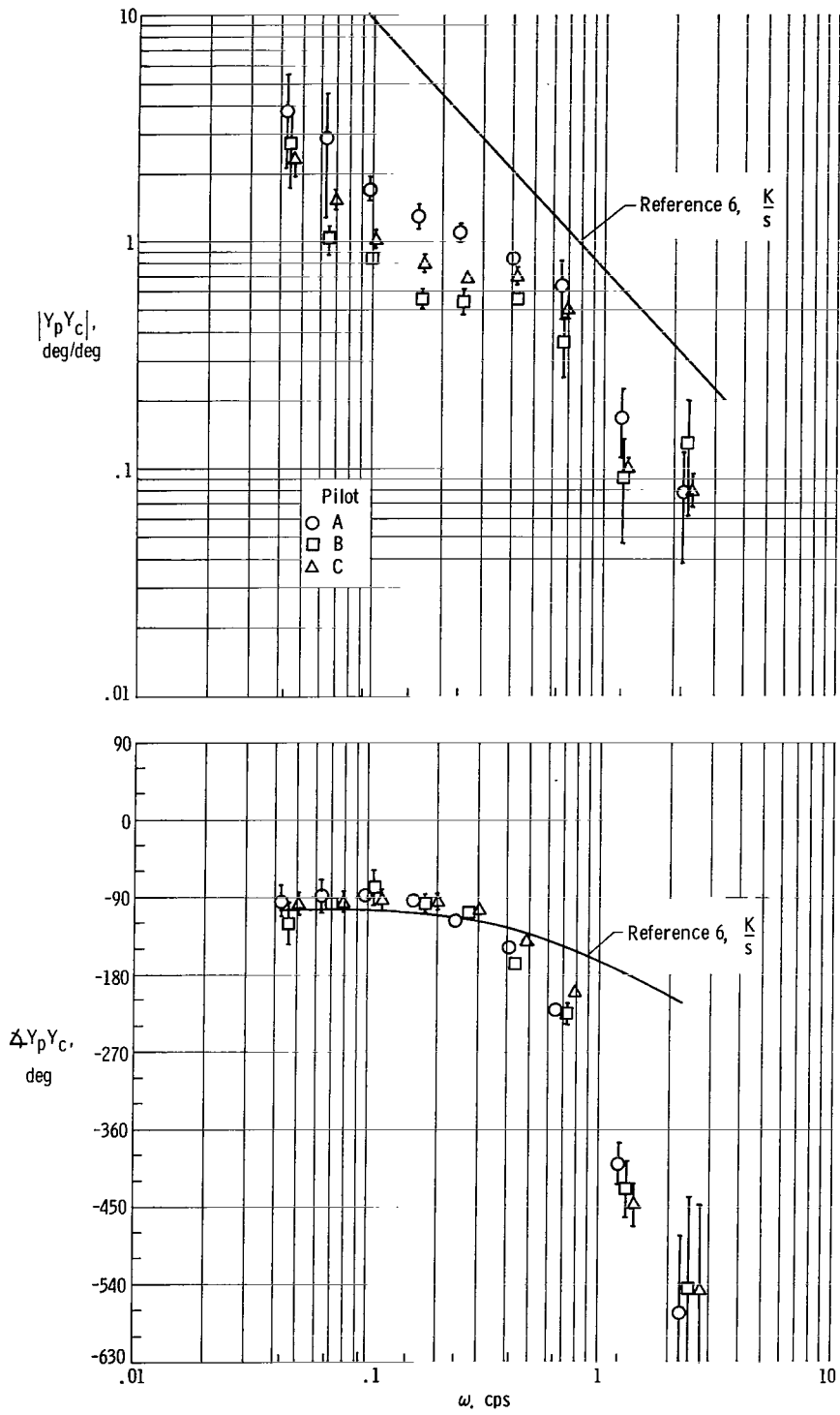
(e) Controlled element A-2*, T-33 ground.
