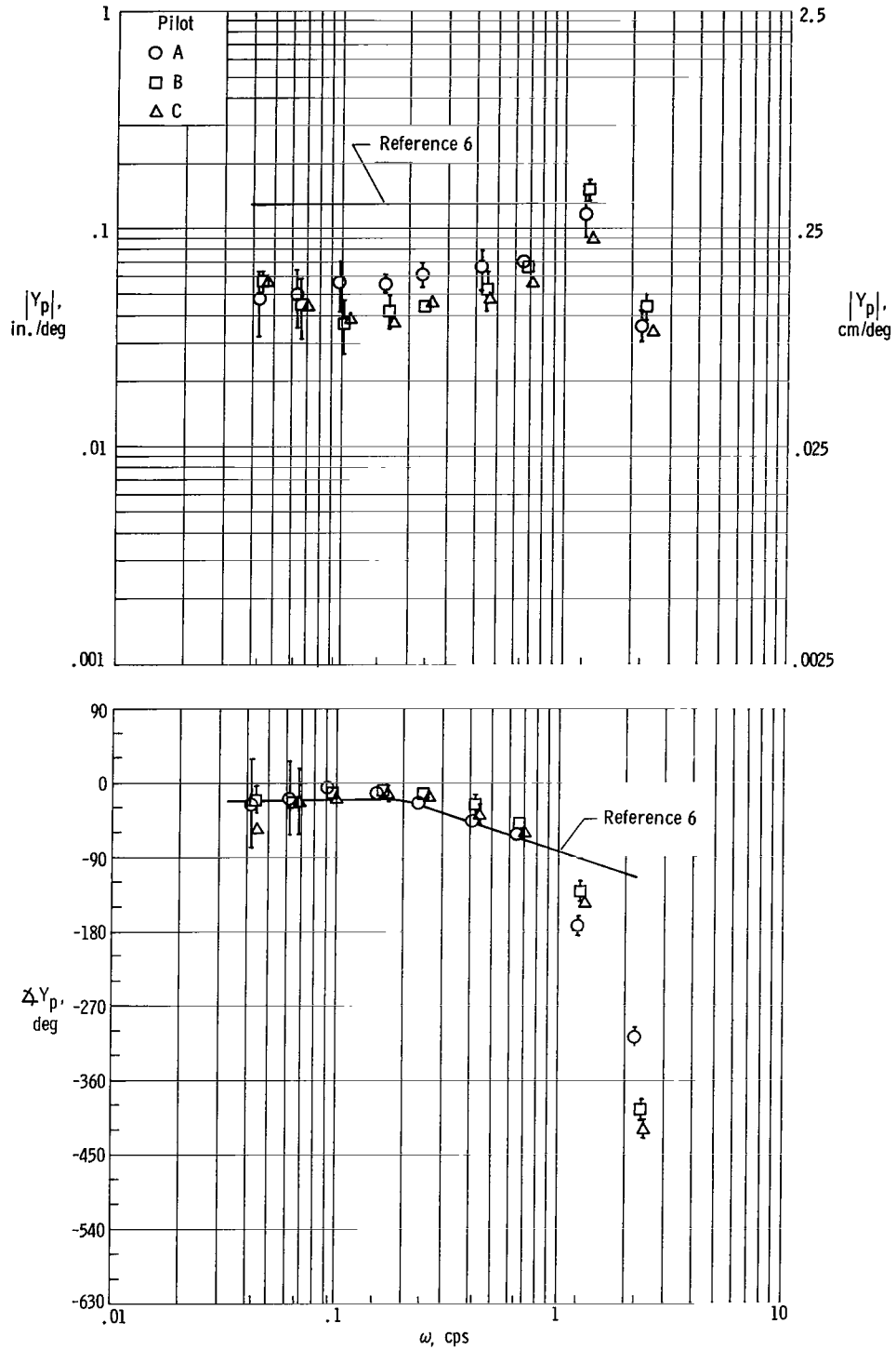
(a) Controlled element \frac{K}{s} , T-33 ground.
