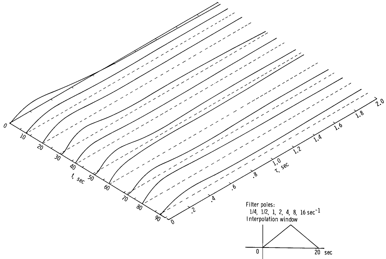
(a) Response of model to step input.
