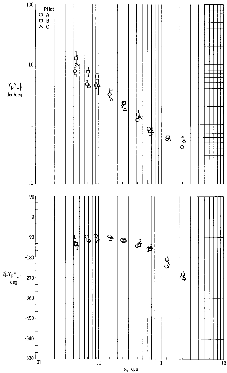
(b) Controlled element \frac{K}{s} , contact analog.
