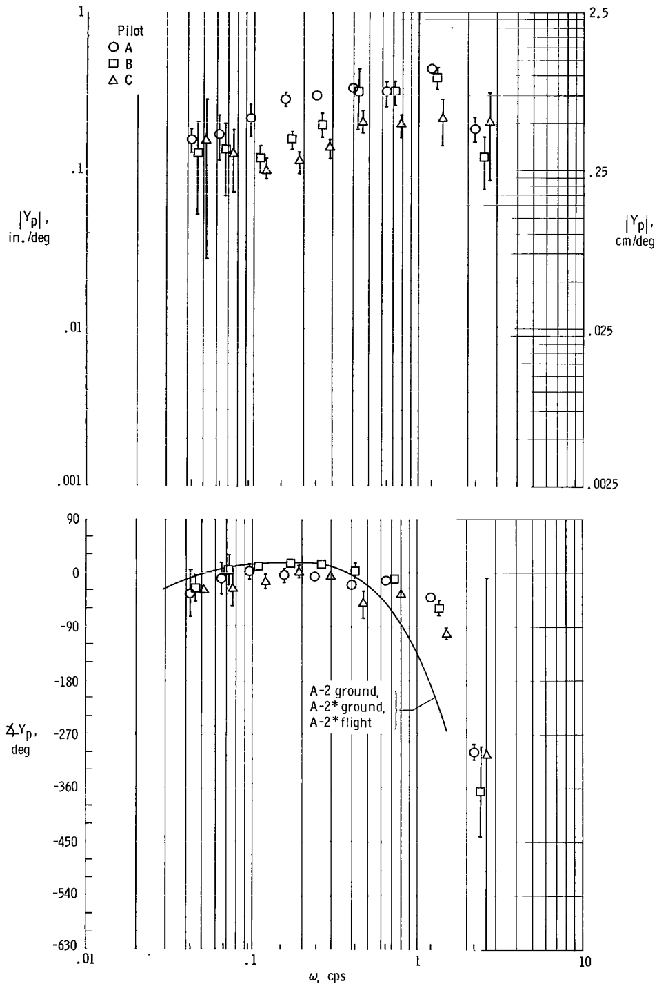
(h) Controlled element A-2, T-33 flight.
