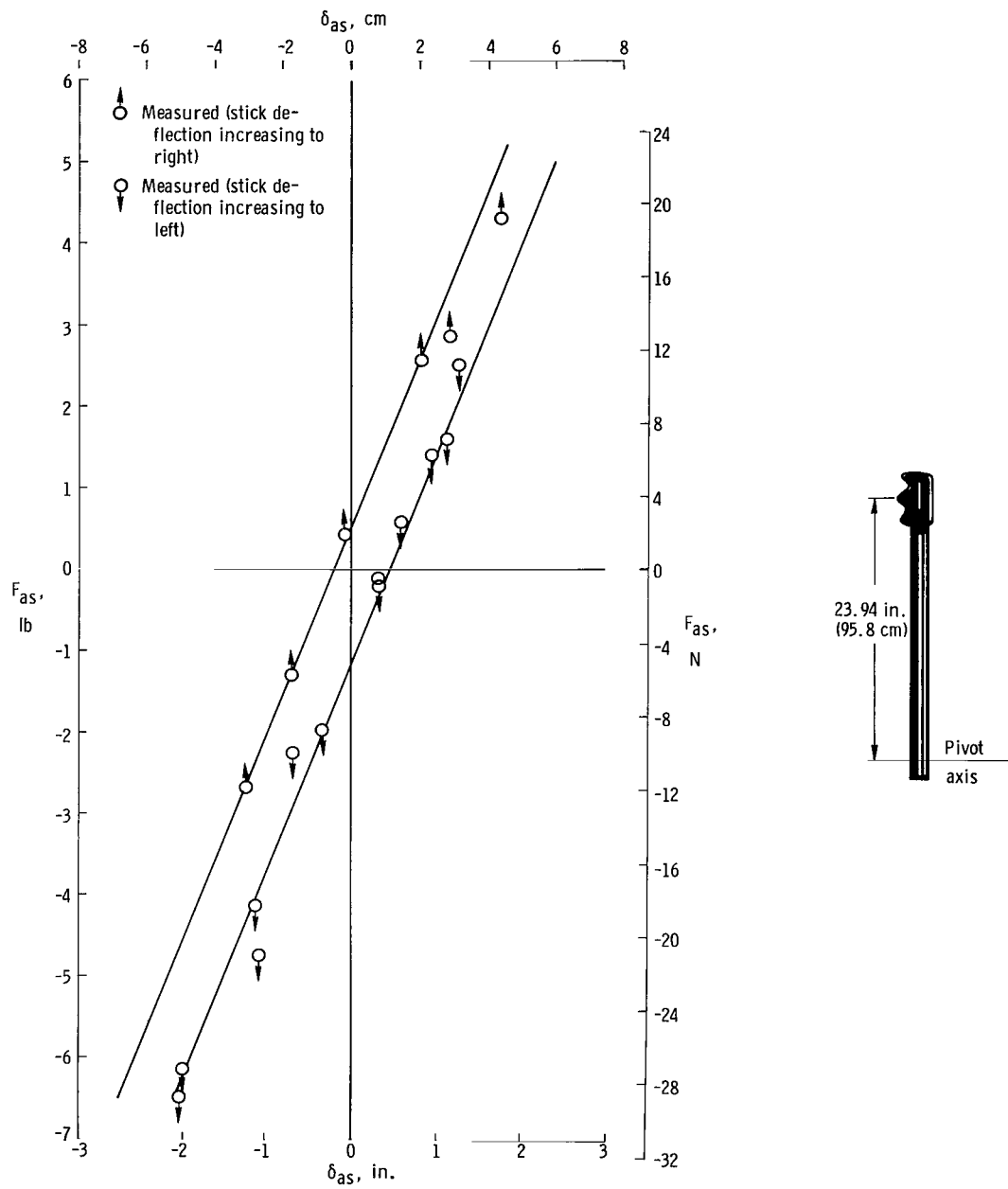
Figure 8. - Hysteresis loop of T-33 aileron stick force as a function of aileron displacement.
