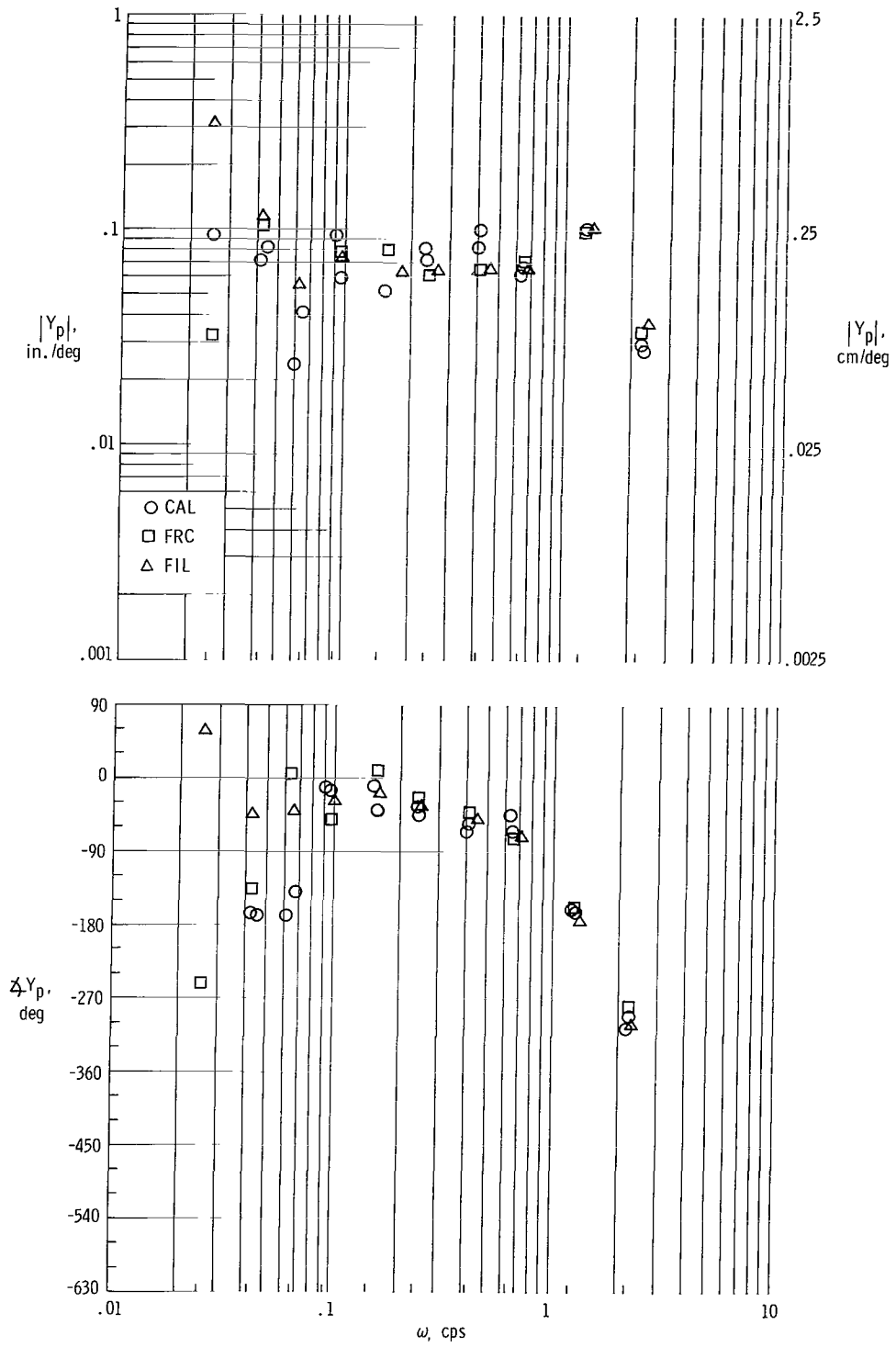
(b) Controlled element \frac{K}{s} , run 25.
