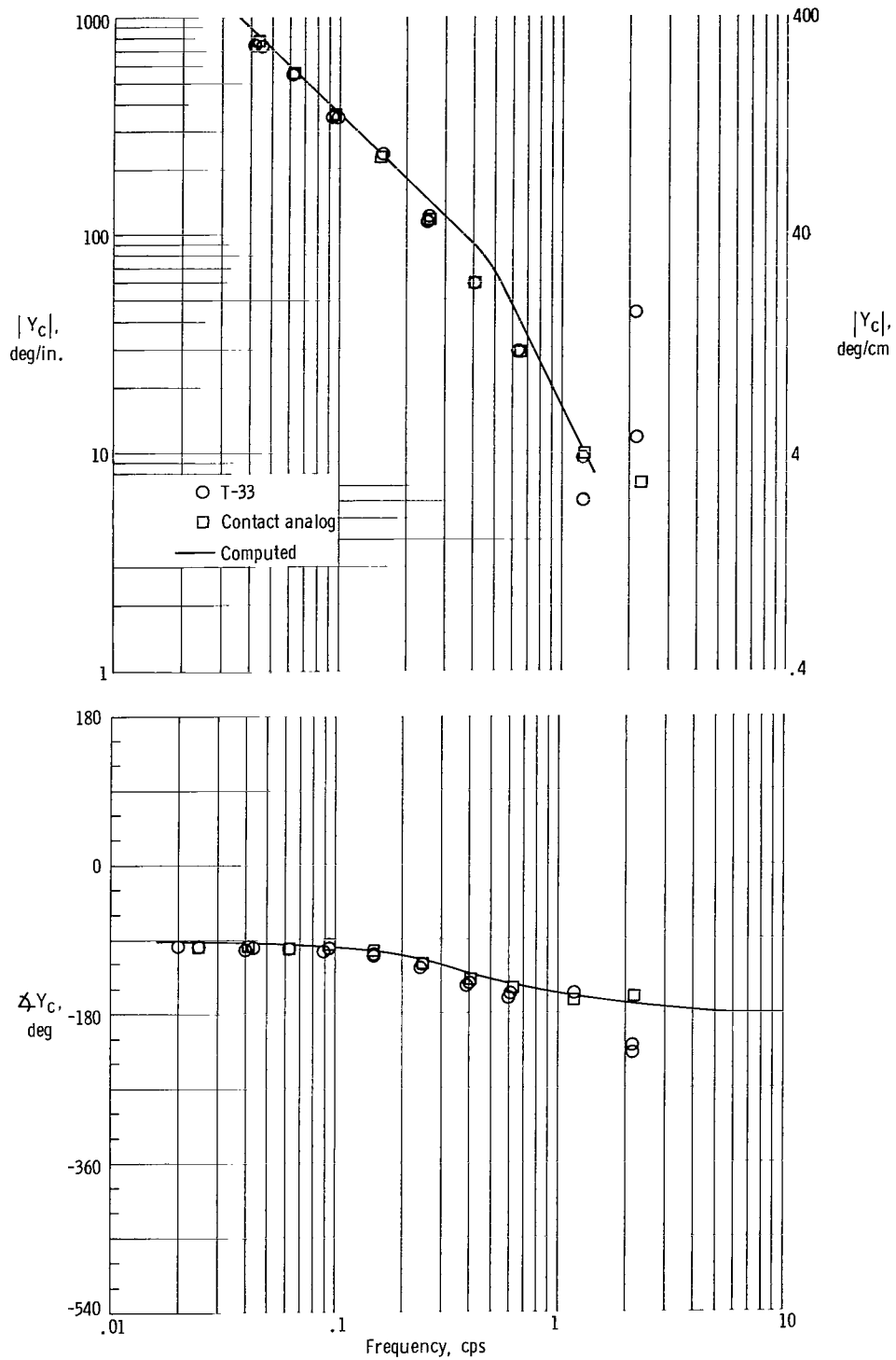
Figure 13. — Comparison of measured and computed Y_c for controlled element A-2*.
