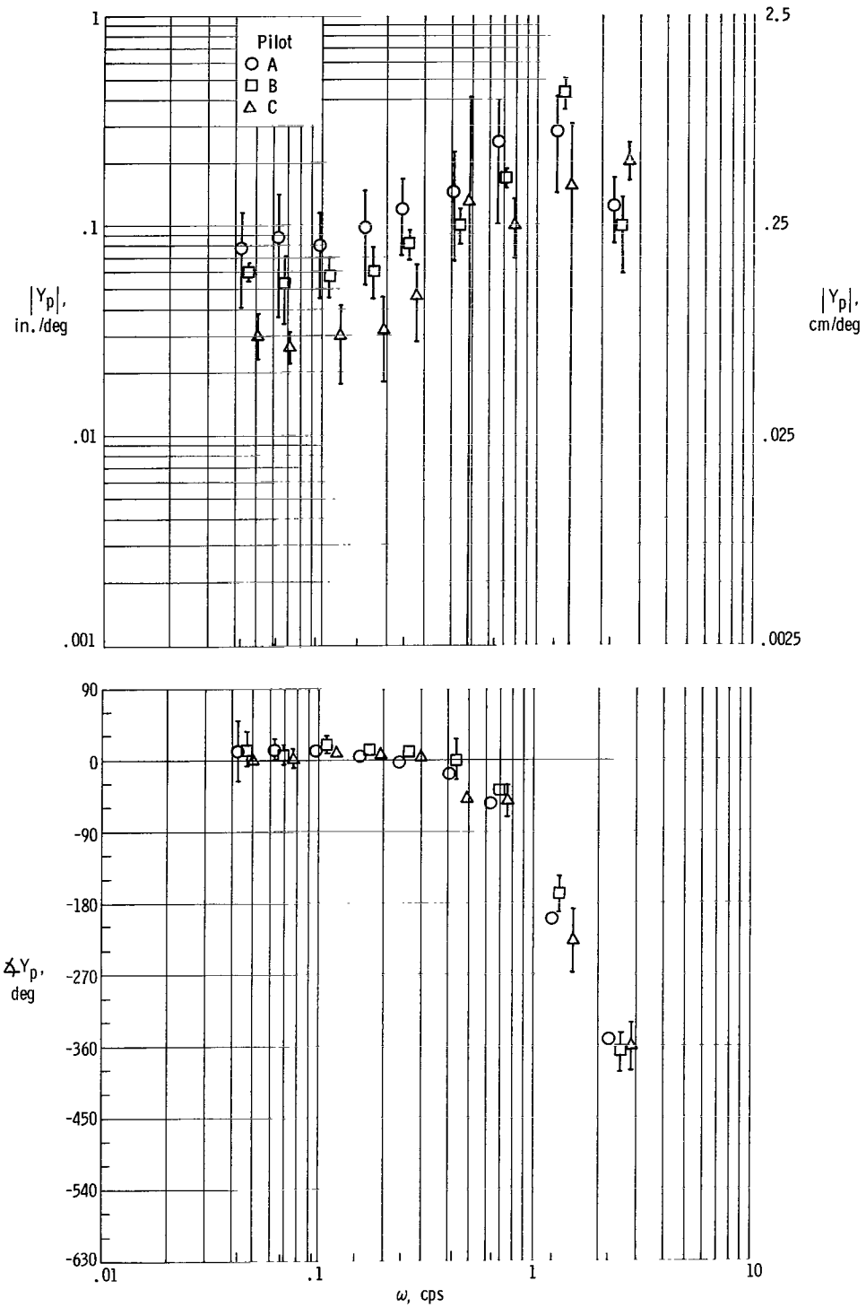
(i) Controlled element A-2*, T-33 flight.
