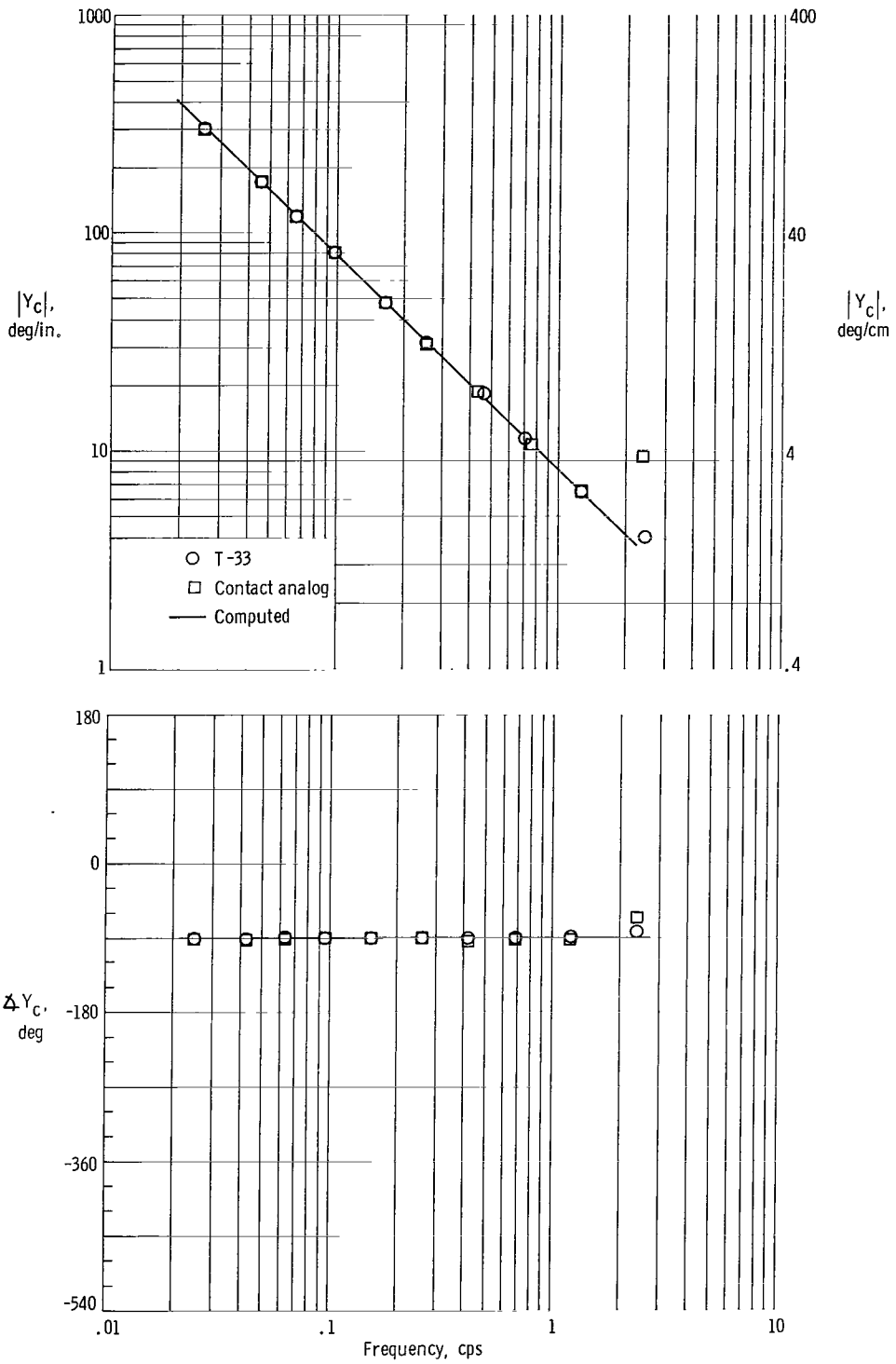
Figure 11.— Comparison of measured and computed Y_c for controlled element \frac{K}{s} .
