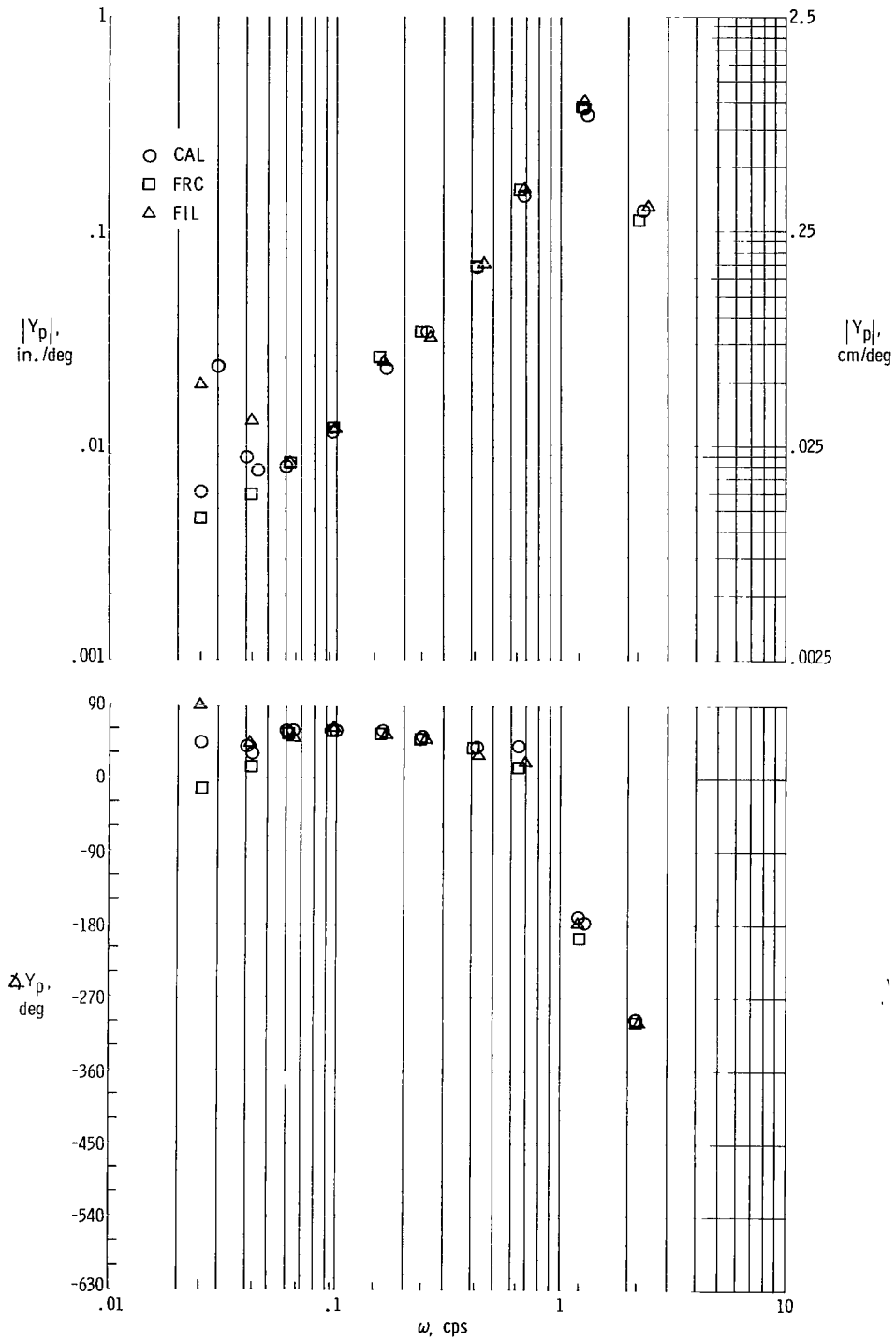
(a) Controlled element \frac{K}{s(s - \frac{1}{T})} , run 4.
