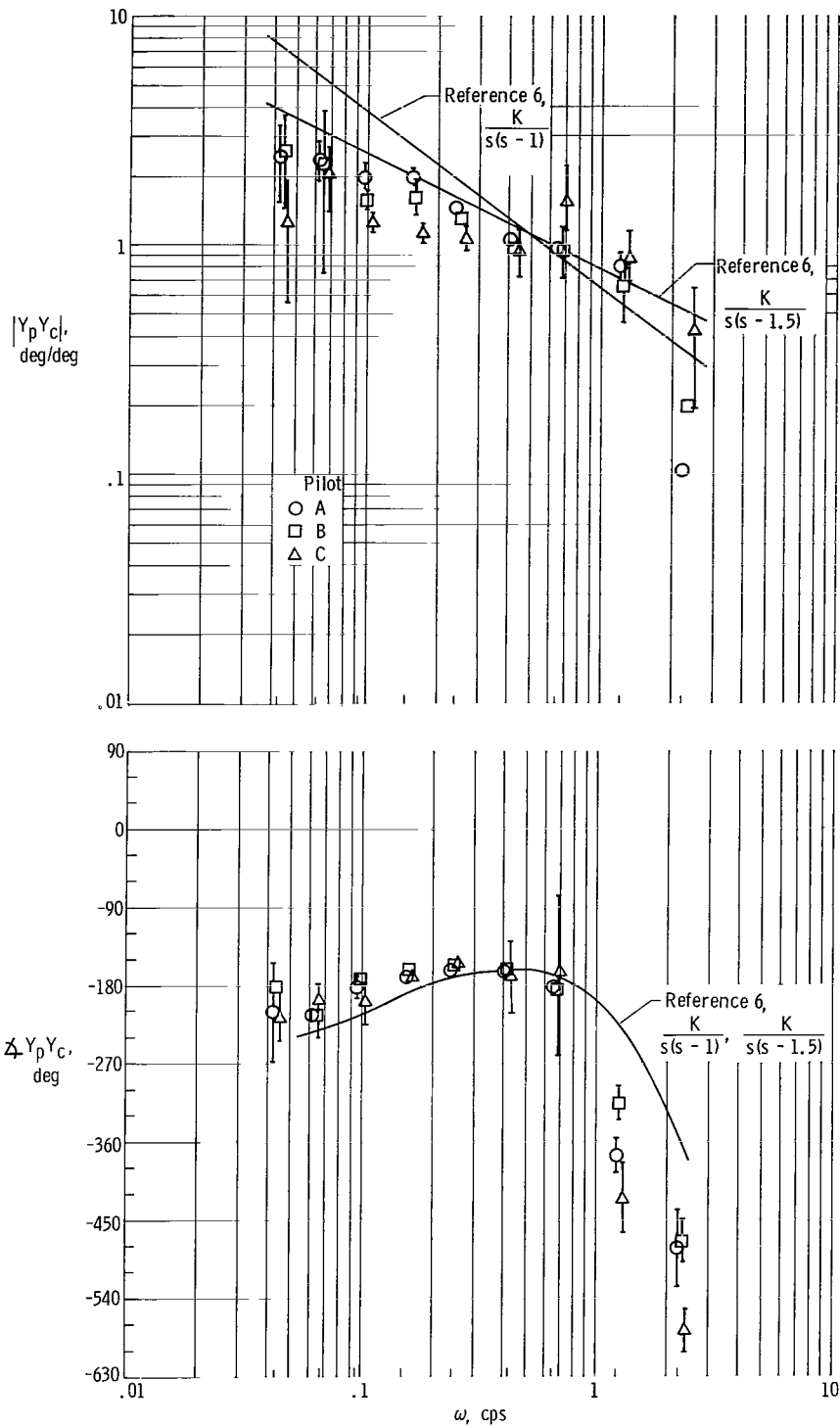
(c) Controlled element \frac{K}{s(s - \frac{1}{T})} , T-33 ground.
