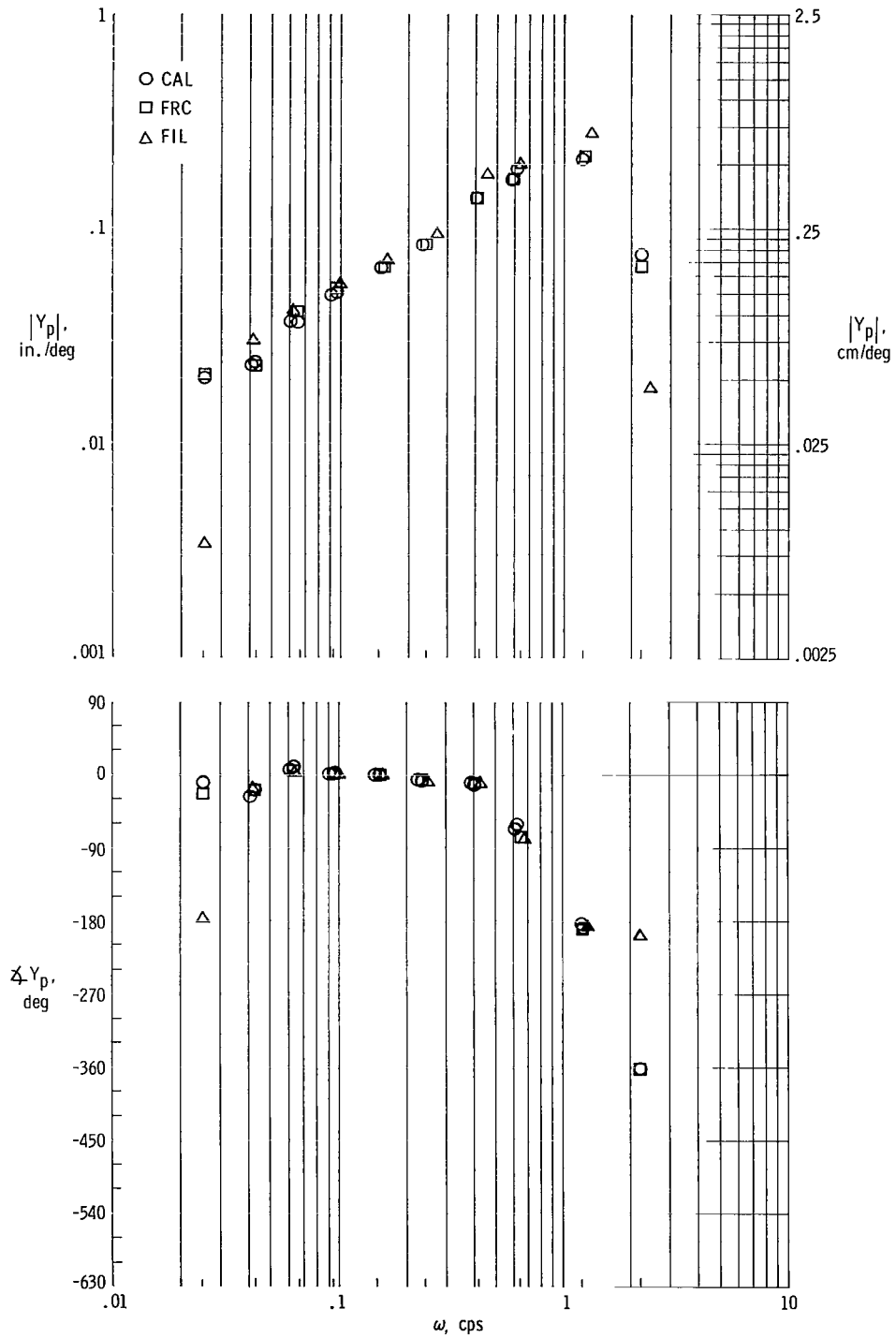
(c) Controlled element A-2 ground, run 39.
