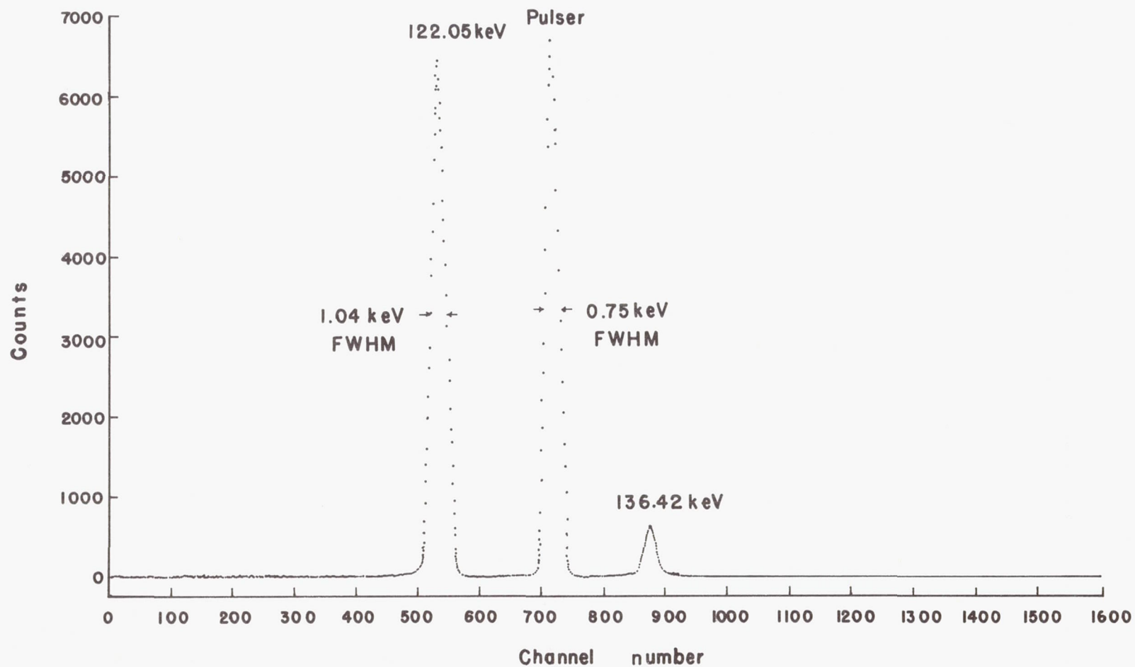
Figure 7.- Gamma rays of \text{Co}^{57} . Si(Li) detector at 77 o K and 490 V bias; energy resolution, 0.043 keV/ch.
