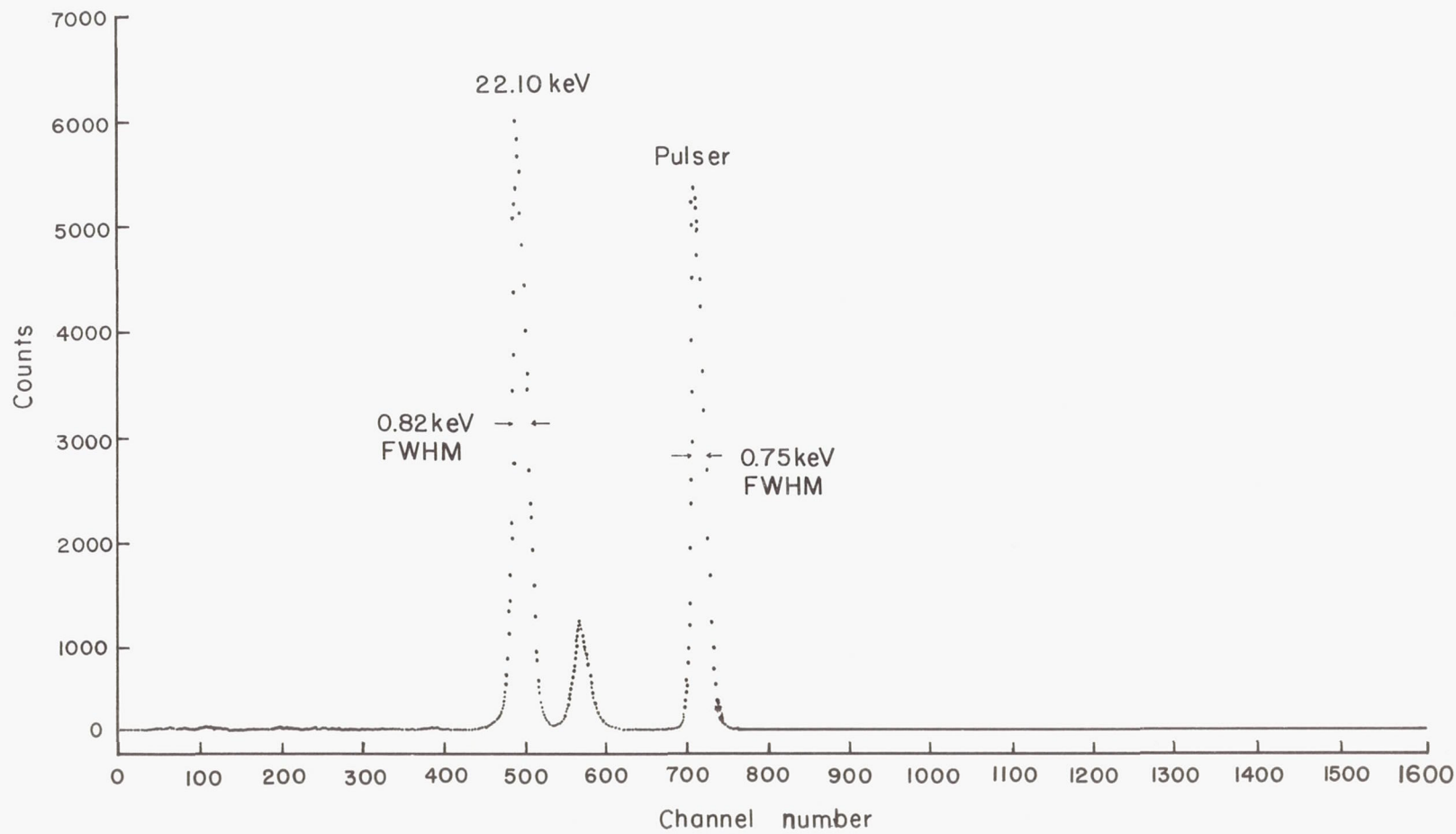
Figure 6.- X-ray spectrum of Cd 109 . Si(Li) detector at 77° K and 490 V bias; energy resolution, 0.043 keV/ch.
