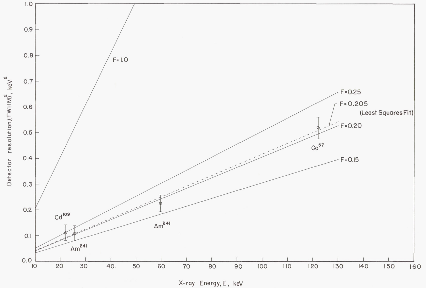
Figure 9.- Fano factor for Si(Li) detectors. (FWHM)^2 = (2.355)^2 E F E .
