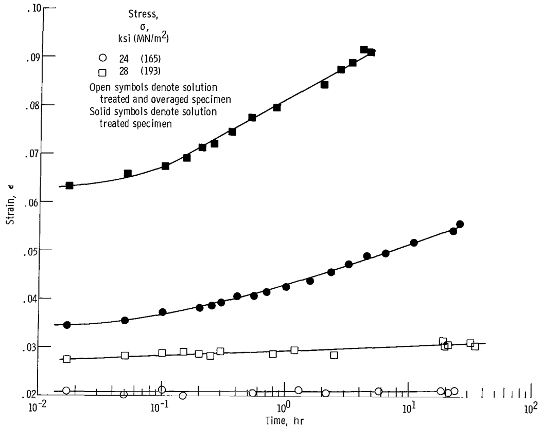
Figure 7. - Effect of overaging on creep behavior at 1800° F (1255 K).
