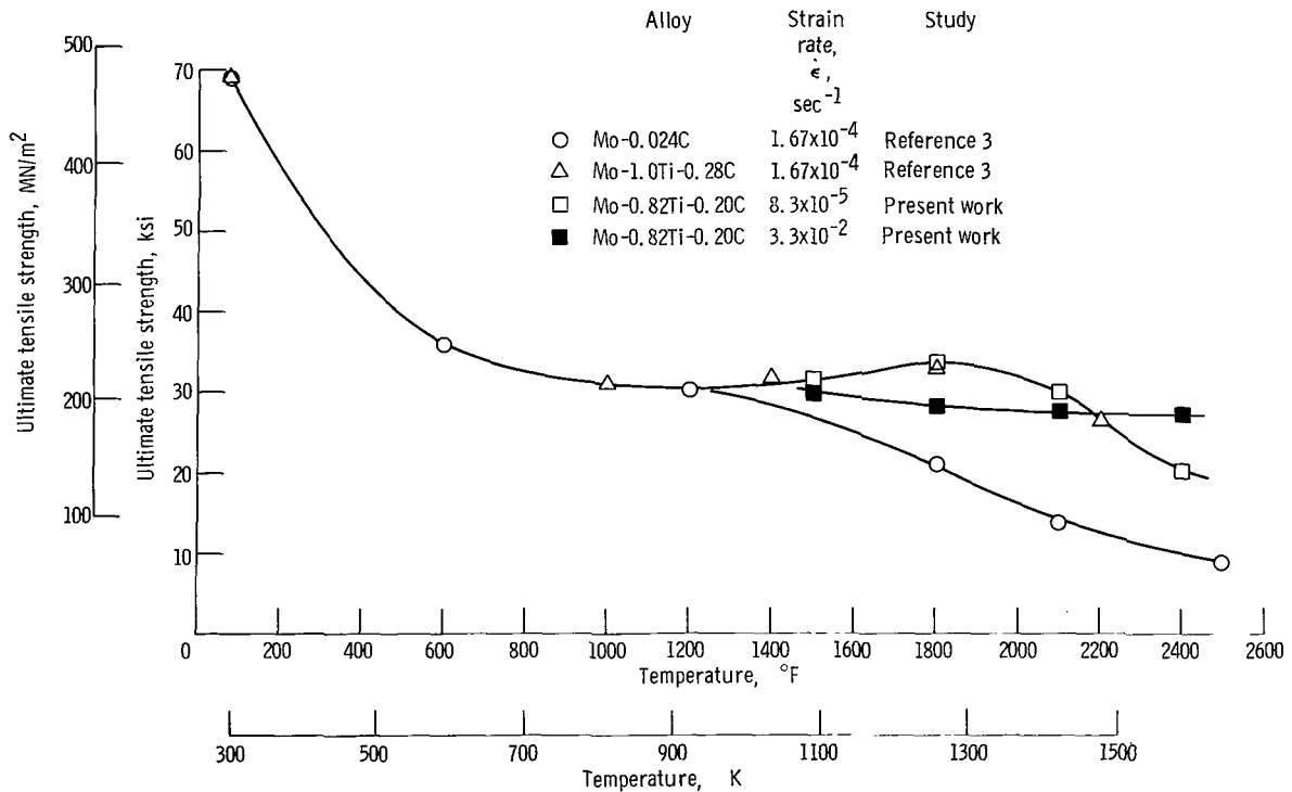
Figure 1. - Influence of temperature on ultimate tensile strength of molybdenum and Mo-Ti-C alloy.
