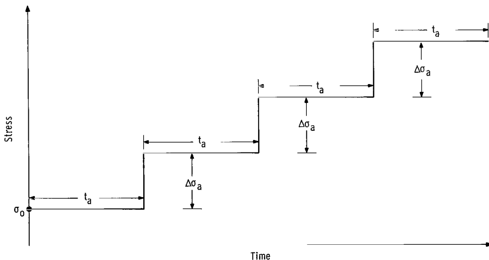
Figure 4. - Schematic of loading program used in incremental creep tests at 1800^\circ \text{ F} ( 1255 \text{ K} ), where t_a is time under given creep stress and \Delta\sigma_a is change in stress during incremental creep test.
