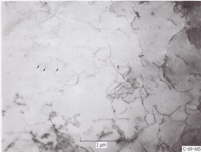
Figure 11. - Transmission electron micrograph taken from specimen tested at 1800° F (1255 K). Prestrained at 24 kips per square inch (165 MN/m 2 ) for 24 hours and then tested at 28 kips per square inch (193 MN/m 2 ) see figure . Arrows indicate selected precipitates on dislocations. X50 000.
