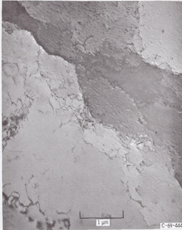
Figure 10. - Microstructure of specimen crept at 3200° F (2033 K) at stress of 2.5 kips per square inch. (17.2 MN/m 2 ). X30 000.
