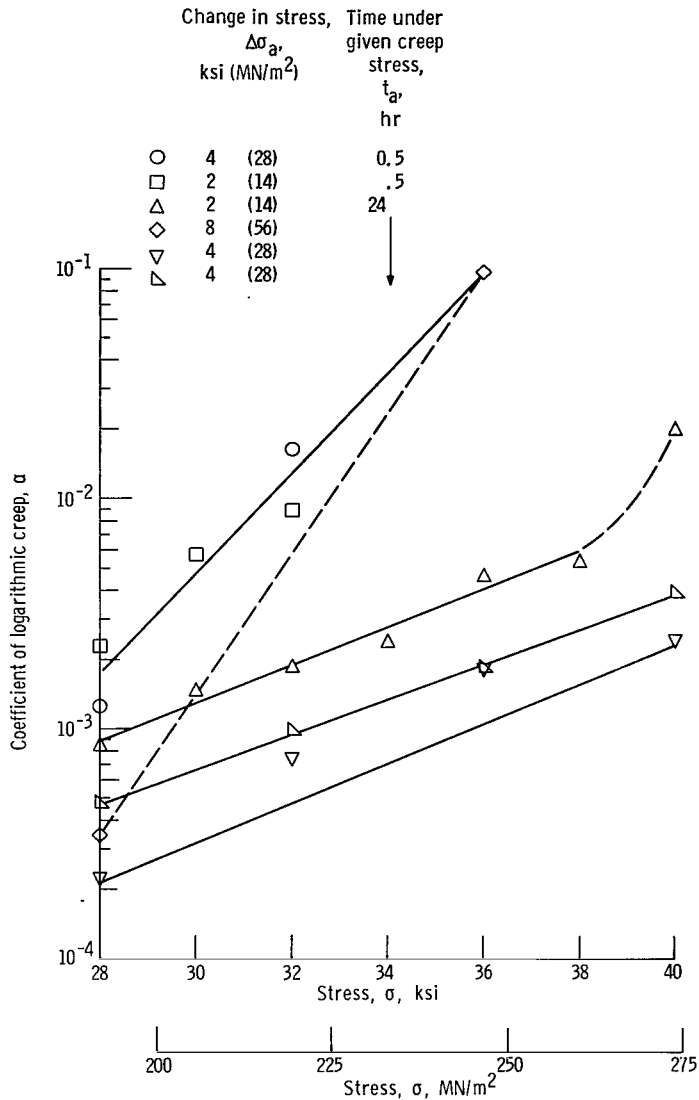
Figure 6. - Stress dependence of logarithmic creep constant \alpha for different loading histories.
