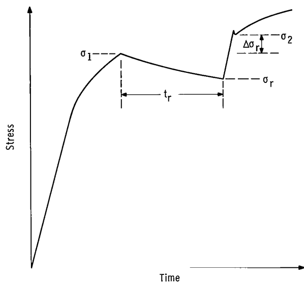
Figure 8. - Schematic of relaxation experiment showing definition of terms, where t_r is relaxation time, \sigma_1 is initial stress in stress relaxation test, \sigma_2 is yield stress on reloading after stress relaxation, \sigma_r is stress at time t_r , and \Delta\sigma_r = \sigma_2 - \sigma_1 .
