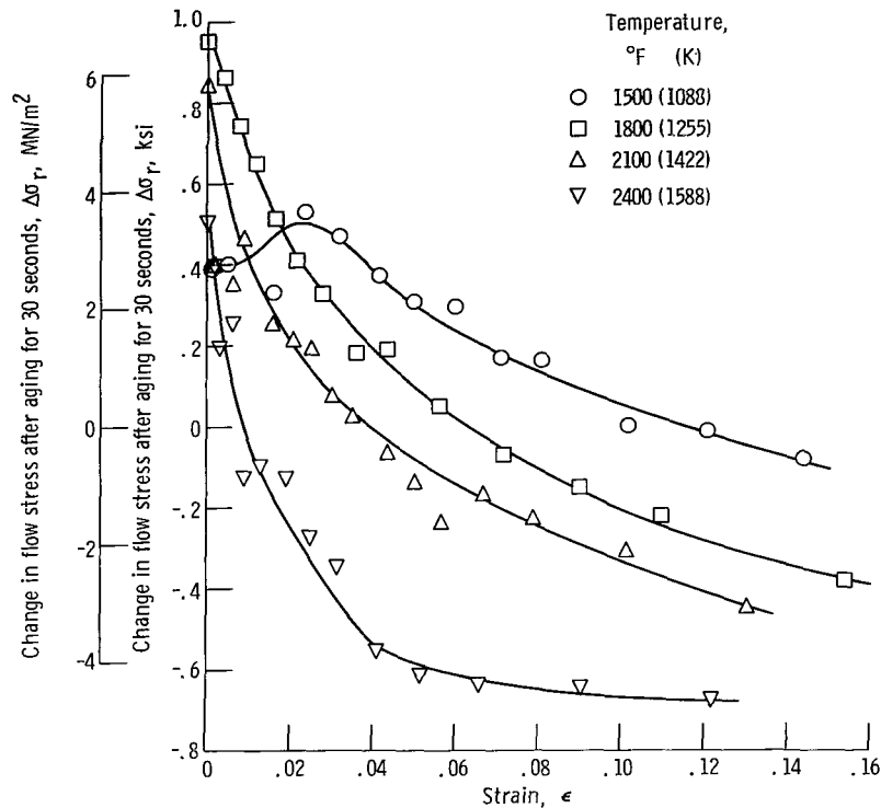
Figure 9. - Stress increment \Delta\sigma_r , after aging under constant strain for 30 seconds, as function of strain and temperature.
