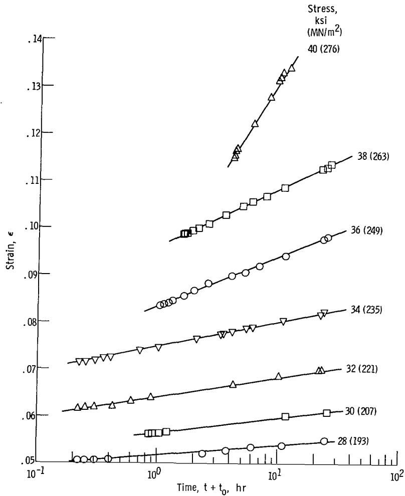
Figure 5. - Logarithmic creep of Mo-Ti-C alloy at 1800^\circ F ( 1255 K). Time under given creep stress, 24 hours; change in stress during incremental creep test, 2 kips per square inch ( 14 MN/m ^2 ).
