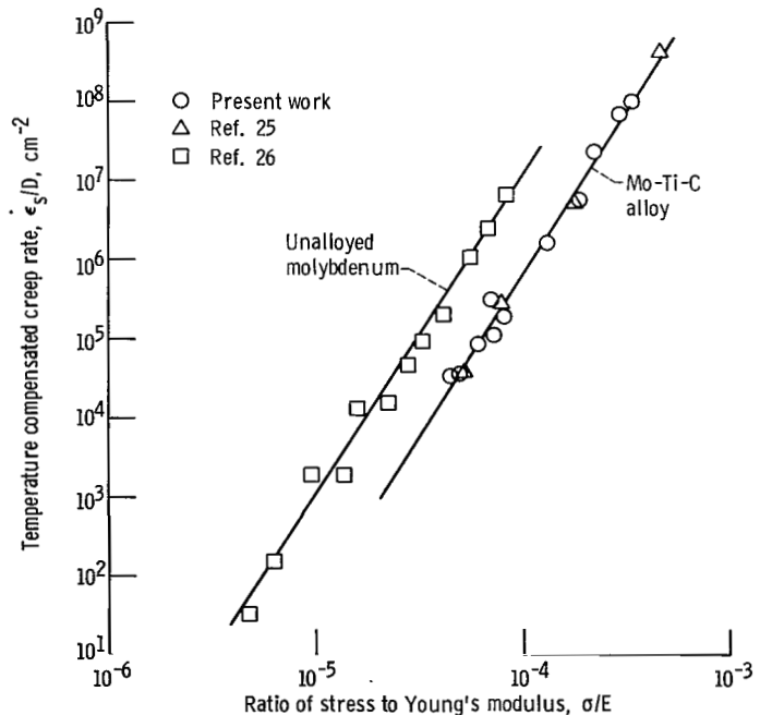
Figure 2. - Low stress creep of molybdenum (ref. 26) and Mo-Ti-C alloy (present work and ref. 25).
