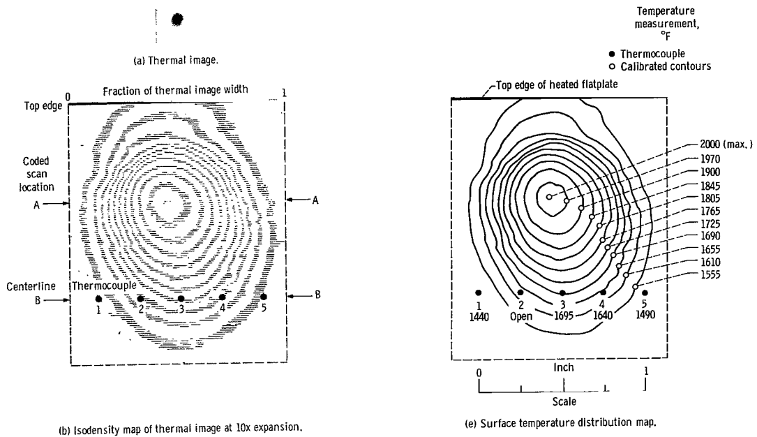
(b) Isodensity map of thermal image at 10x expansion.
