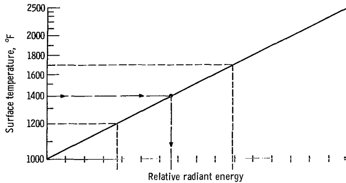
(a) Master temperature distribution (MTD) curve.
