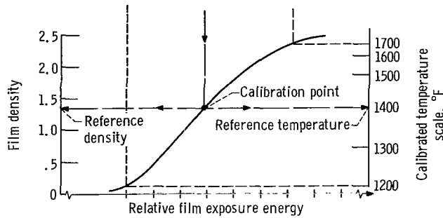
(b) Film response (FR) curve.
