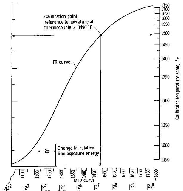
(d) Calibration curve of film density to surface temperature.
