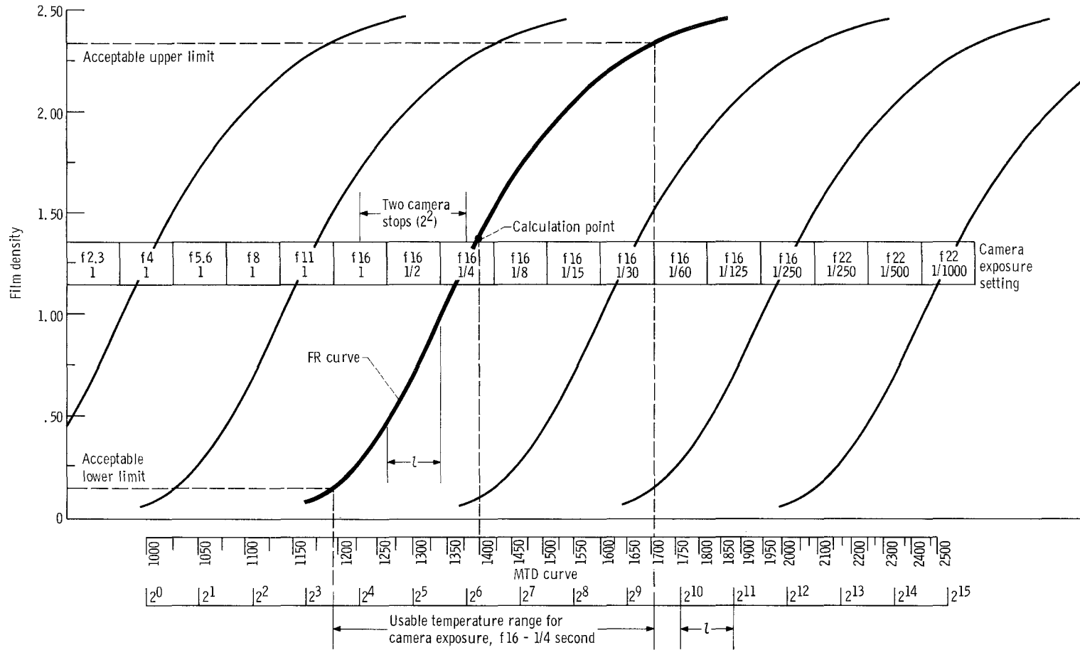
Figure 8. - Typical system calibration guide chart showing usable temperature range for various camera exposures. l = 2x change in relative energy.
