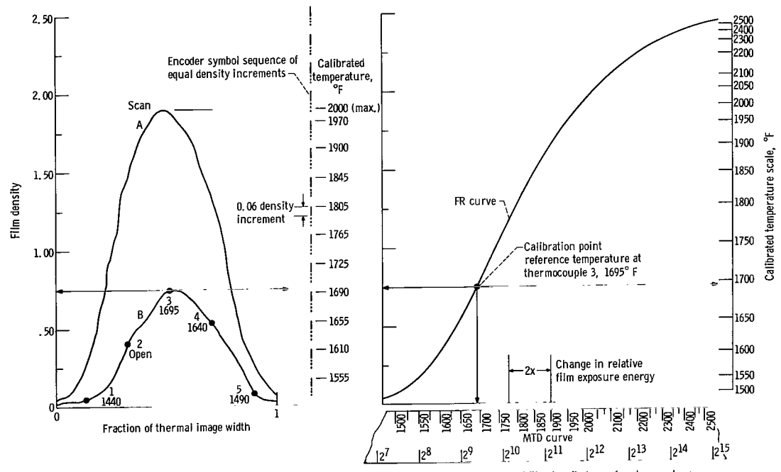
(c) Conventional film density profile scan at thermocouple locations indicated in (b).
