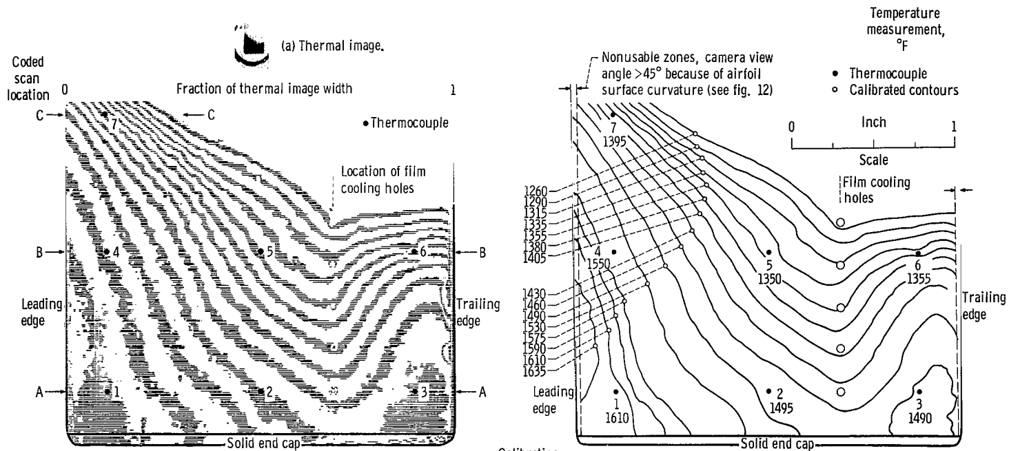
(a) Thermal image. (b) Isodensity map of thermal image at 20x expansion. (c) Conventional film density profile scan at locations indicated in (b).
