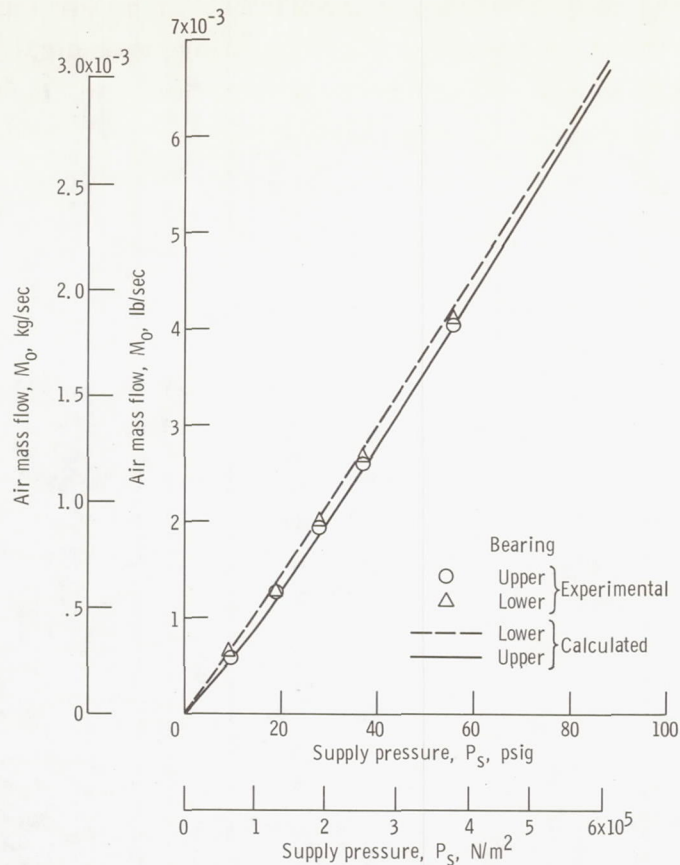
Figure 7. - Comparison of calculated and experimental values of air mass flow. Atmospheric pressure, 14.4 psia (99 kN/m 2 ); rotor diameter, 2.5 inches (6.3 cm); bearing length, 3.75 inches (9.5 cm); number of orifices per bearing, 12; orifice diameter, 0.022 inch (0.56 mm). Radial clearances: upper bearing, 0.00132 inch (0.0335 mm); lower bearing, 0.00138 inch (0.035 mm).
