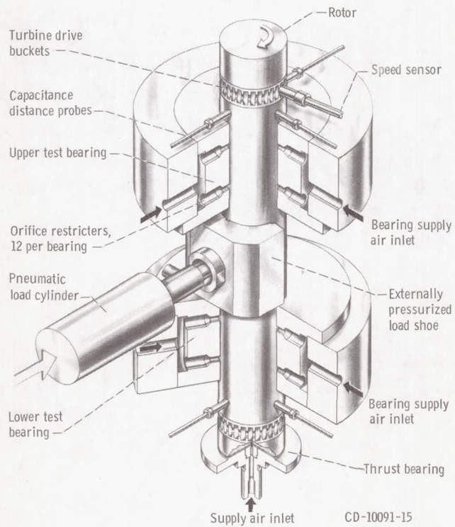
(b) Schematic.
