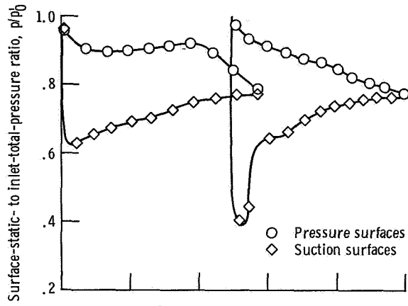
(a) Static-pressure distribution.
