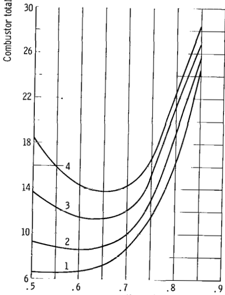
(c) Ratio of liner open area to reference area, 0.8.
