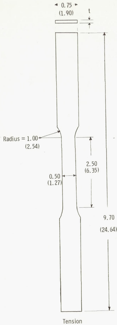
(a) Specimens from sheet material.
