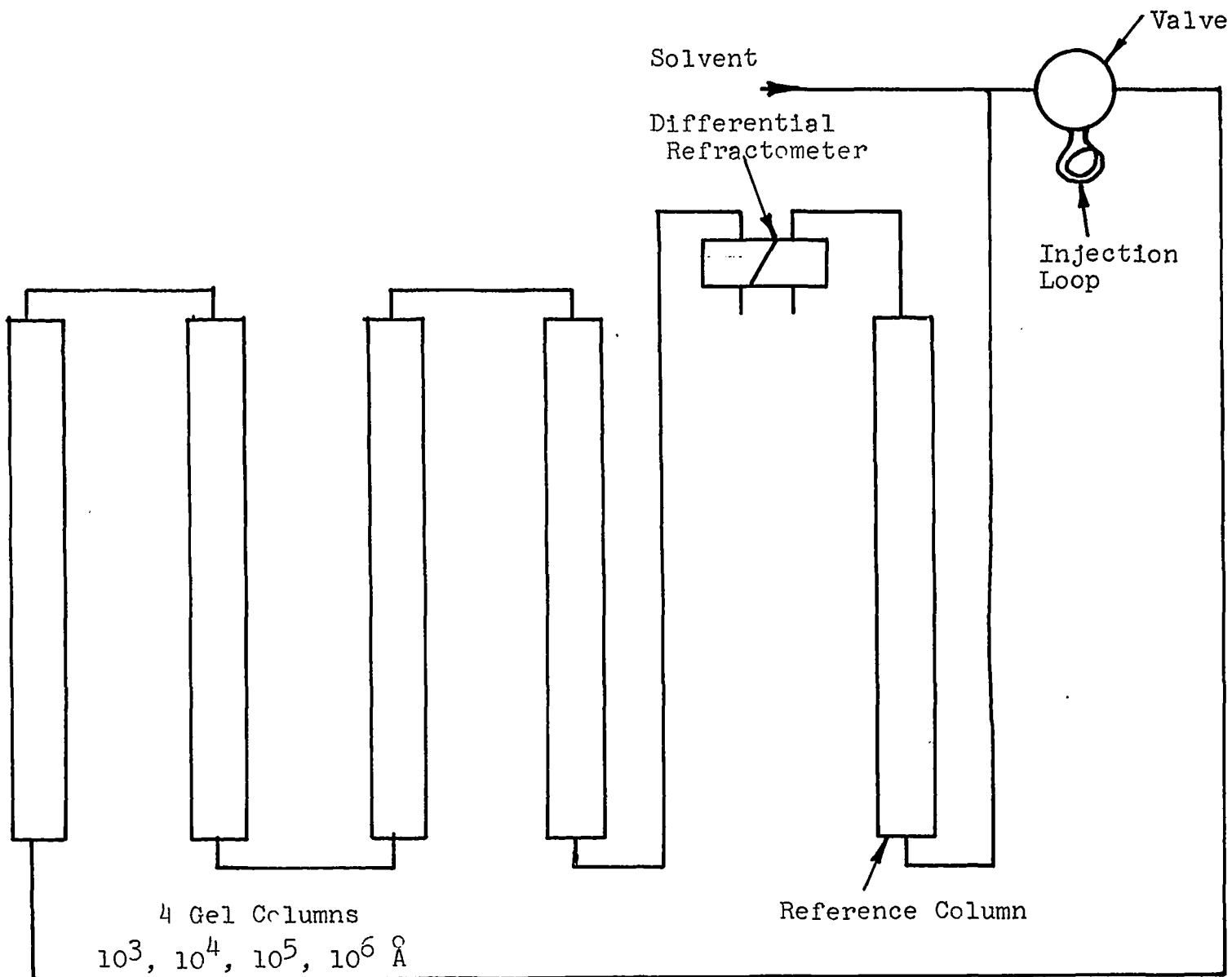
Figure 20 SIMPLIFIED SCHEMATIC DIAGRAM OF GPC APPARATUS
