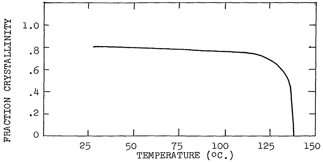
Figure 4 FRACTION CRYSTALLINITY OF POLYETHYLENE VS. TEMPERATURE (Ref. 17)
