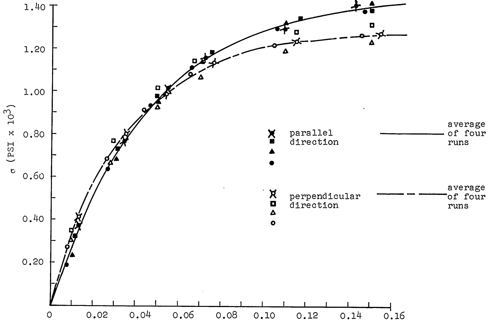
Figure 14 STRESS-STRAIN CURVES FOR UNCROSSLINKED GULF 5555 1.5 MIL POLYETHYLENE FILM AT AMBIENT TEMPERATURE
