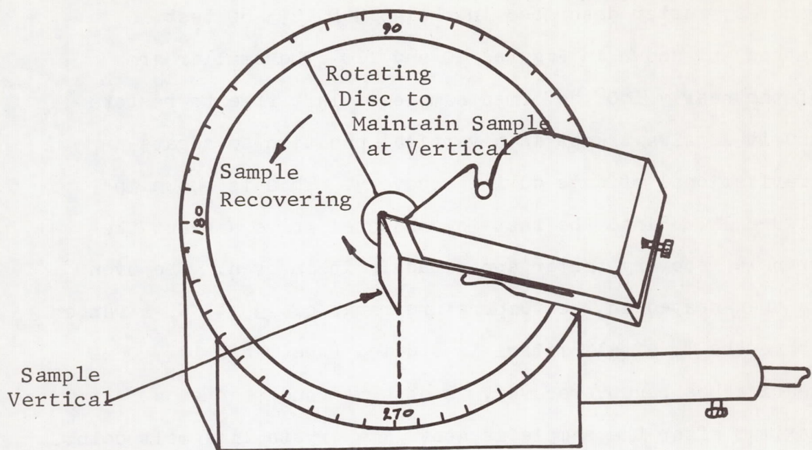
Figure 10. WRINKLE RECOVERY, "MEMORY", TESTING APPARATUS-SCHEMATIC
