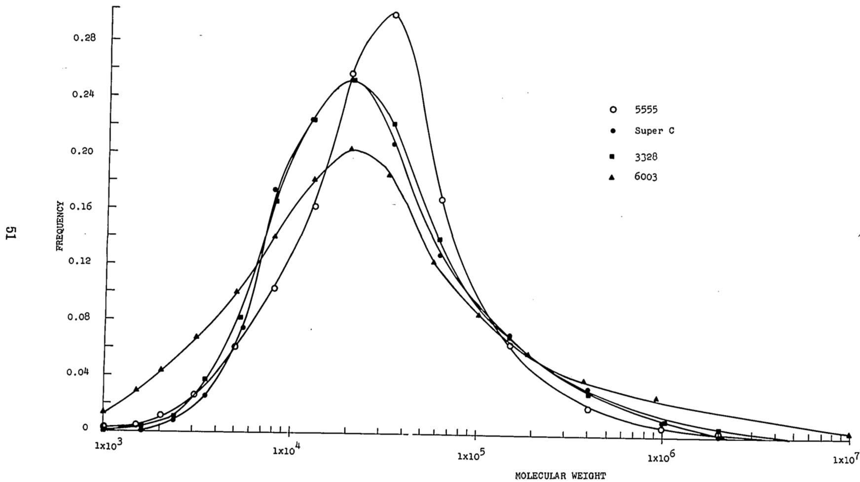
Figure 13 LOG MOLECULAR WEIGHT DISTRIBUTIONS OF THE POLYETHYLENES UNDER STUDY
