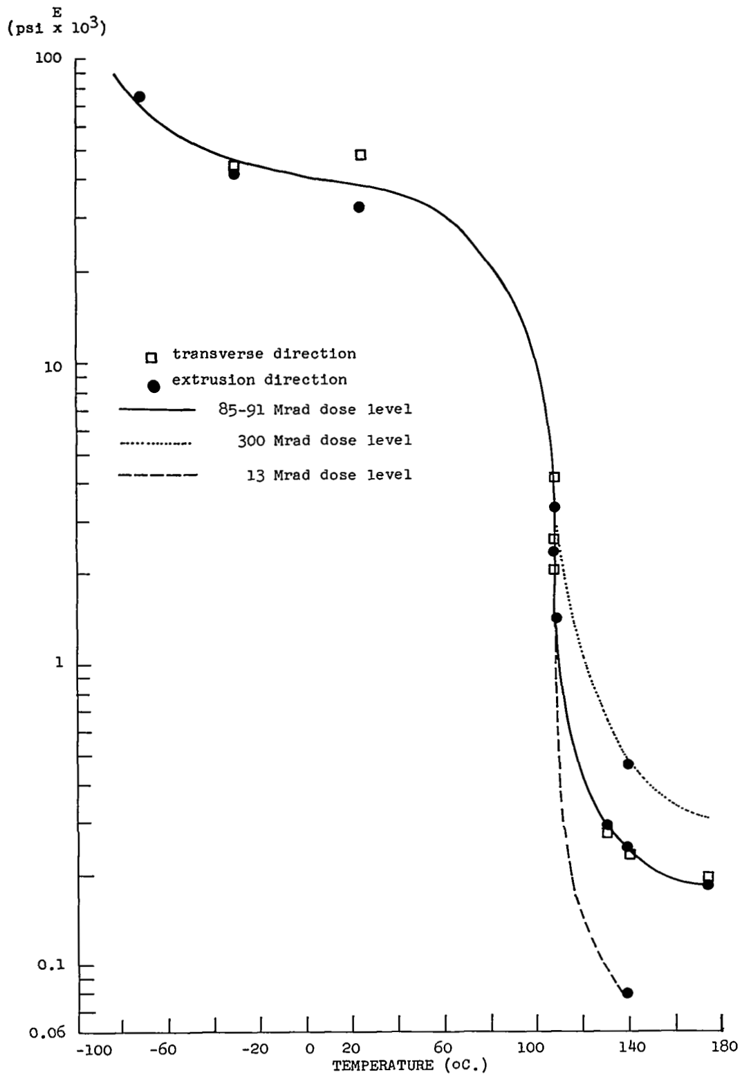
Figure 17 MODULUS OF ELASTICITY VS. TEMPERATURE FOR 1.5 MIL GULF 5555 POLYETHYLENE FILM
