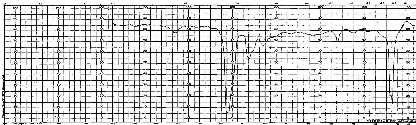
Figure 32 INFRARED SPECTRA-TIME STUDY OF ANNEALED STATE III, CROSSLINKED, GULF 5555 1.5 MIL POLYETHYLENE FILM - 101 HR. AND 389 HR.
