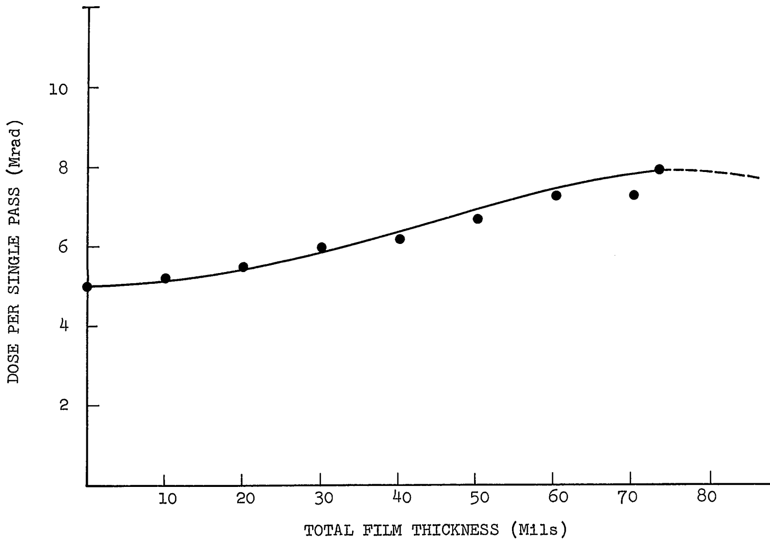
Figure 6 EXPERIMENTAL DOSE-DEPTH RELATIONSHIP FOR 1.5 MeV ELECTRONS PASSING THROUGH POLYETHYLENE
