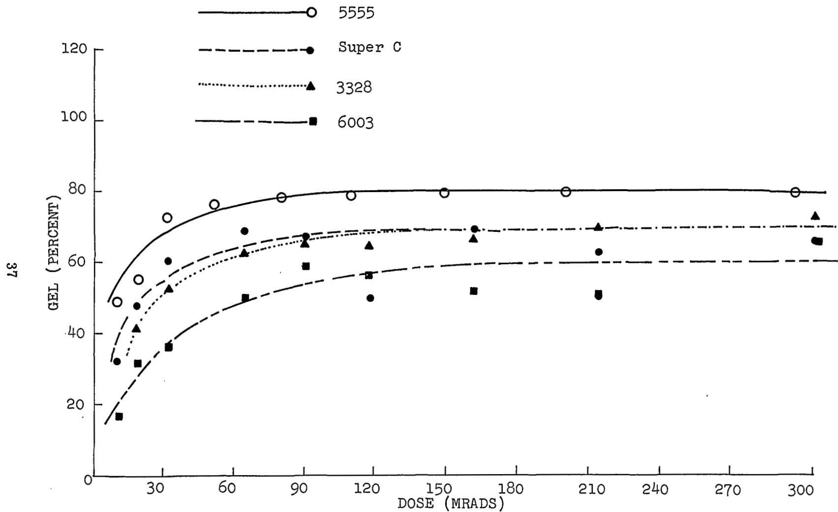
Figure 7 GEL FRACTIONS VS. DOSE FOR CROSSLINKED POLYETHYLENES UNDER STUDY
