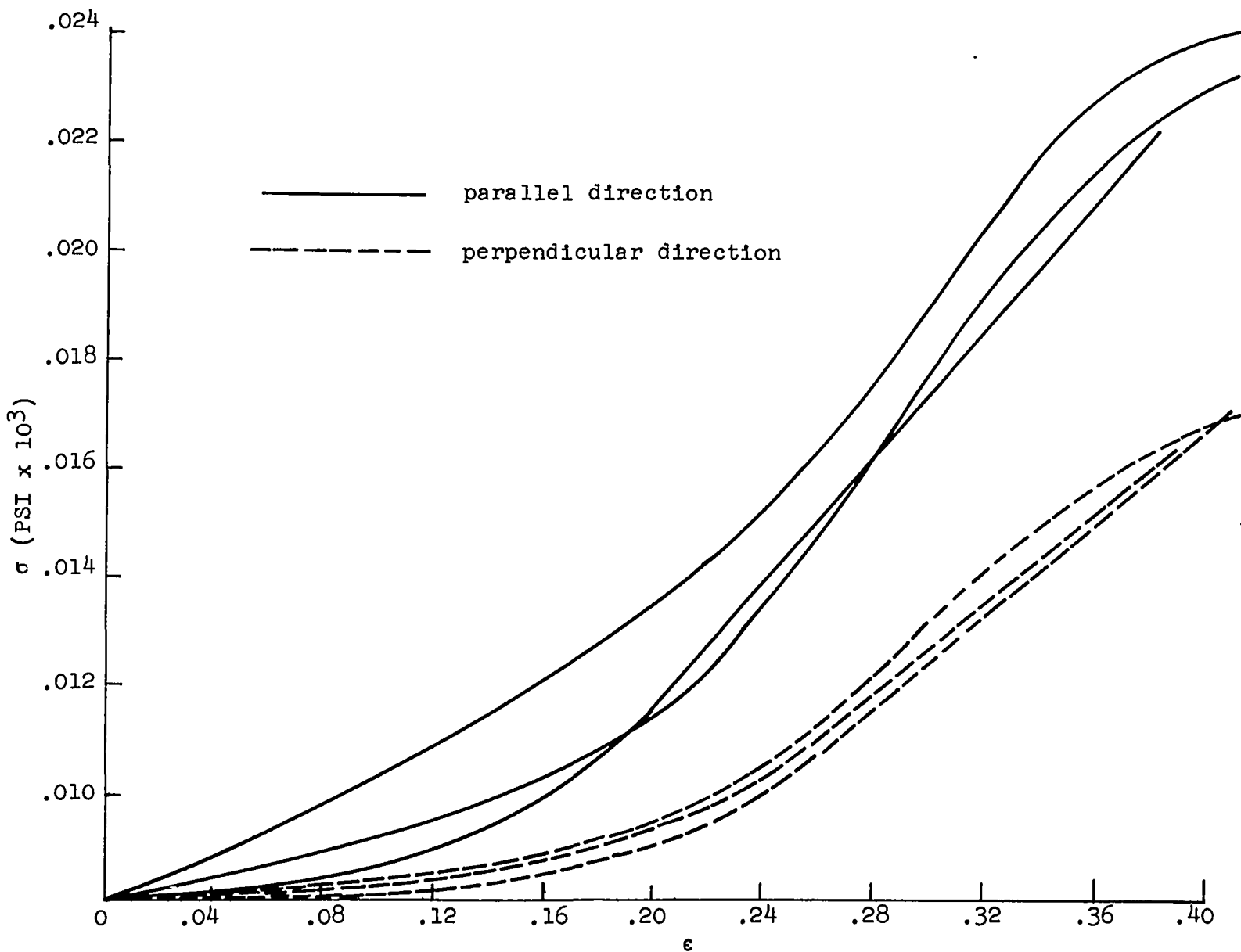
Figure 15 STRESS-STRAIN CURVES FOR CROSSLINKED GULF 5555 1.5 MIL POLYETHYLENE FILM AT 140°C.
