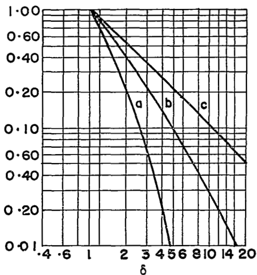
Fig. 2 DECREASE IN SOLUBLE FRACTION OF CROSSLINKED POLYMER WHEN \delta EXCEEDS 1. (Reference 1)
