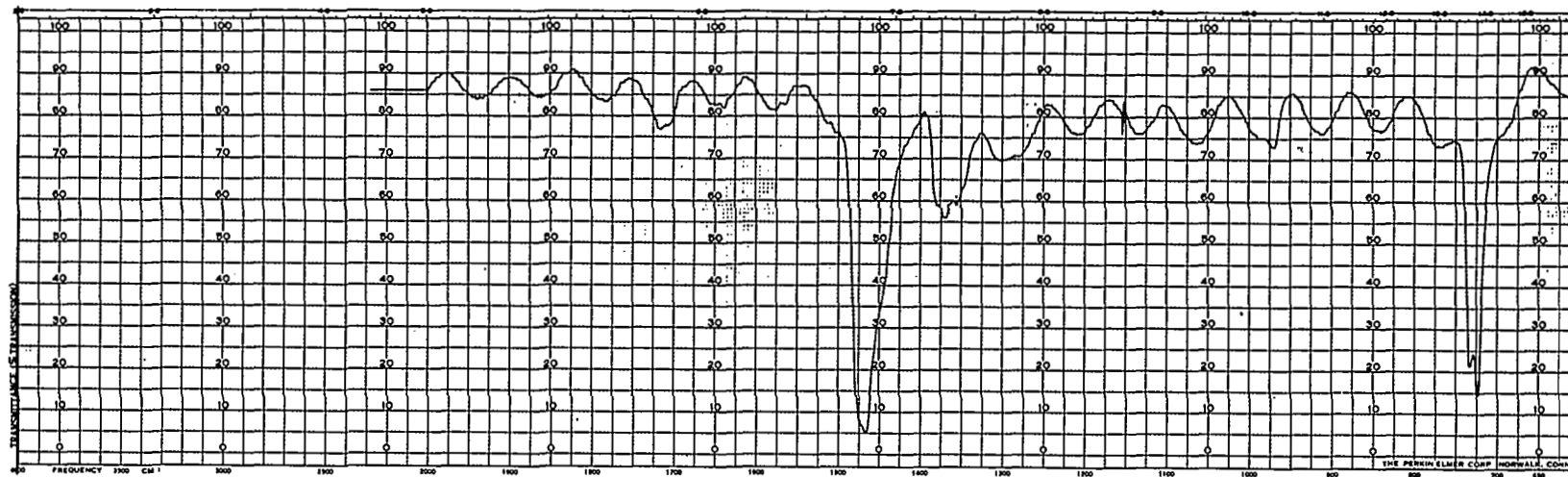
Figure 31 INFRARED SPECTRA-TIME STUDY OF ANNEALED STATE III, CROSSLINKED, GULF 5555 1.5 MIL POLYETHYLENE FILM - 1.87 HR. AND 24.62 HR.
