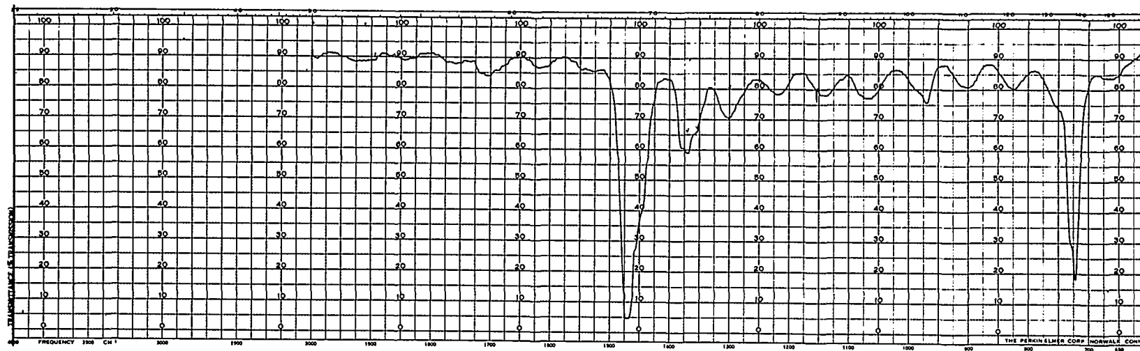
Figure 29 INFRARED SPECTRA-TIME STUDY OF ANNEALED STATE III, CROSSLINKED, GULF 5555 1.5 MIL POLYETHYLENE FILM - 0.14 HR. AND 0.31 HR.
