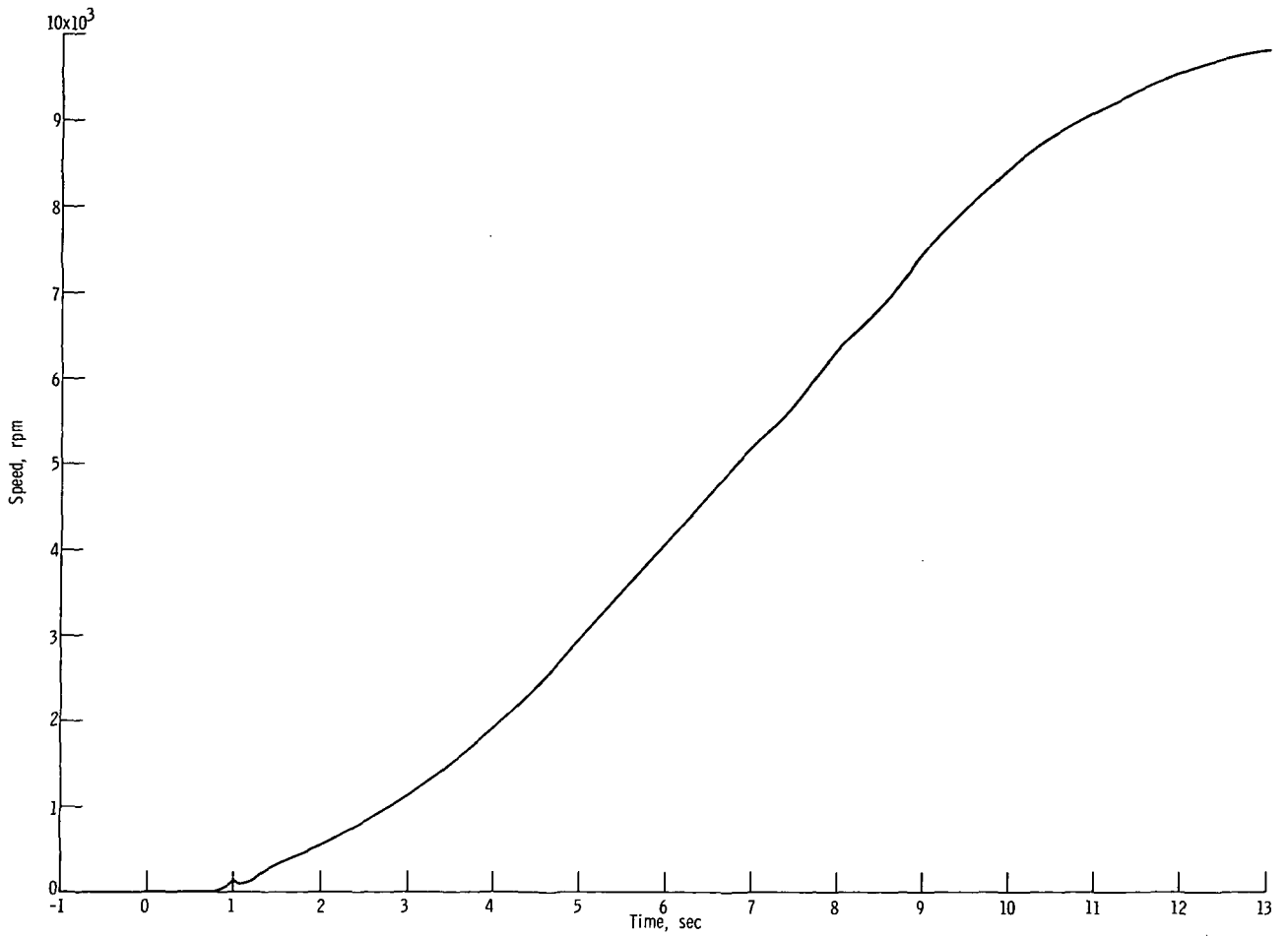
Figure 14. - Speed against time for wet axial pump test. Nominal tank pressure, 35 psia (24.1 N/cm 2 ).
