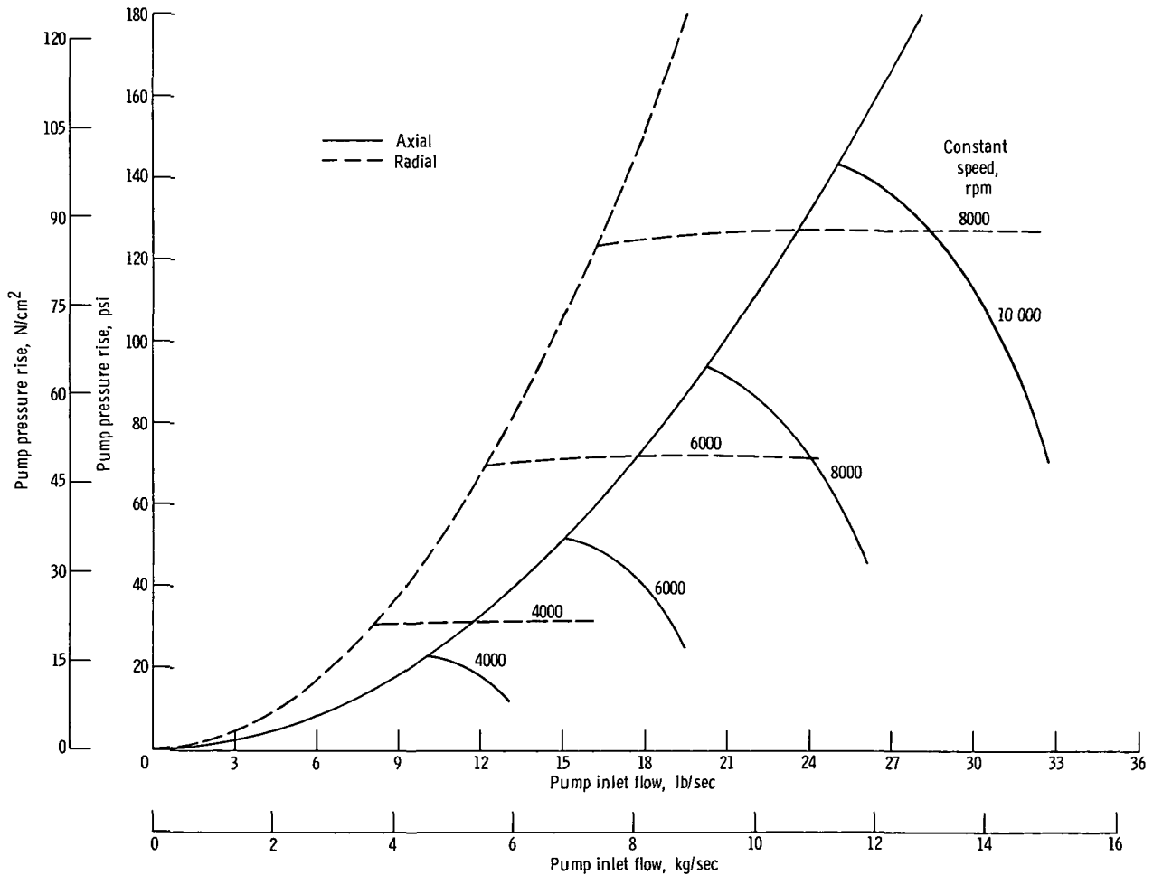
Figure 20. - Axial and radial characteristics of pump used in bootstrap tests.
