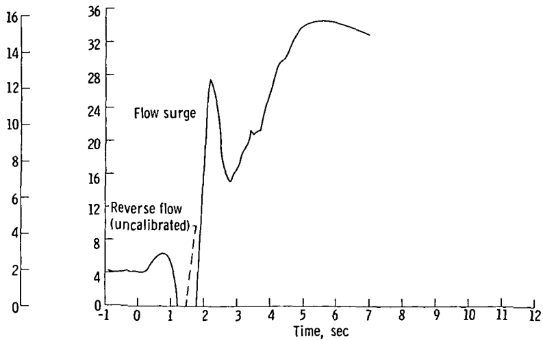
Figure 8. - Pump inlet flow against time after opening of turbine power control valve (TPCV) for four bootstrap tests.
