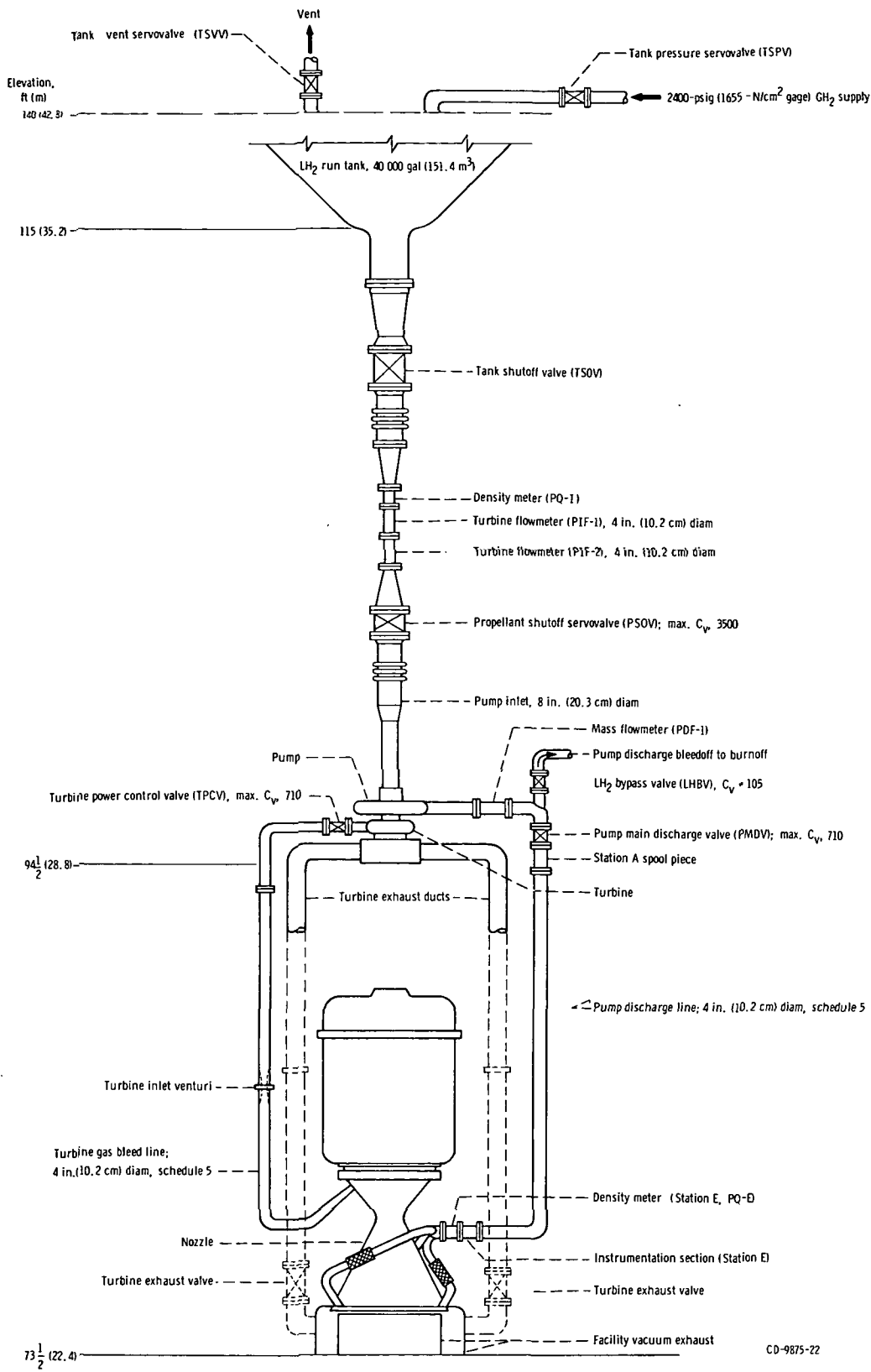
Figure 1. - Full-scale nuclear rocket cold-flow experiment in B-3 facility.
