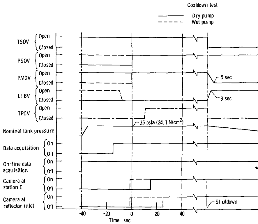
Figure 4. - Time history of events produced by an automatic test sequencer. TPCV open for bootstrap tests only.
