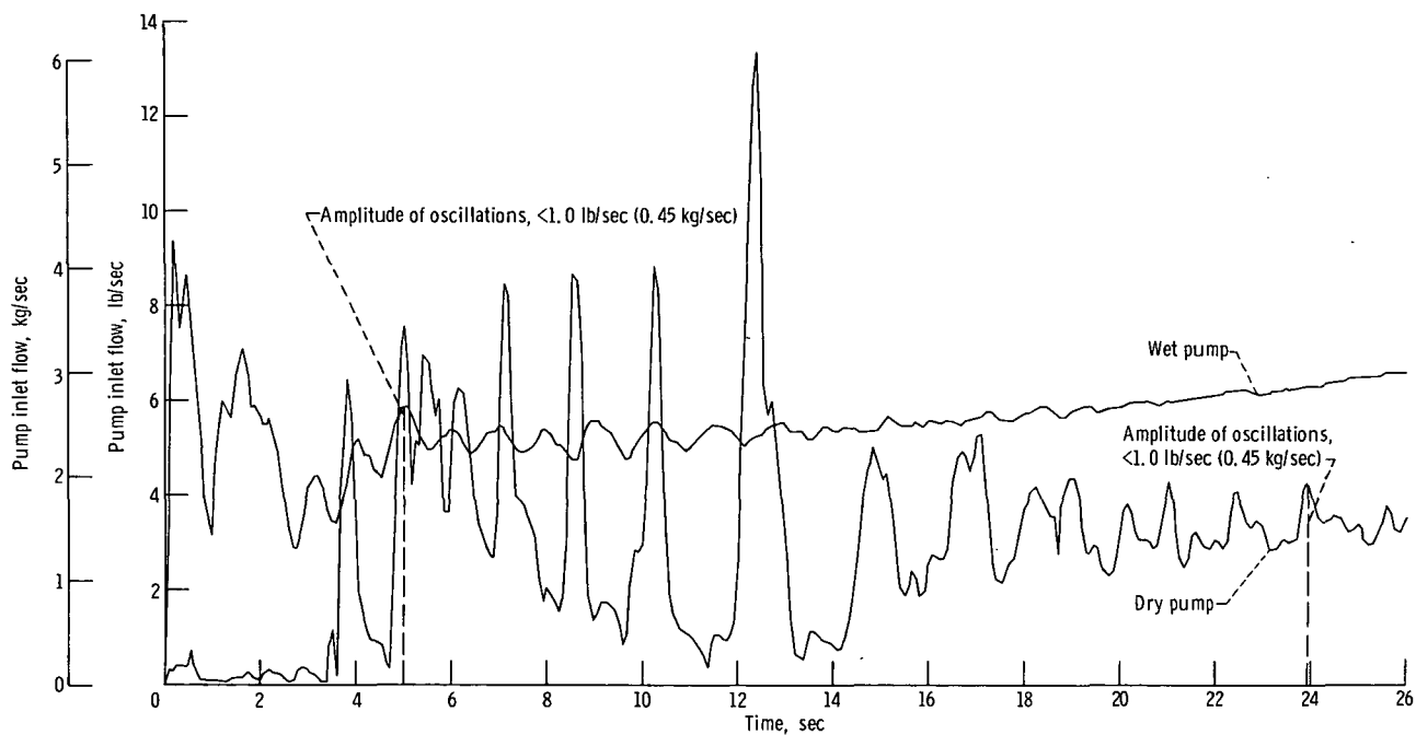
Figure 5. - Pump inlet flow against time for wet and dry pump cooldown tests. Nominal tank pressure, 35 psia (24.1 N/cm 2 ).
