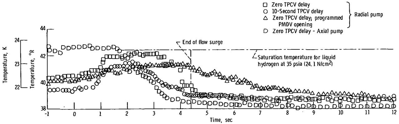
Figure 19. - Pump inlet temperature against time for wet pump bootstrap tests with 35-psia (24.1-N/cm 2 ) nominal tank pressure.
