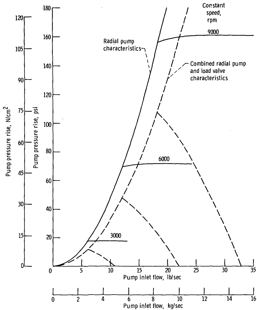
Figure 21. - Pump pressure rise against pump inlet flow for radial pump.
