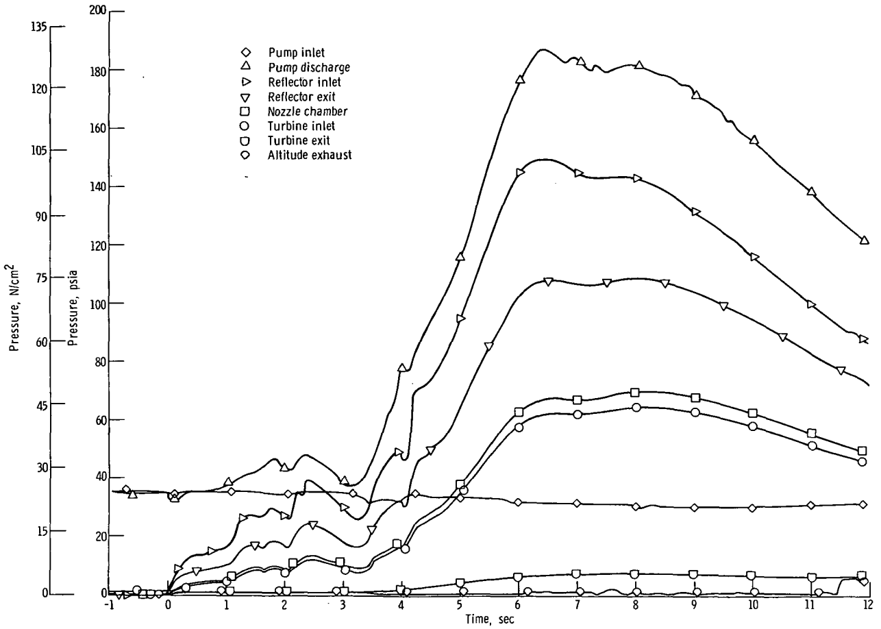
Figure 11. - Pressure profile for wet pump bootstrap test. Nominal tank pressure, 35 psia (24.1 \text{N/cm}^2 ).
