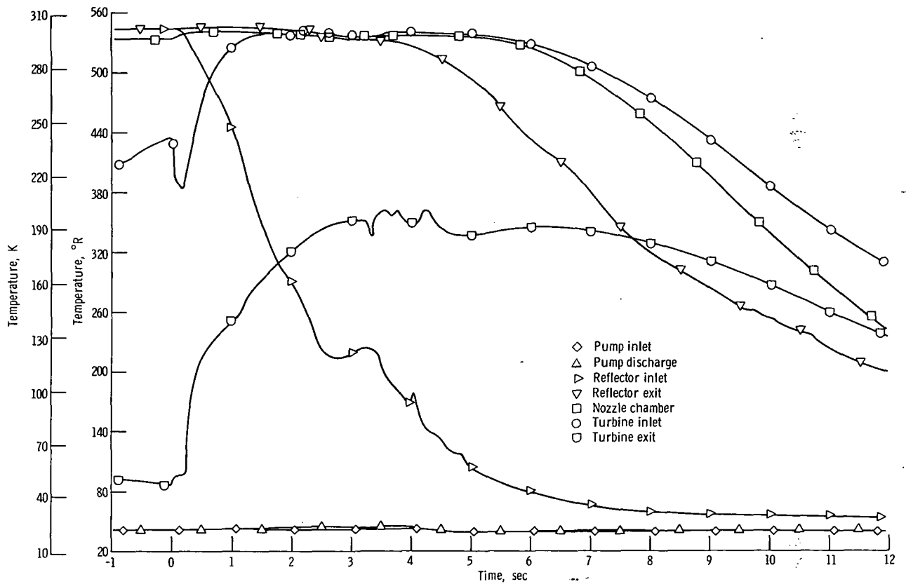
Figure 10. - Temperature profile for wet pump bootstrap test. Nominal tank pressure, 35 psia (24.1 N/cm 2 ).
