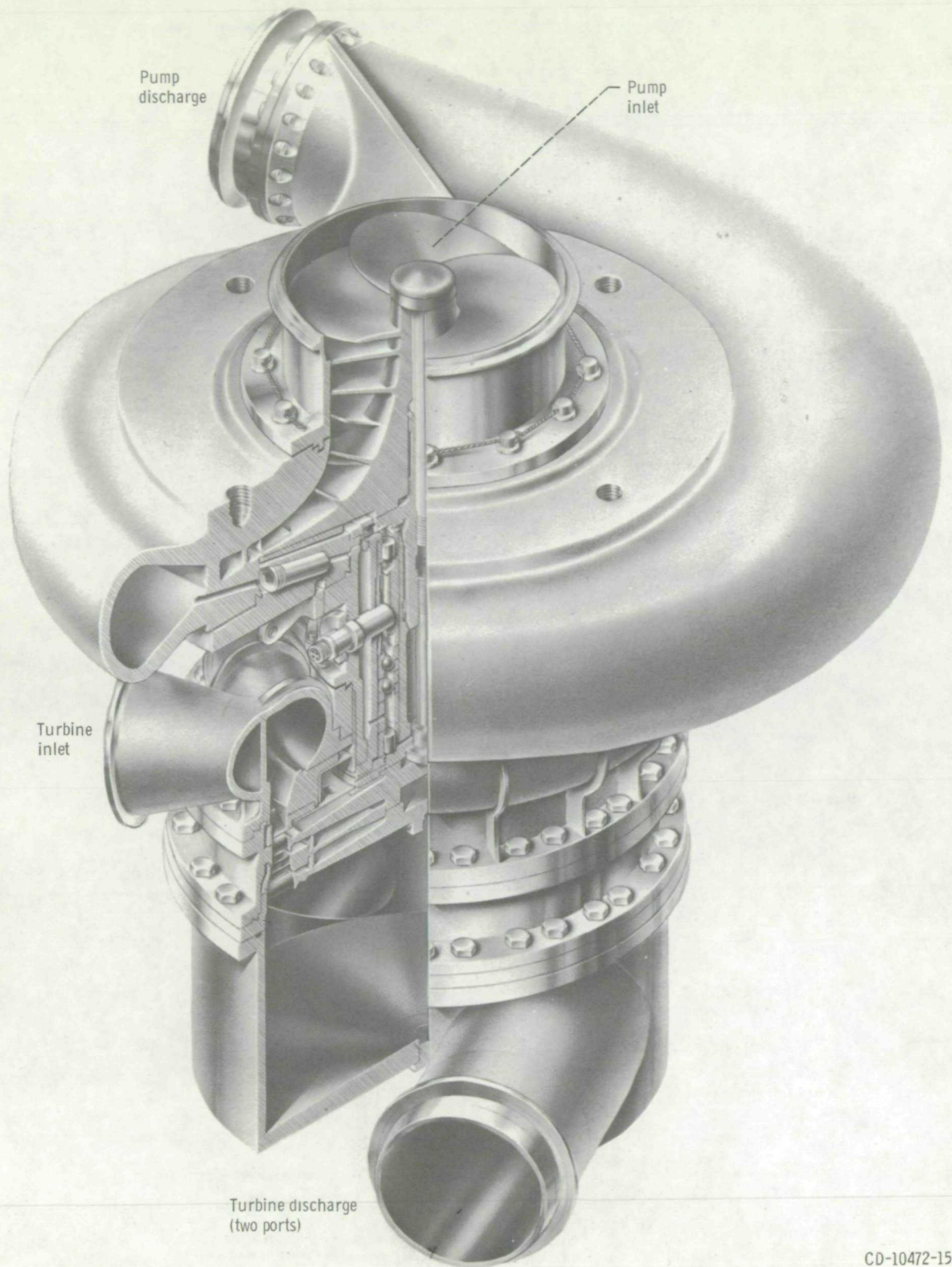
Figure 2. - Mark III, Model 4 turbopump.
