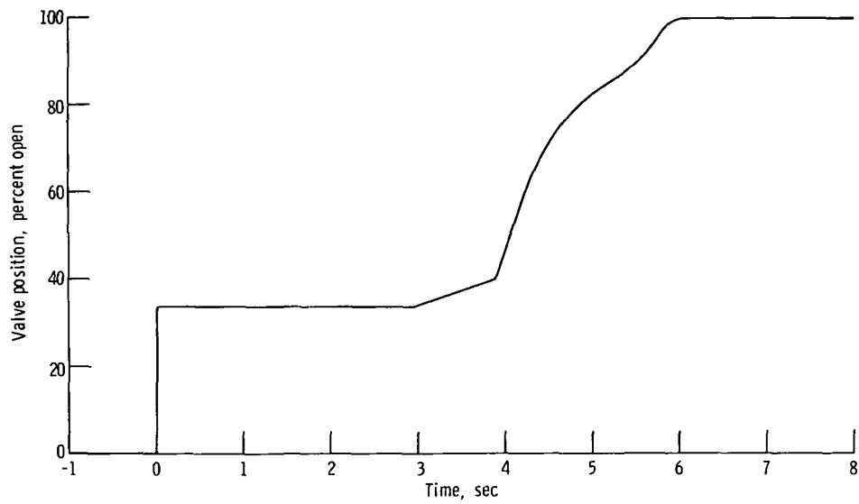
Figure 17. - Programmed opening of pump main discharge valve (PMDV) for wet pump bootstrap test. Nominal tank pressure, 35 psia (24.1 N/cm 2 ).
