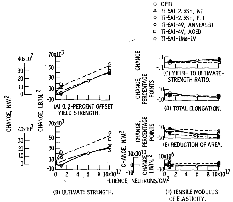
Figure 10. - Effect of reactor irradiation at 17 K on 17 K tensile properties of titanium and titanium-base alloys. Neutron energy > 0.5 MeV (80 fJ).
