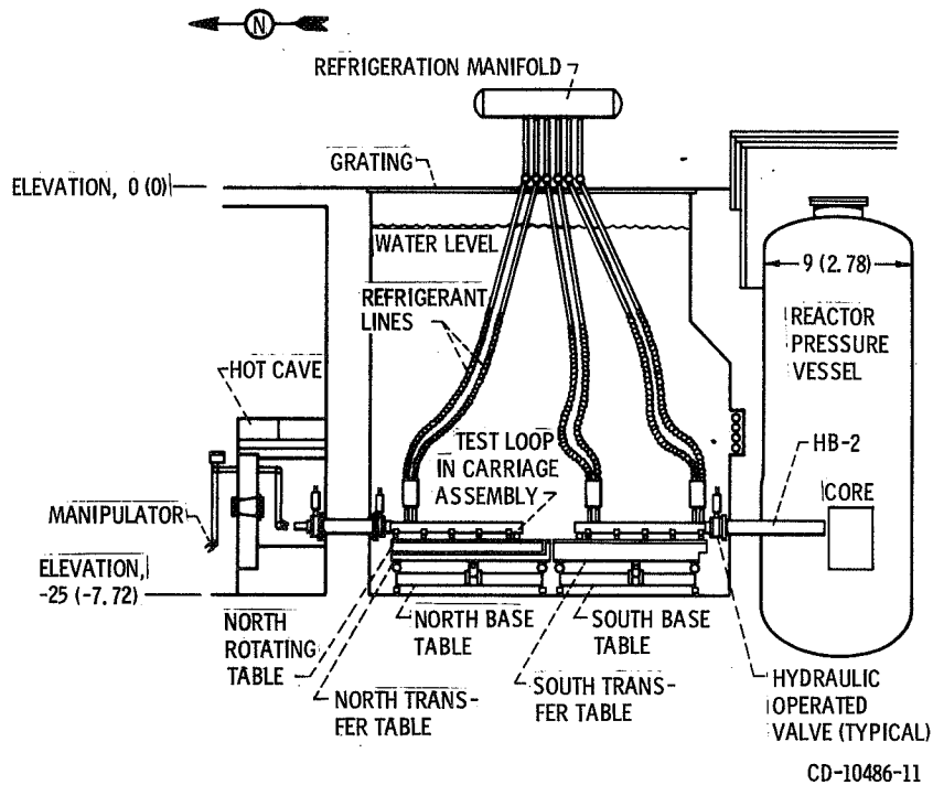
Figure 2. - Cryogenic irradiation test equipment. All dimensions are in feet (m).
